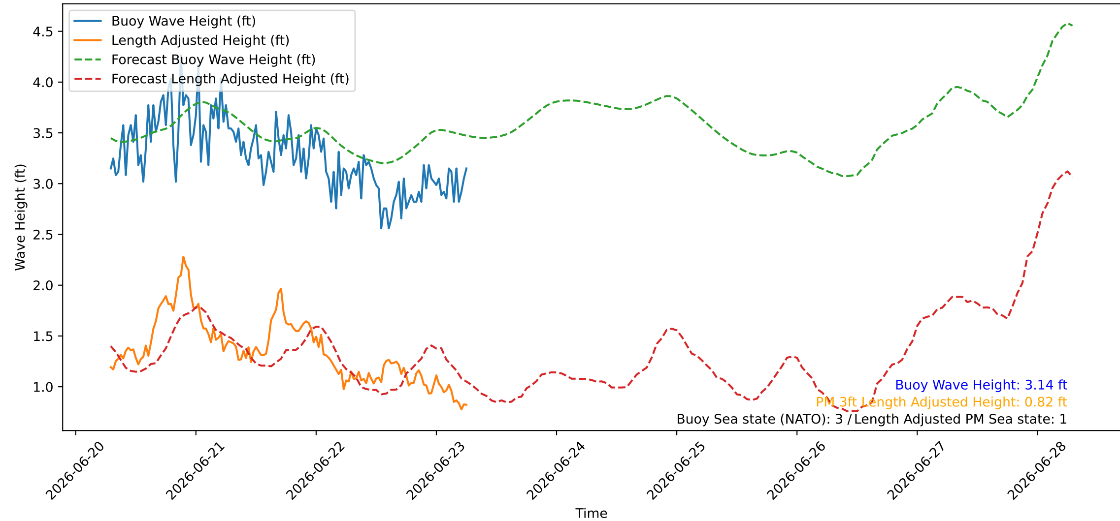
Wave Heights over Time for Oceanside Harbor at 2026-06-23 06:50:26
