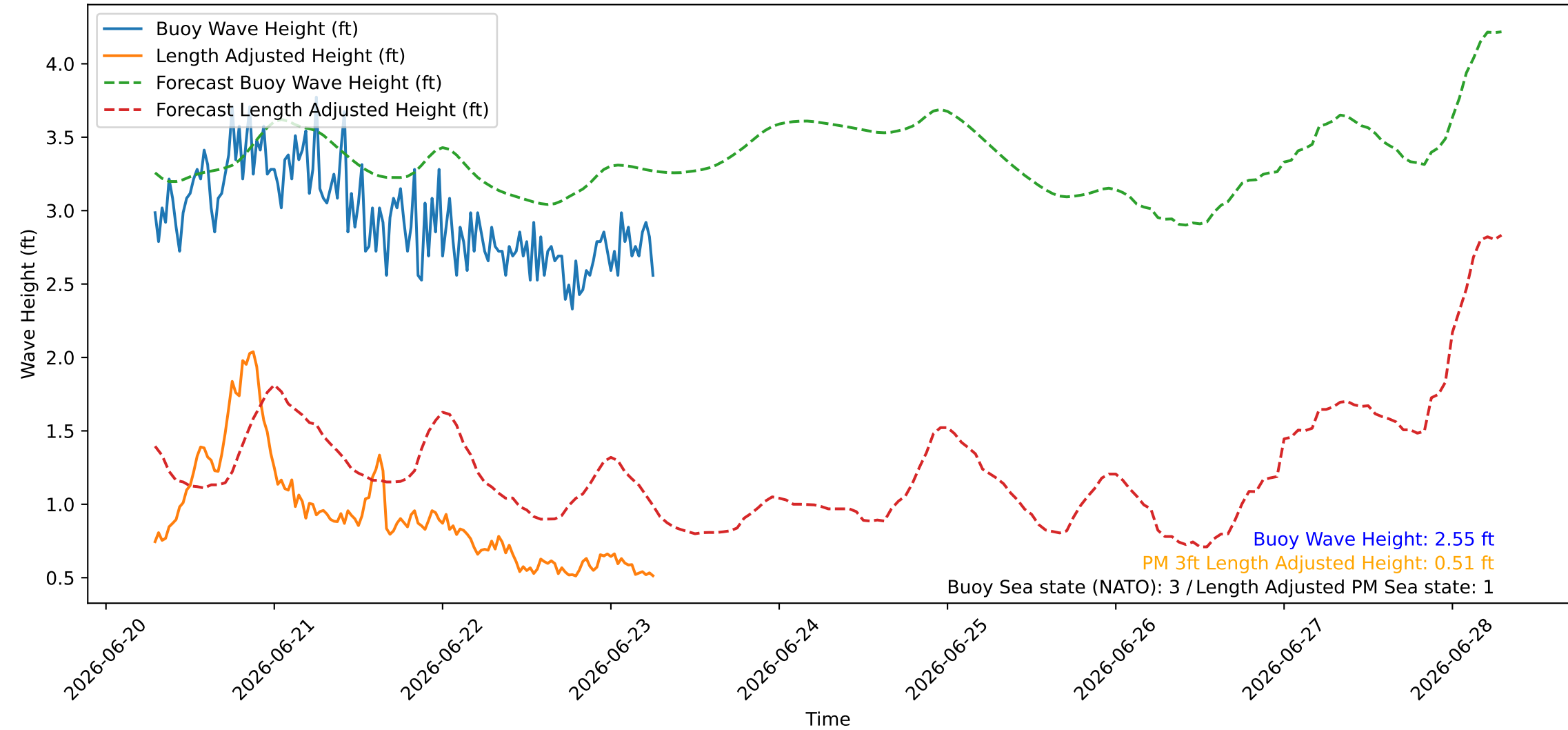
Wave Heights over Time for Red Beach at 2026-06-23 06:50:47
