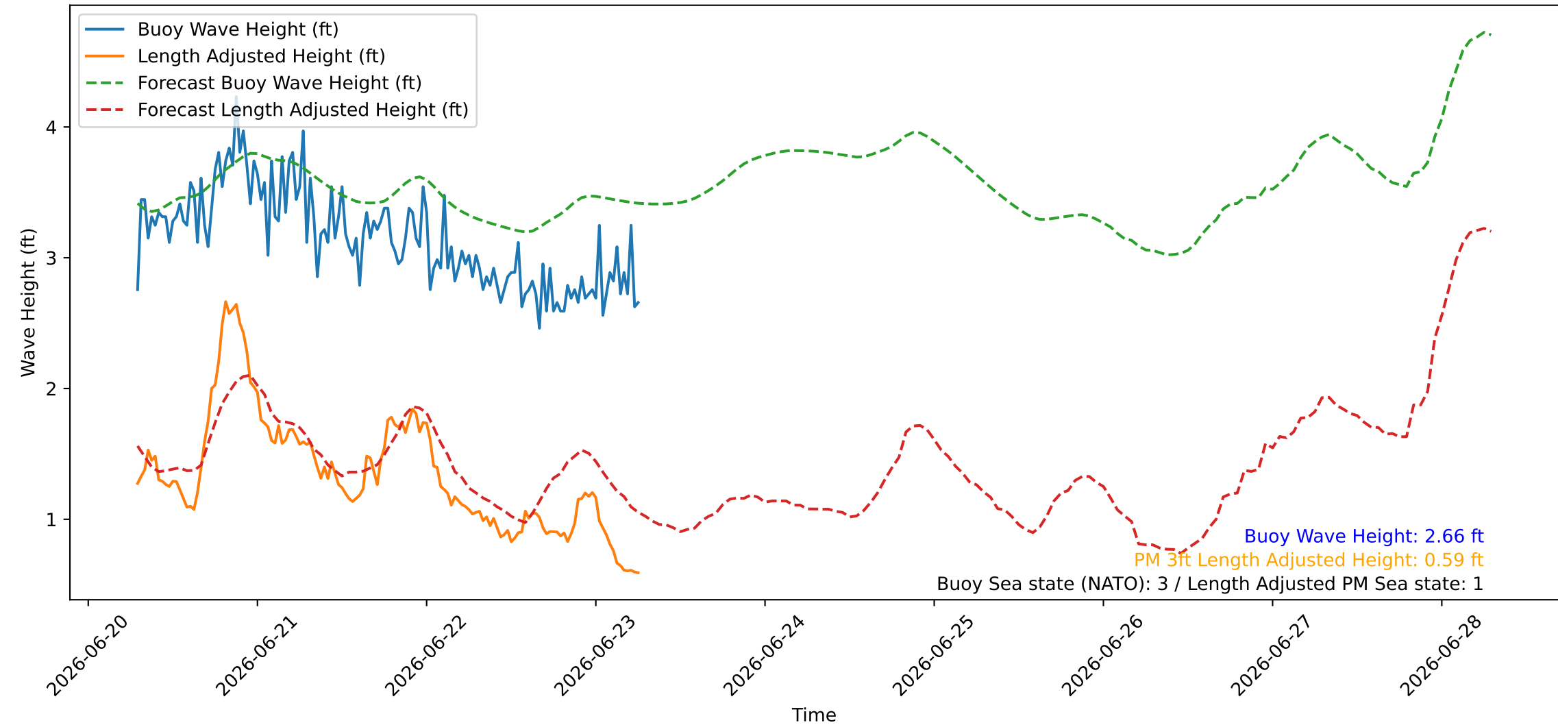
Wave Heights over Time for Green Beach at 2026-06-23 06:51:09
