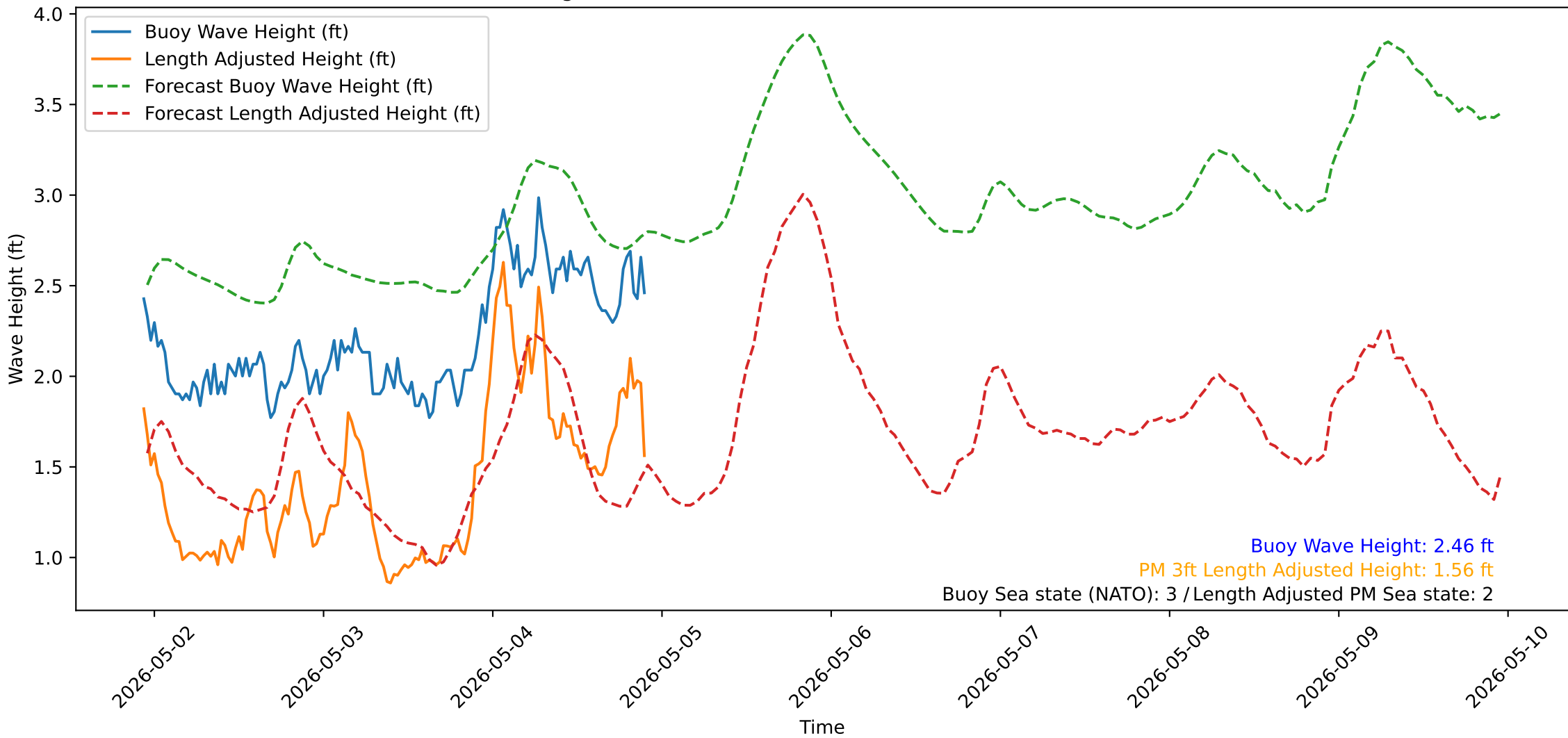
Wave Heights over Time for Green Beach at 2026-05-04 22:31:13
