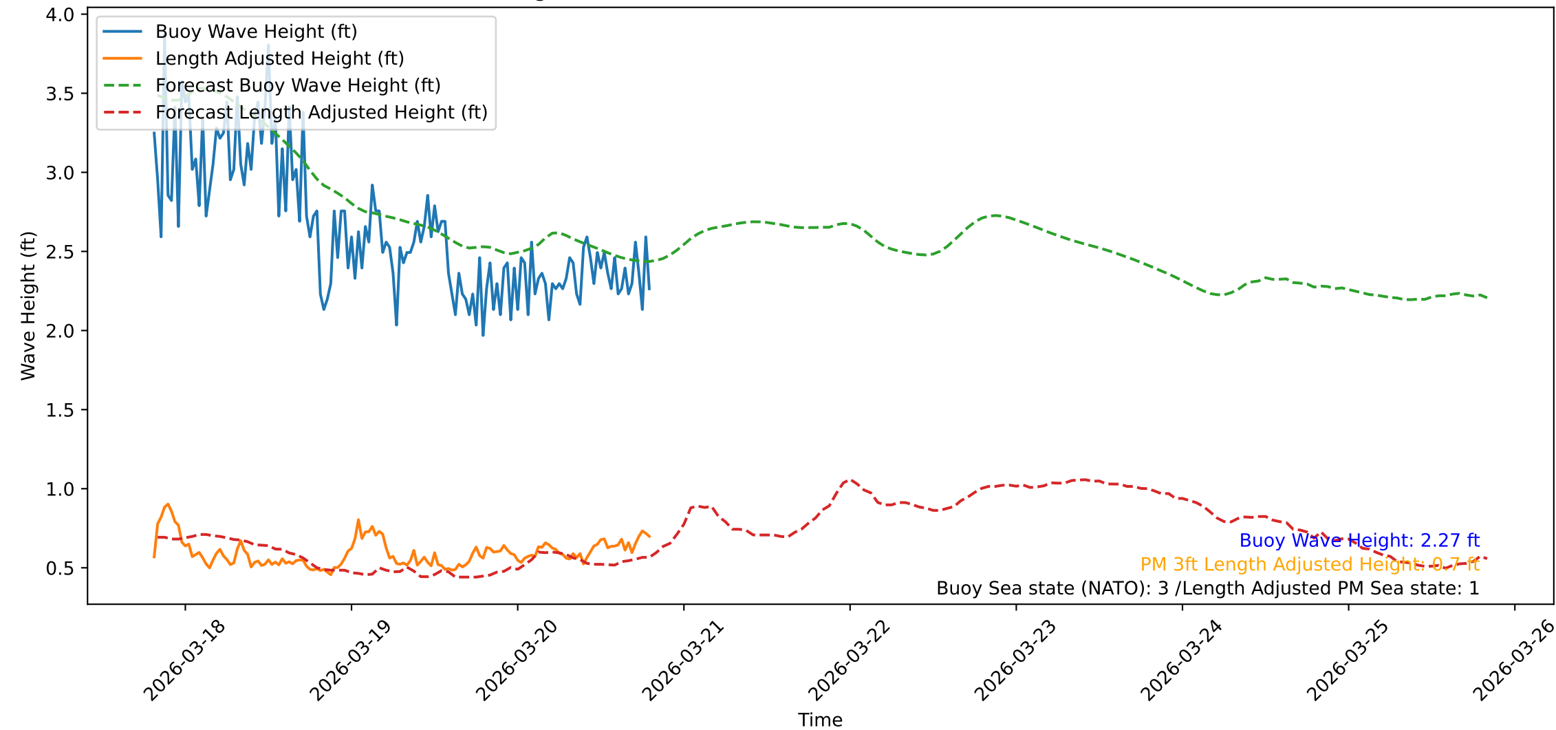
Wave Heights over Time for Oceanside Harbor at 2026-03-20 19:30:31
