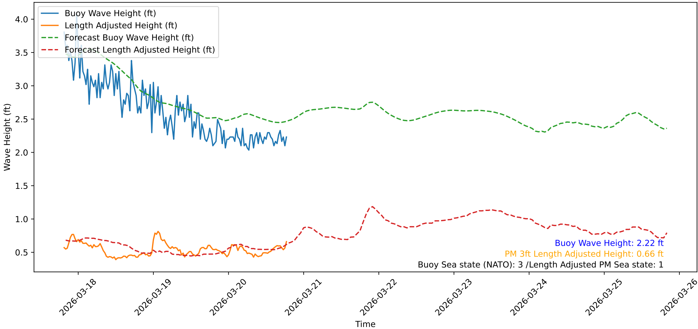
Wave Heights over Time for Green Beach at 2026-03-20 19:31:10
