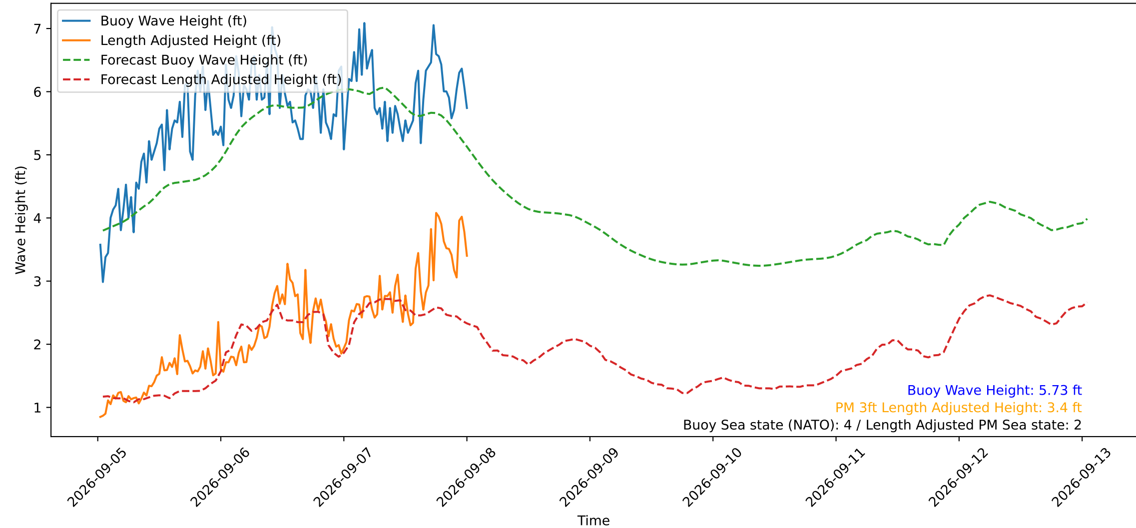
Wave Heights over Time for Oceanside Harbor at 2026-09-08 00:40:29
