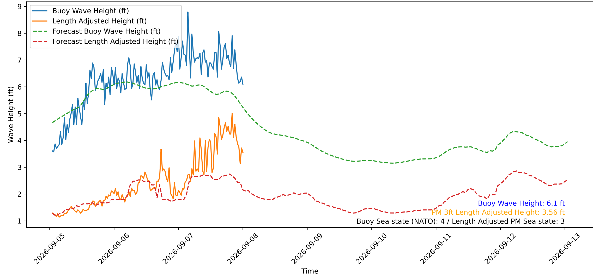
Wave Heights over Time for Green Beach at 2026-09-08 00:41:12
