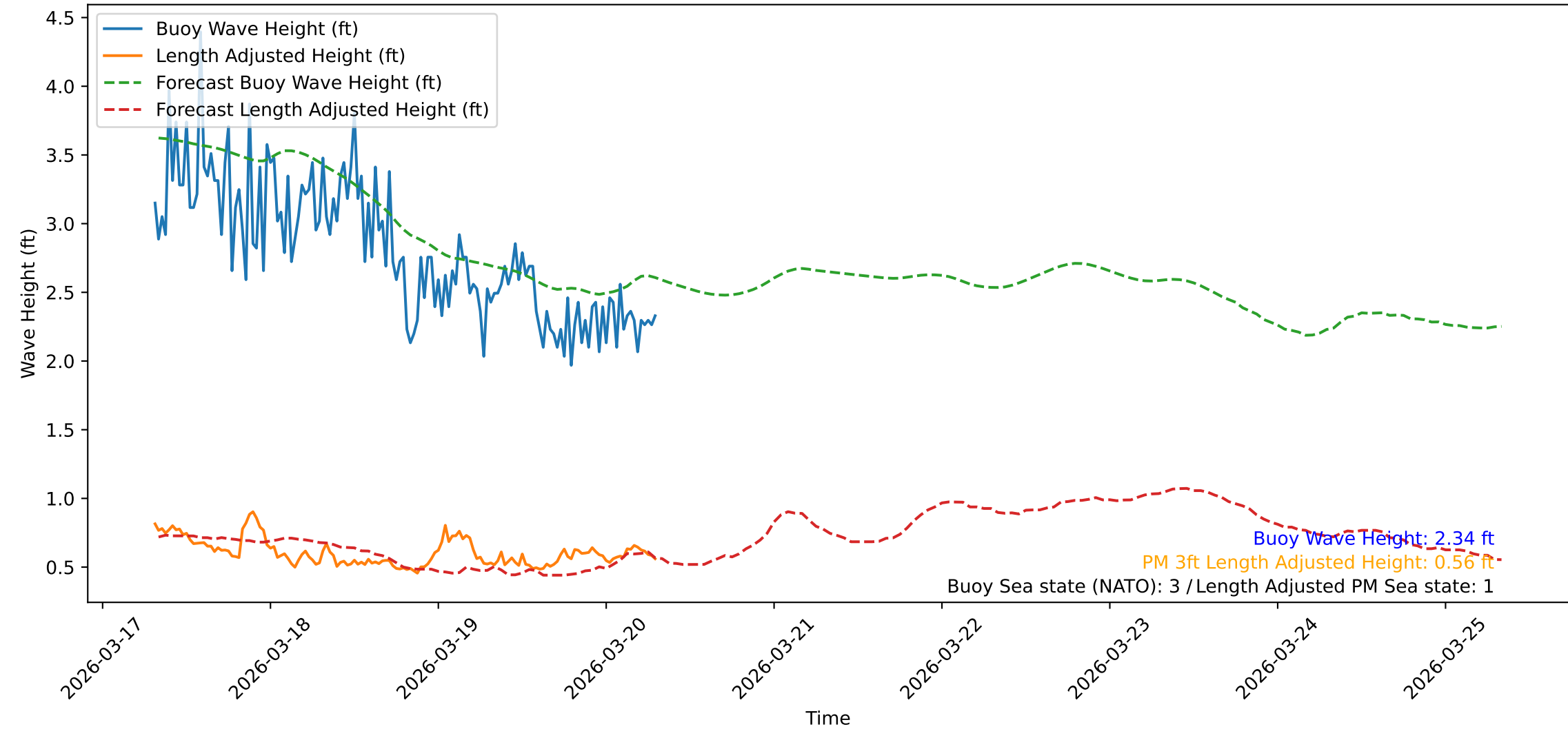
Wave Heights over Time for Oceanside Harbor at 2026-03-20 07:40:32
