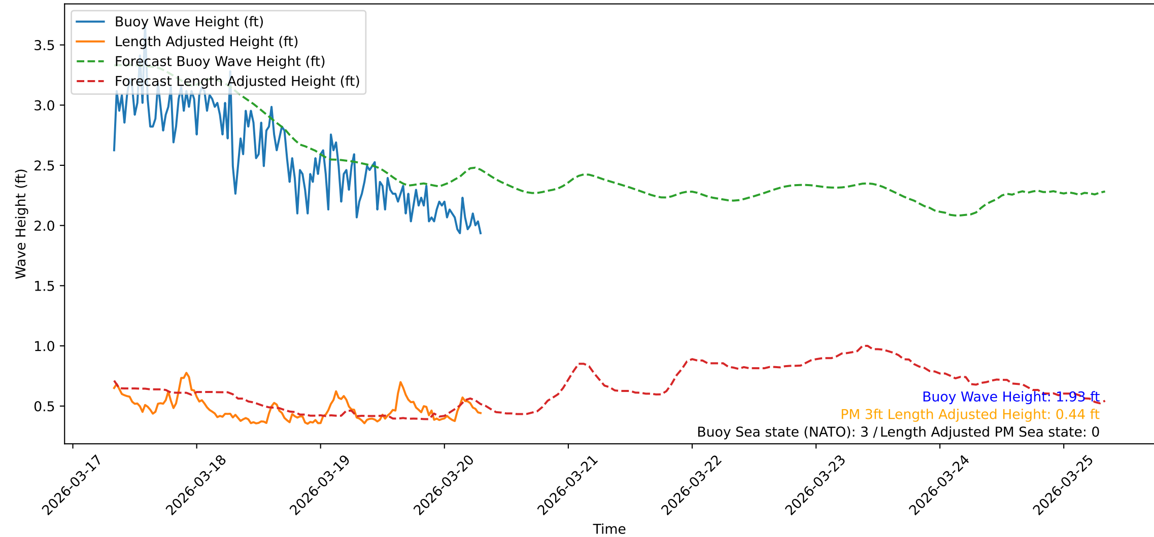
Wave Heights over Time for Red Beach at 2026-03-20 07:40:48
