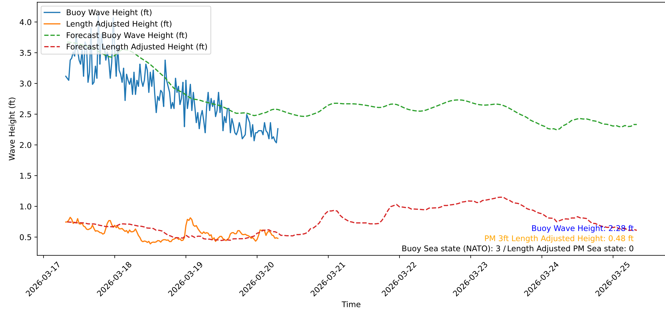
Wave Heights over Time for Green Beach at 2026-03-20 07:41:10
