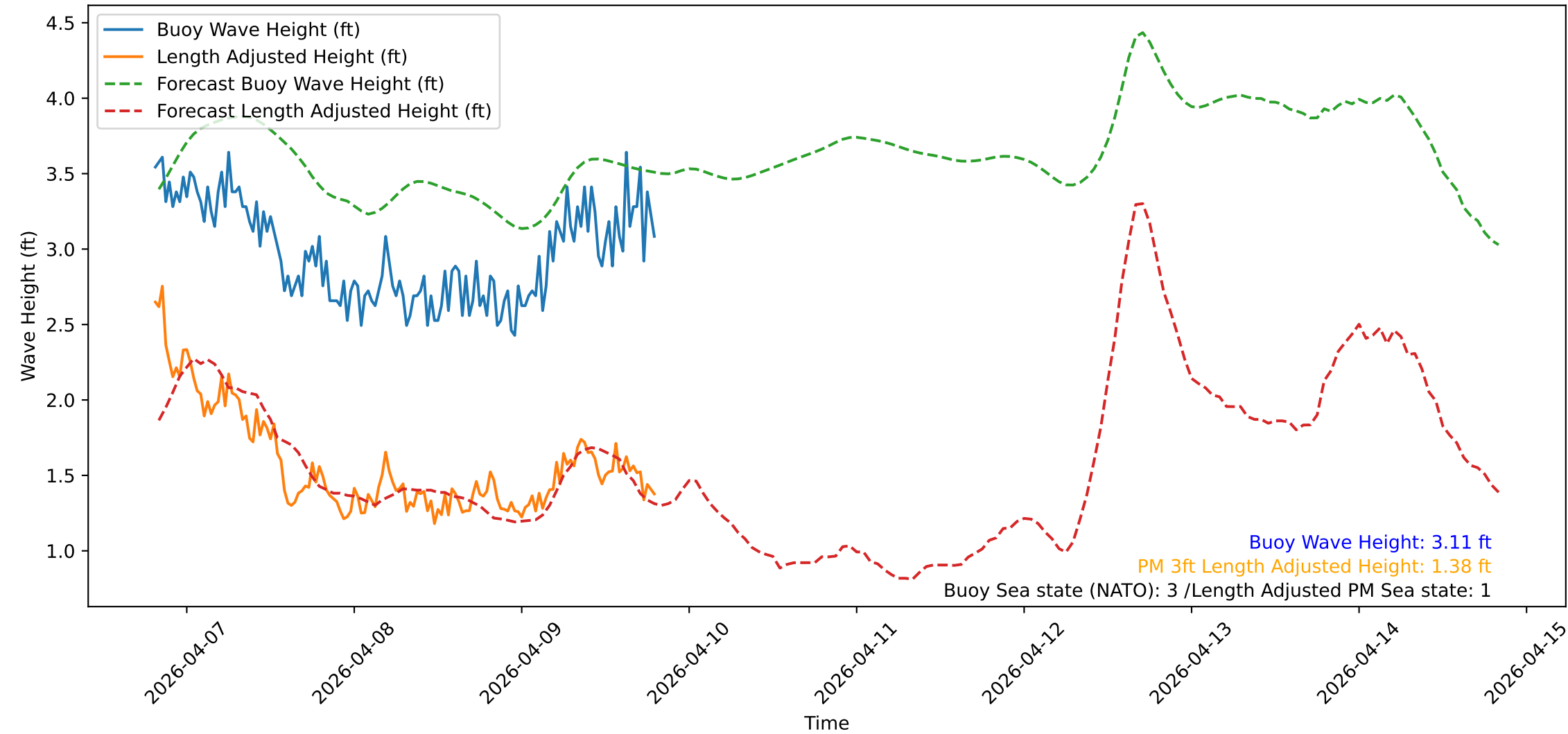
Wave Heights over Time for Oceanside Harbor at 2026-04-09 19:30:32
