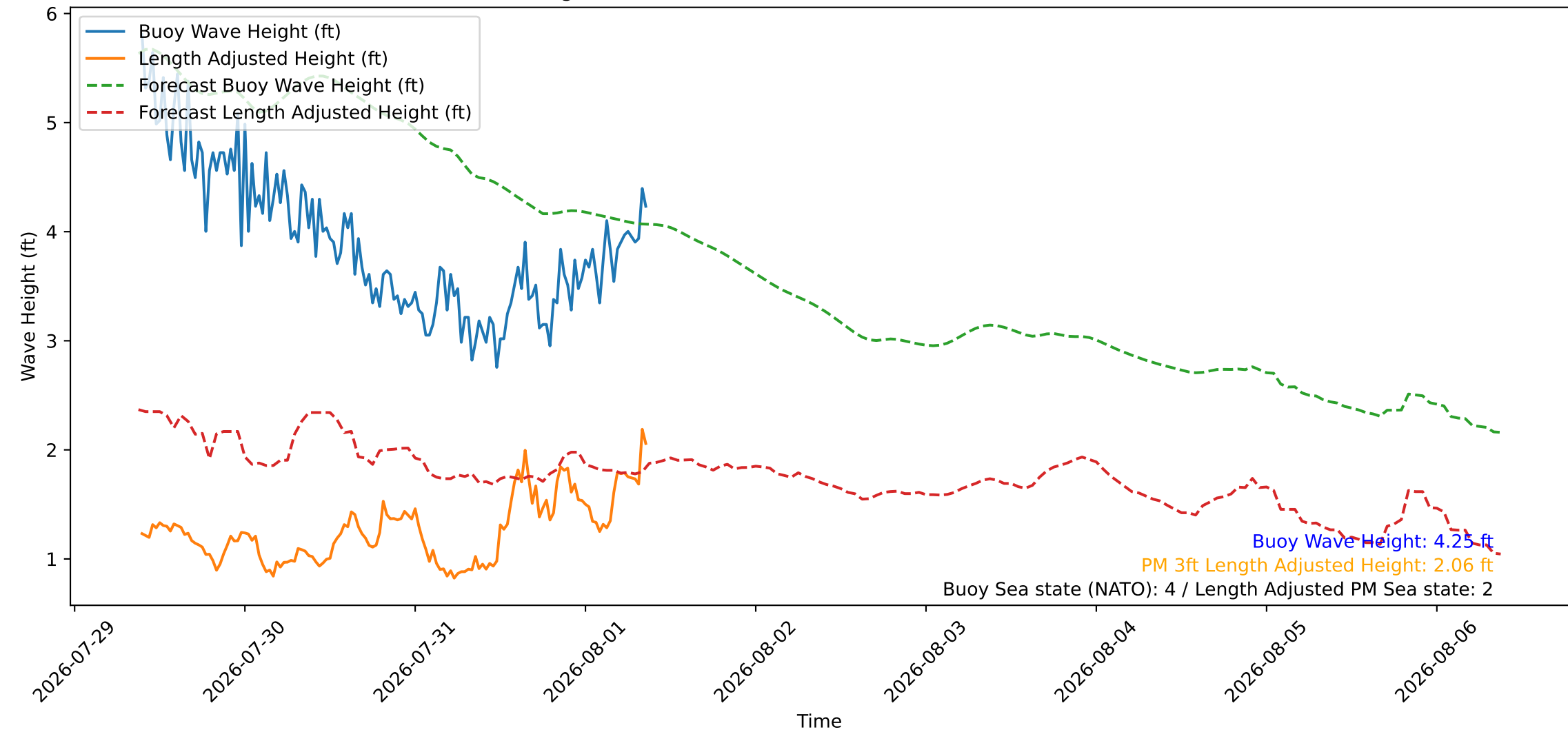
Wave Heights over Time for Green Beach at 2026-08-01 09:21:12
