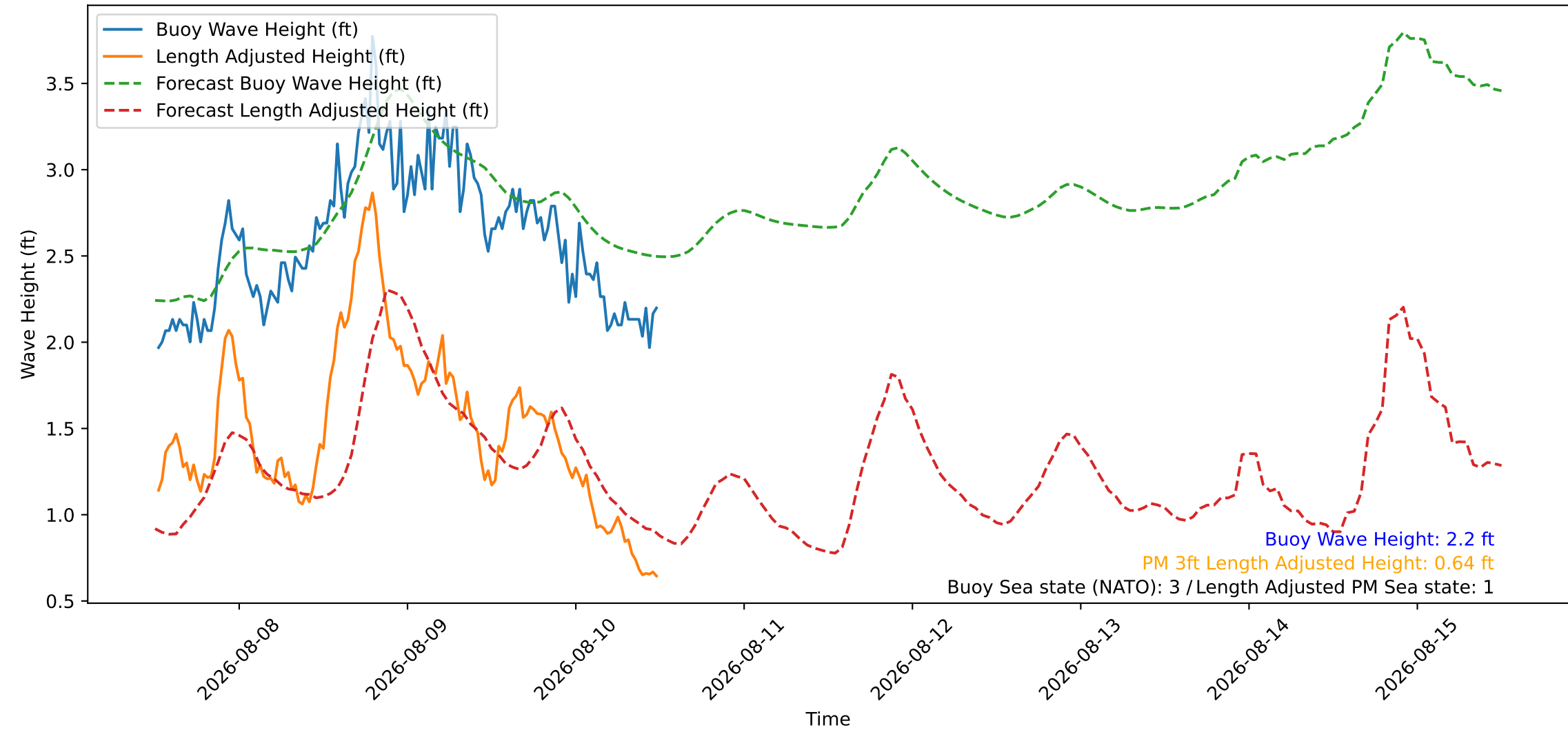
Wave Heights over Time for Green Beach at 2026-08-10 12:21:10
