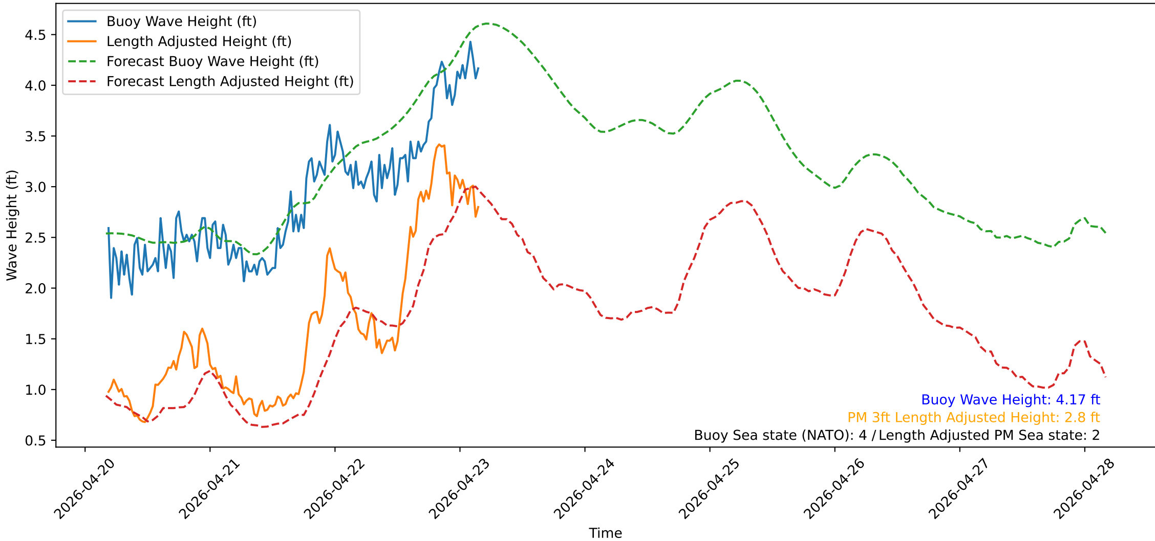
Wave Heights over Time for Oceanside Harbor at 2026-04-23 04:20:31
