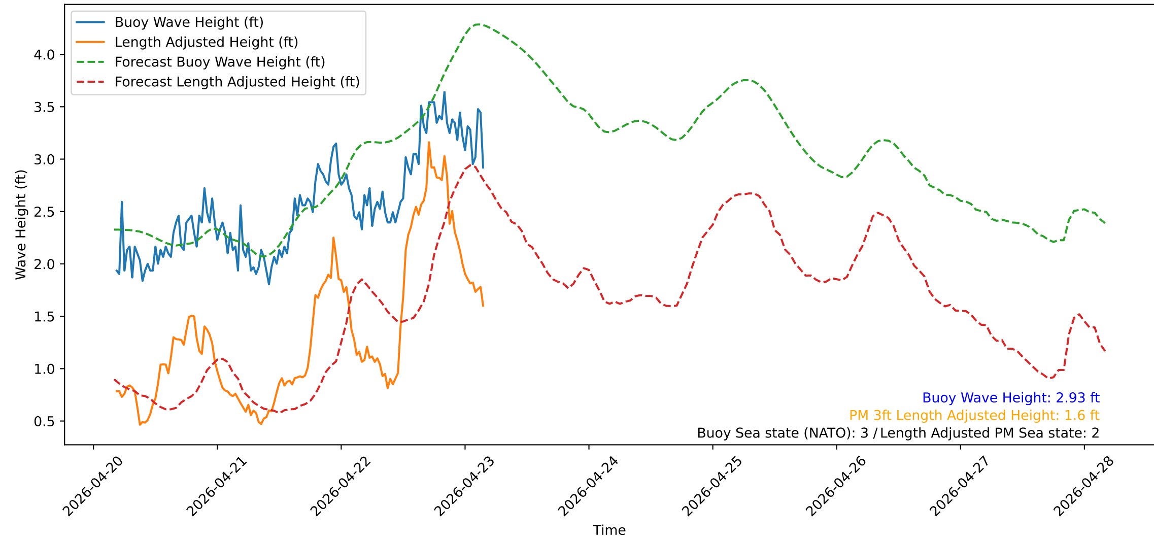
Wave Heights over Time for Red Beach at 2026-04-23 04:20:51
