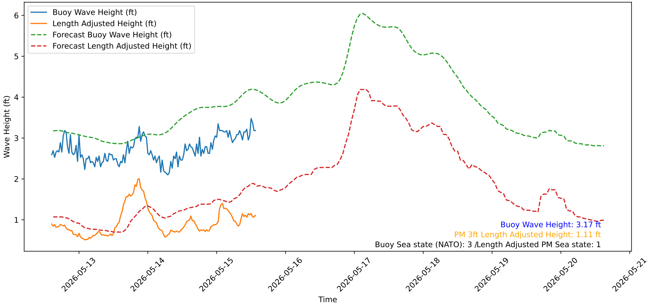
Wave Heights over Time for Green Beach at 2026-05-15 14:31:14
