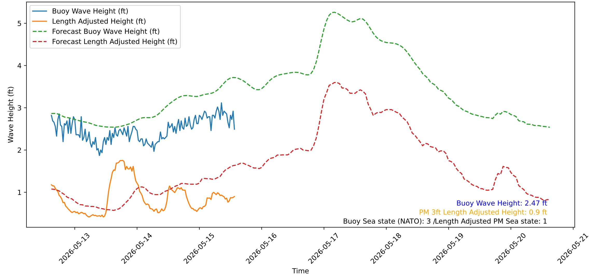
Wave Heights over Time for Red Beach at 2026-05-15 14:30:51
