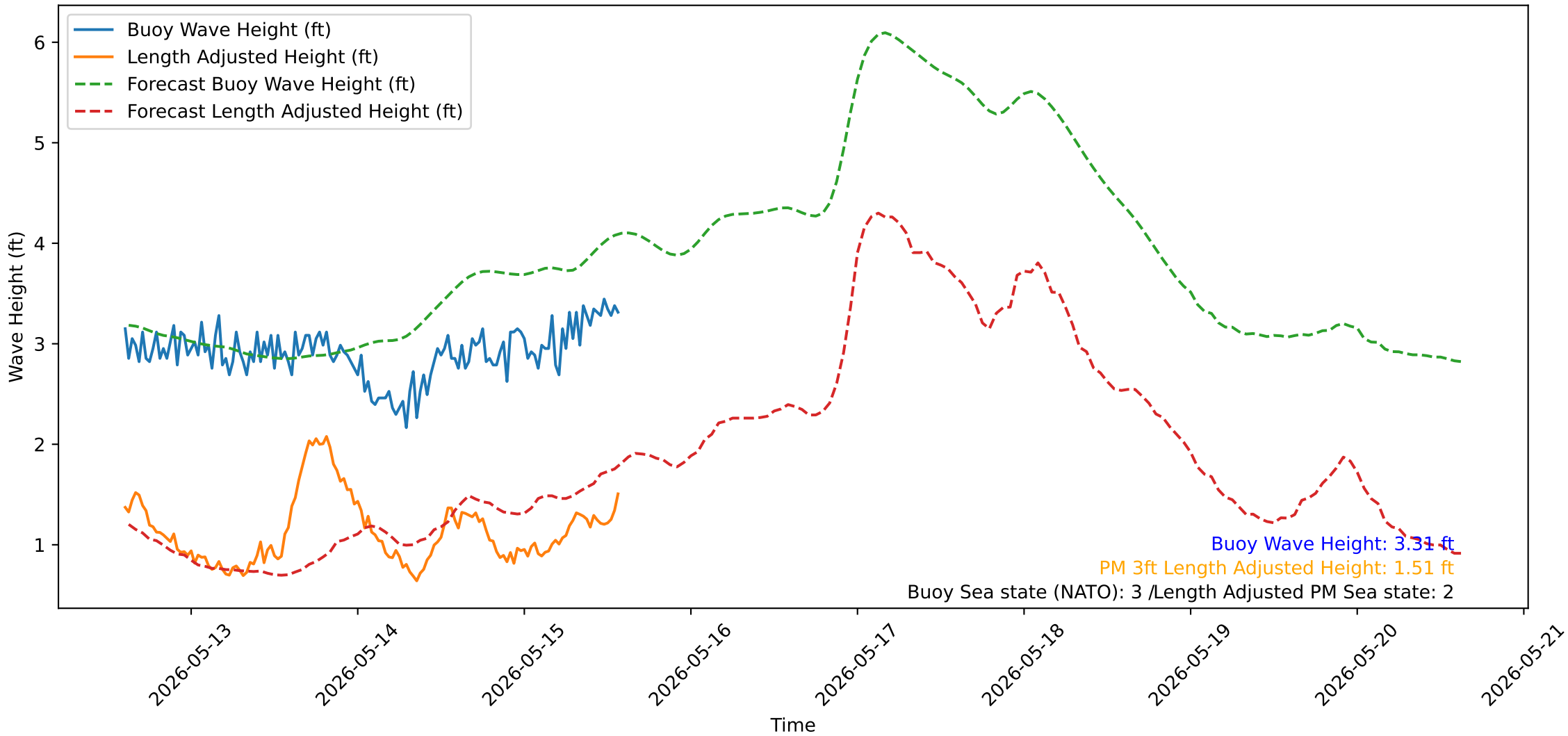
Wave Heights over Time for Oceanside Harbor at 2026-05-15 14:30:32
