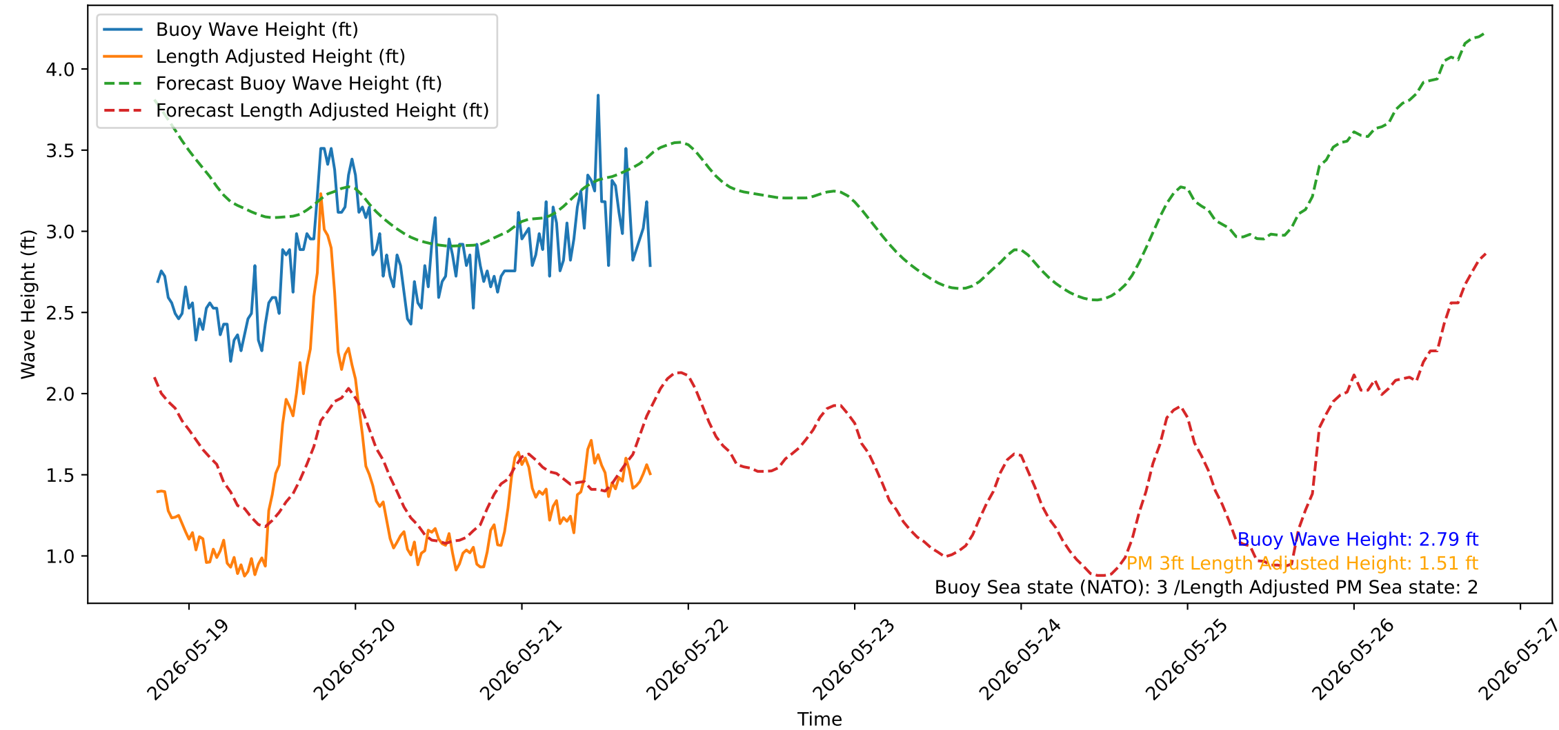
Wave Heights over Time for Oceanside Harbor at 2026-05-21 19:20:31
