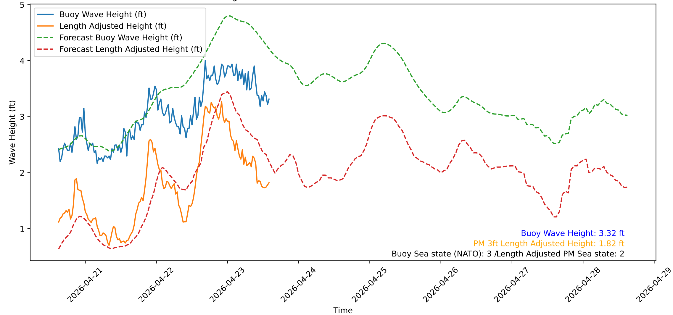
Wave Heights over Time for Green Beach at 2026-04-23 14:51:14
