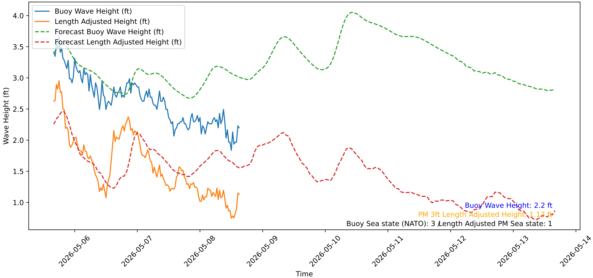
Wave Heights over Time for Green Beach at 2026-05-08 16:01:14
