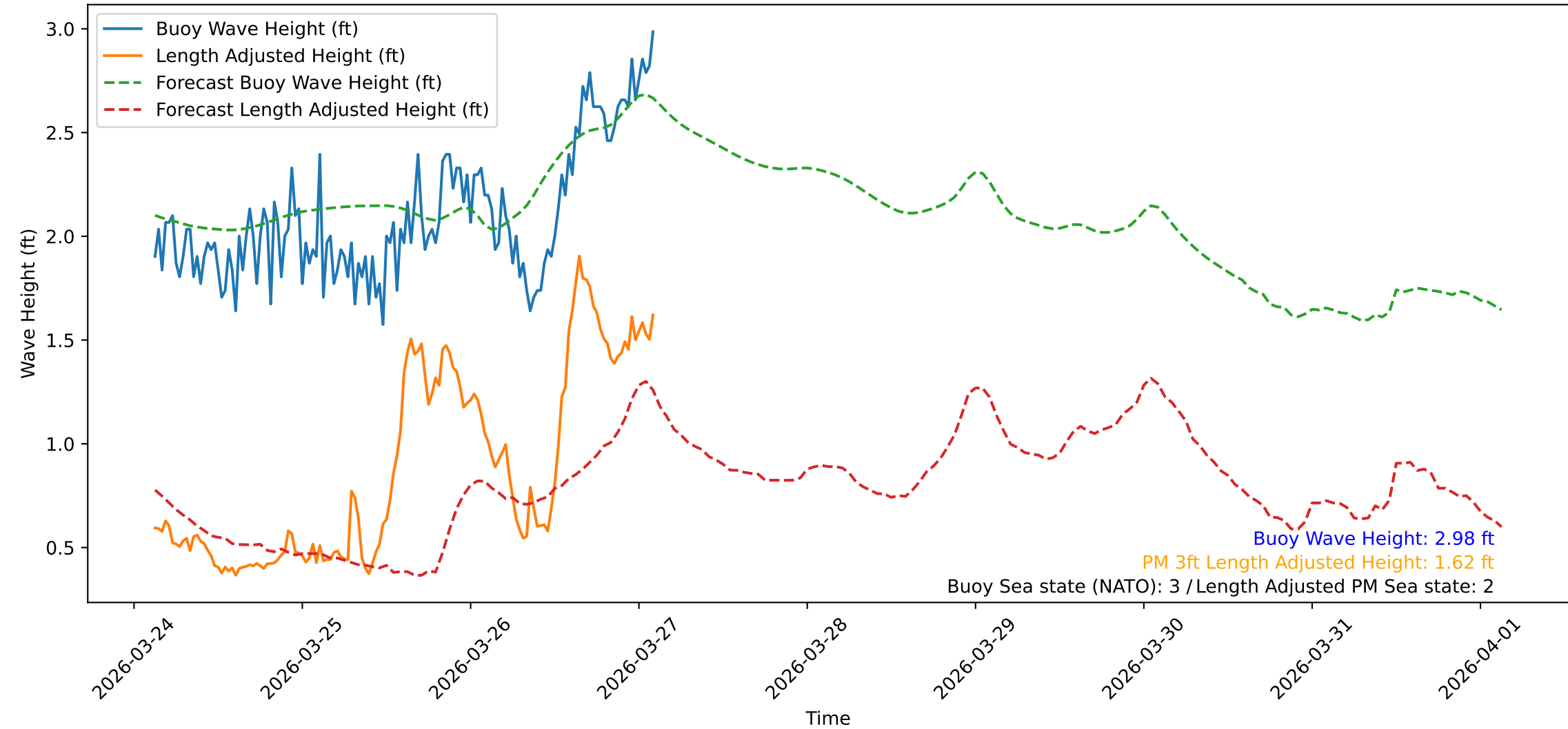
Wave Heights over Time for Red Beach at 2026-03-27 02:50:47
