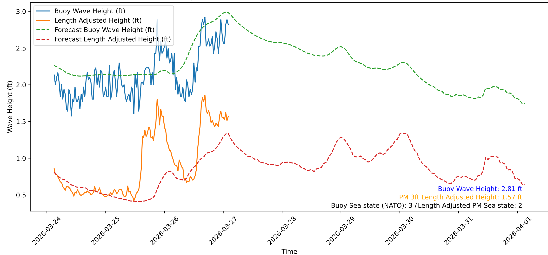
Wave Heights over Time for Oceanside Harbor at 2026-03-27 02:50:31
