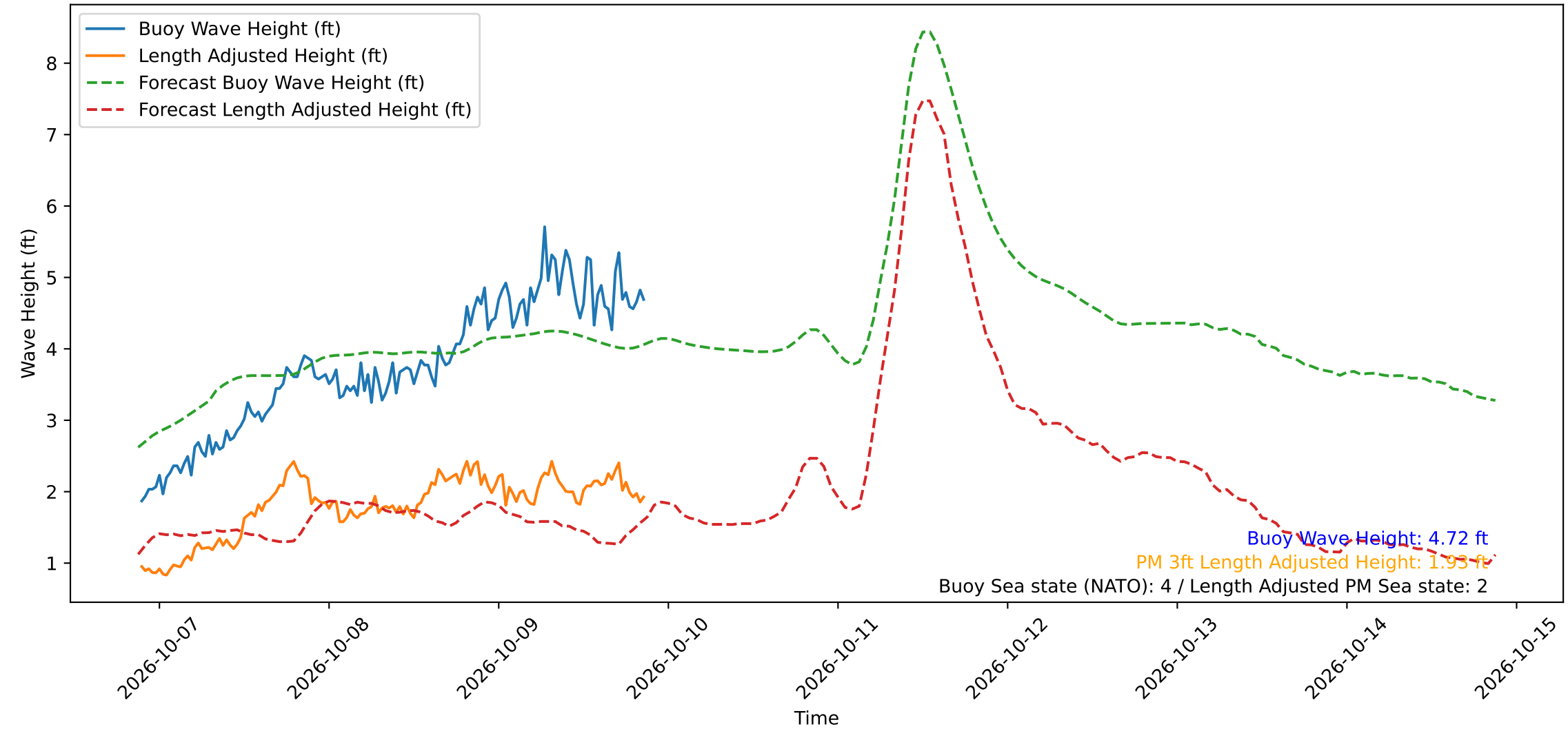
Wave Heights over Time for Red Beach at 2026-10-09 21:20:51
