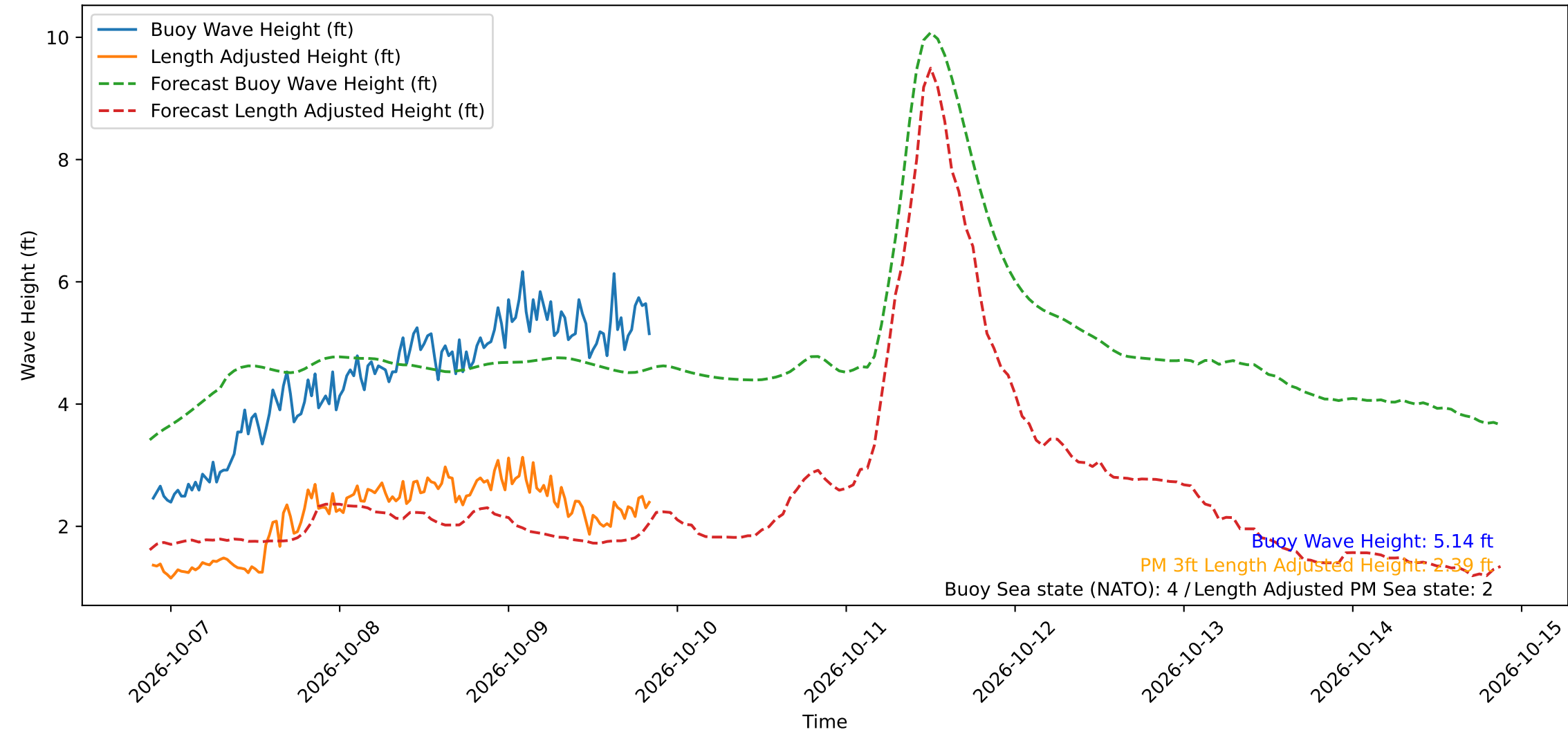
Wave Heights over Time for Green Beach at 2026-10-09 21:21:15
