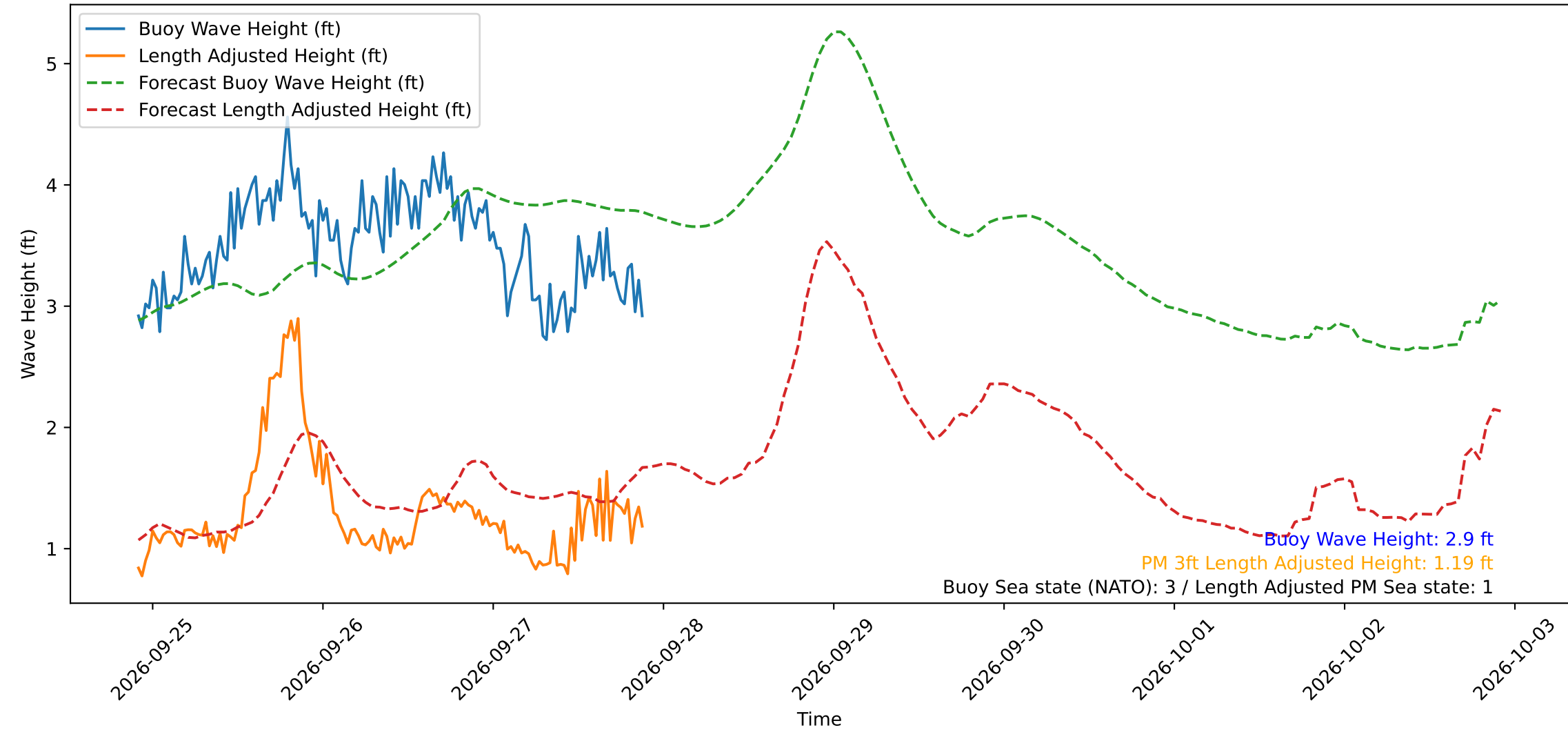
Wave Heights over Time for Green Beach at 2026-09-27 21:51:18
