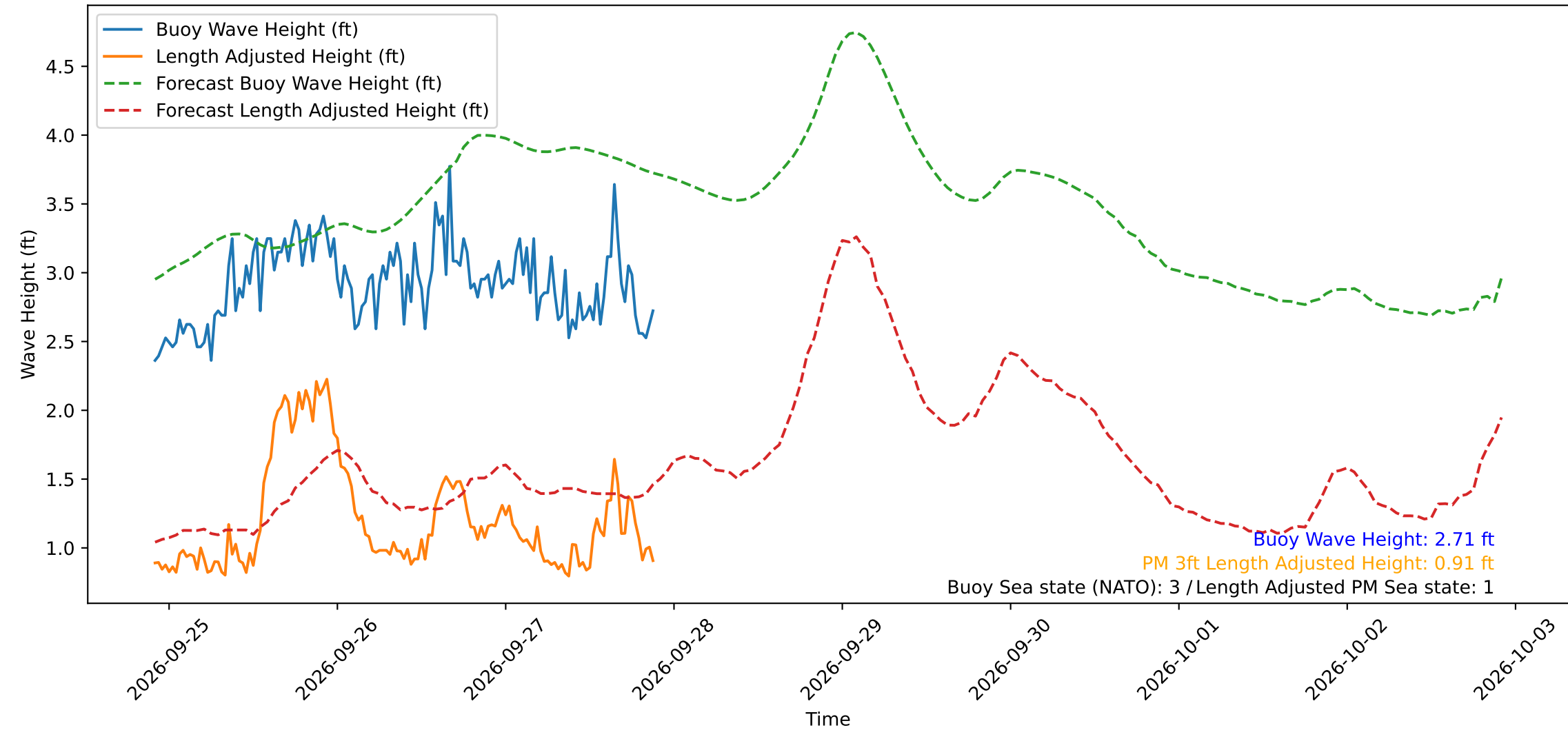
Wave Heights over Time for Oceanside Harbor at 2026-09-27 21:50:31
