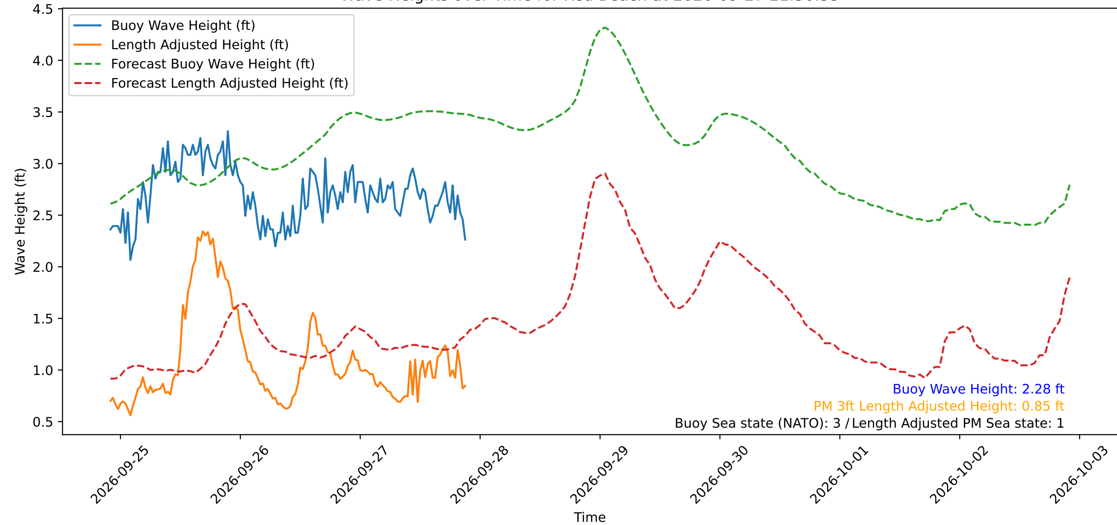
Wave Heights over Time for Red Beach at 2026-09-27 21:50:53
