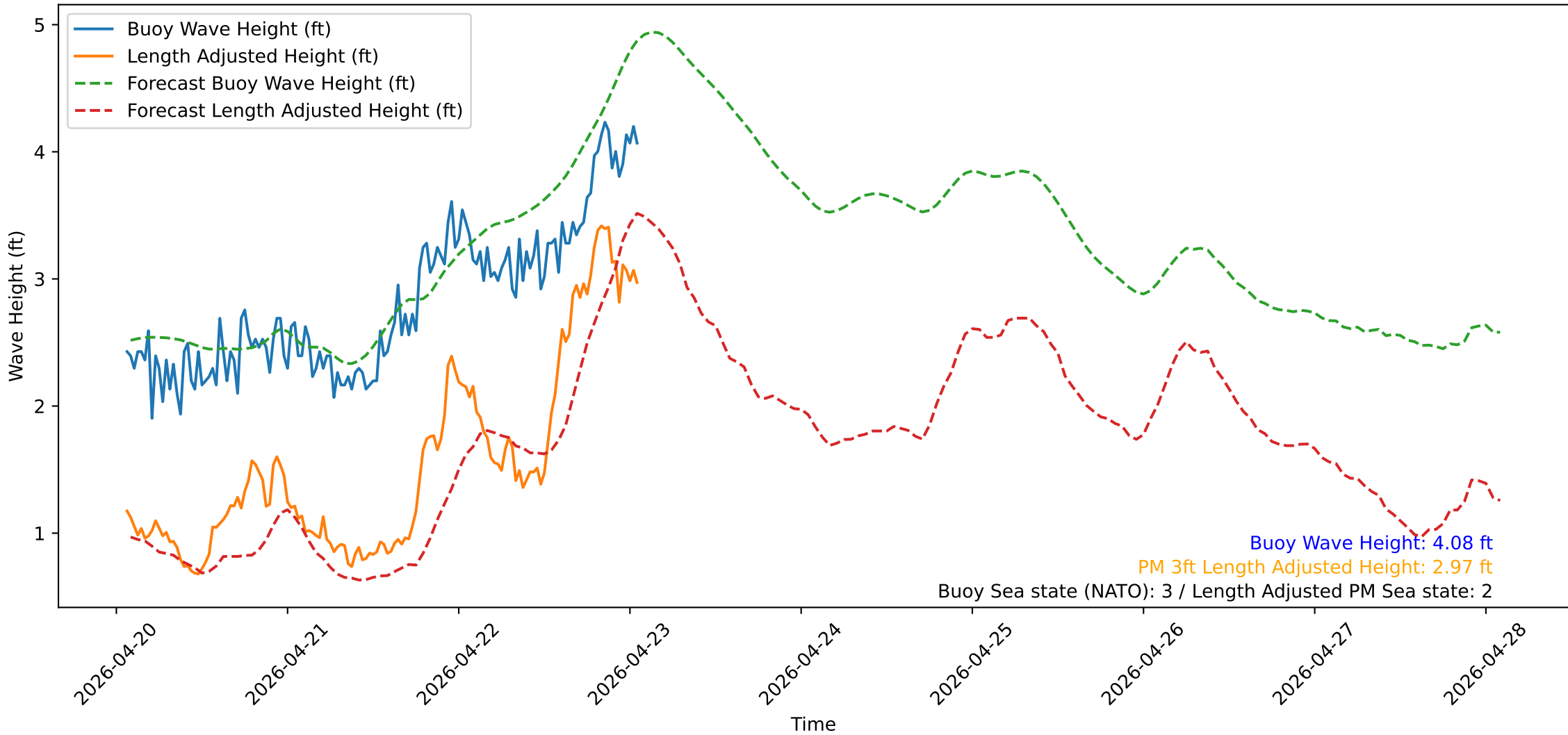
Wave Heights over Time for Oceanside Harbor at 2026-04-23 01:40:30
