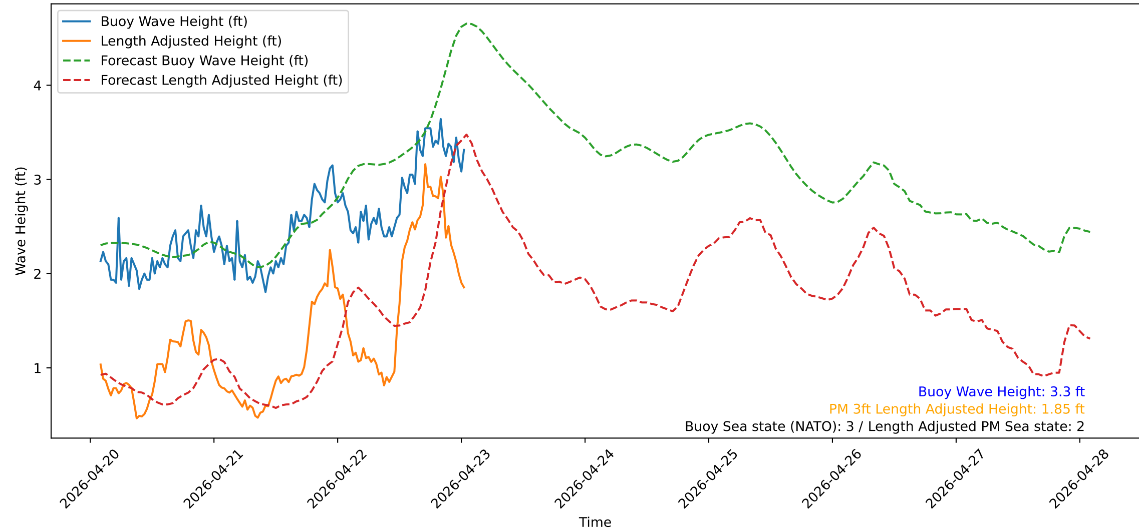
Wave Heights over Time for Red Beach at 2026-04-23 01:40:49
