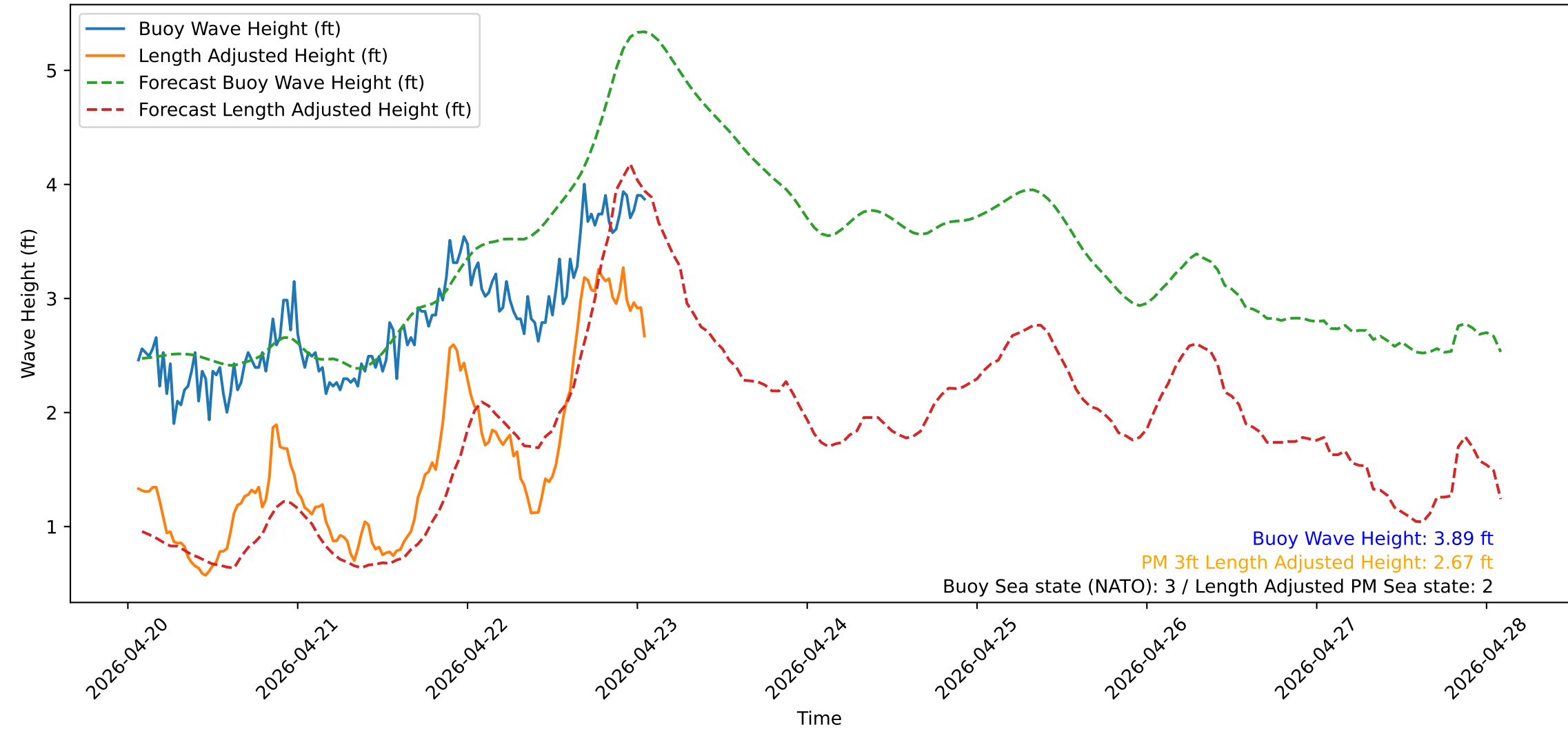
Wave Heights over Time for Green Beach at 2026-04-23 01:41:12
