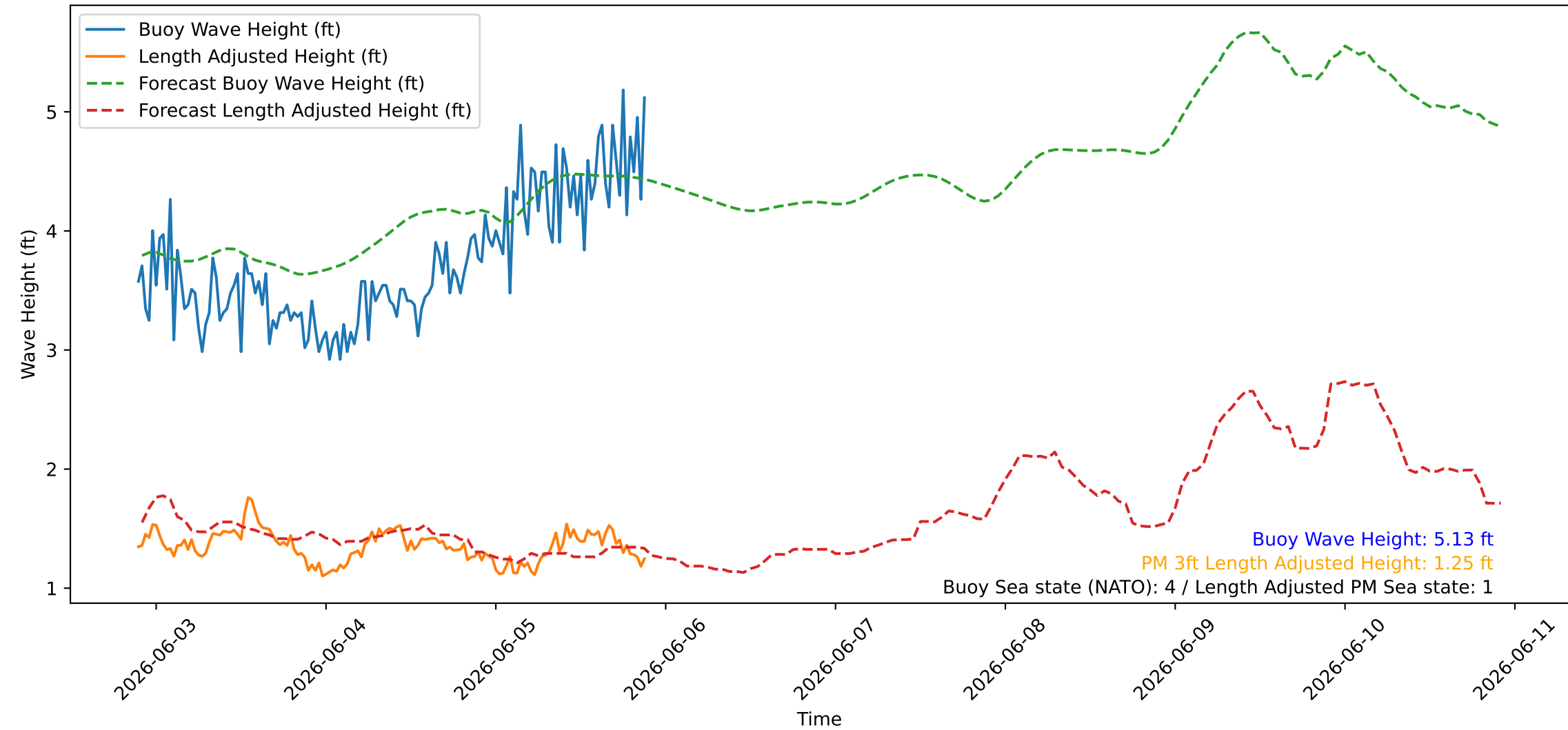
Wave Heights over Time for Oceanside Harbor at 2026-06-05 21:40:27
