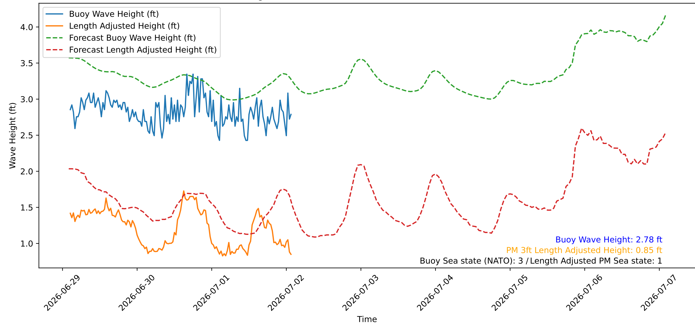
Wave Heights over Time for Red Beach at 2026-07-02 02:10:45
