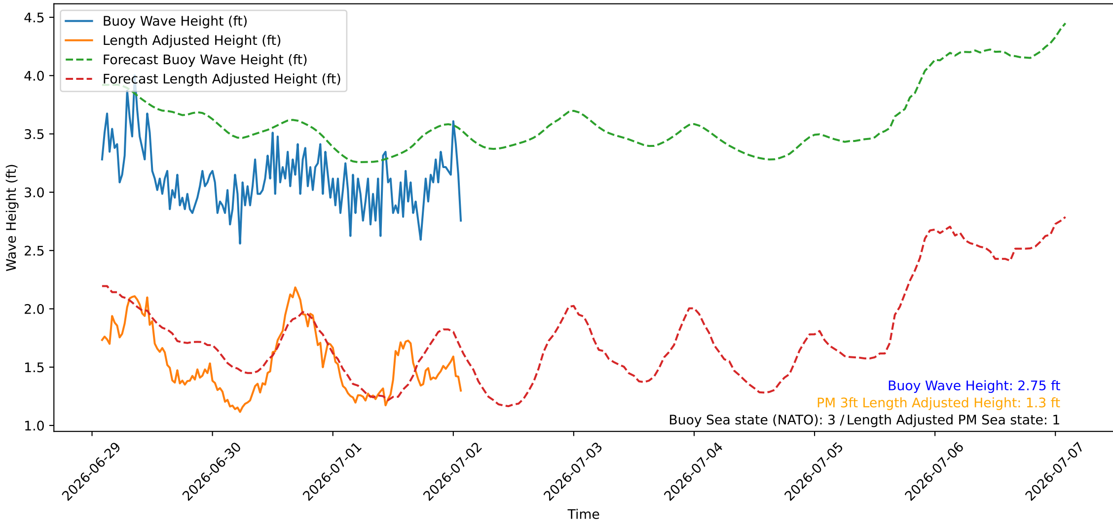
Wave Heights over Time for Oceanside Harbor at 2026-07-02 02:10:26
