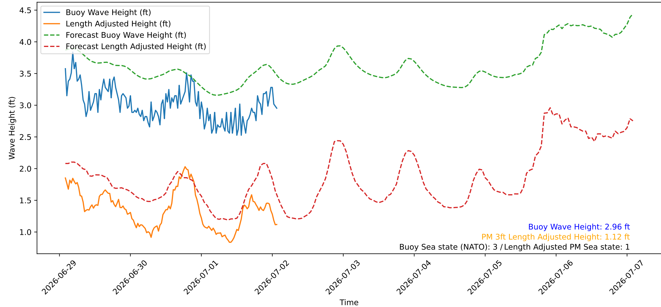
Wave Heights over Time for Green Beach at 2026-07-02 02:11:07
