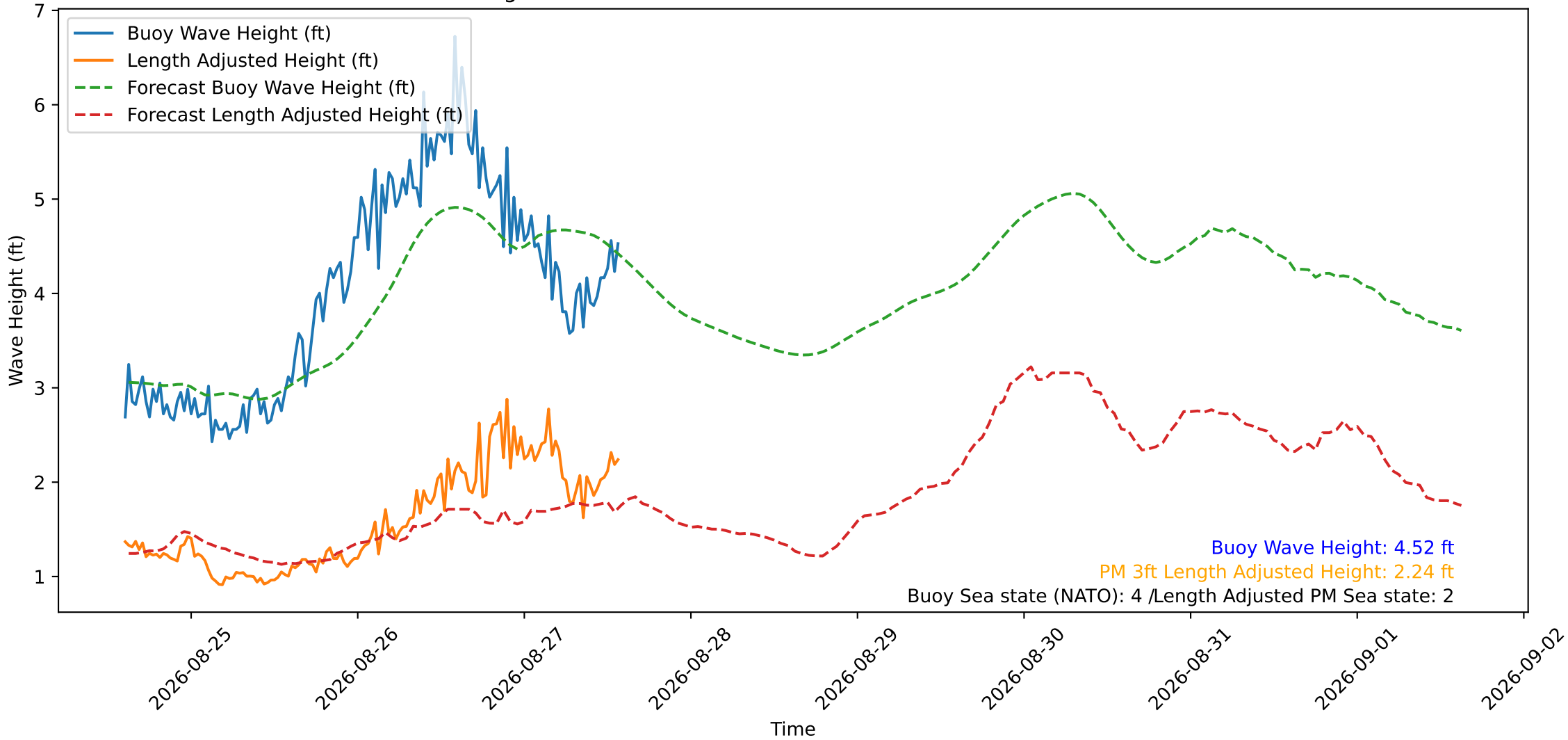
Wave Heights over Time for Oceanside Harbor at 2026-08-27 14:30:29
