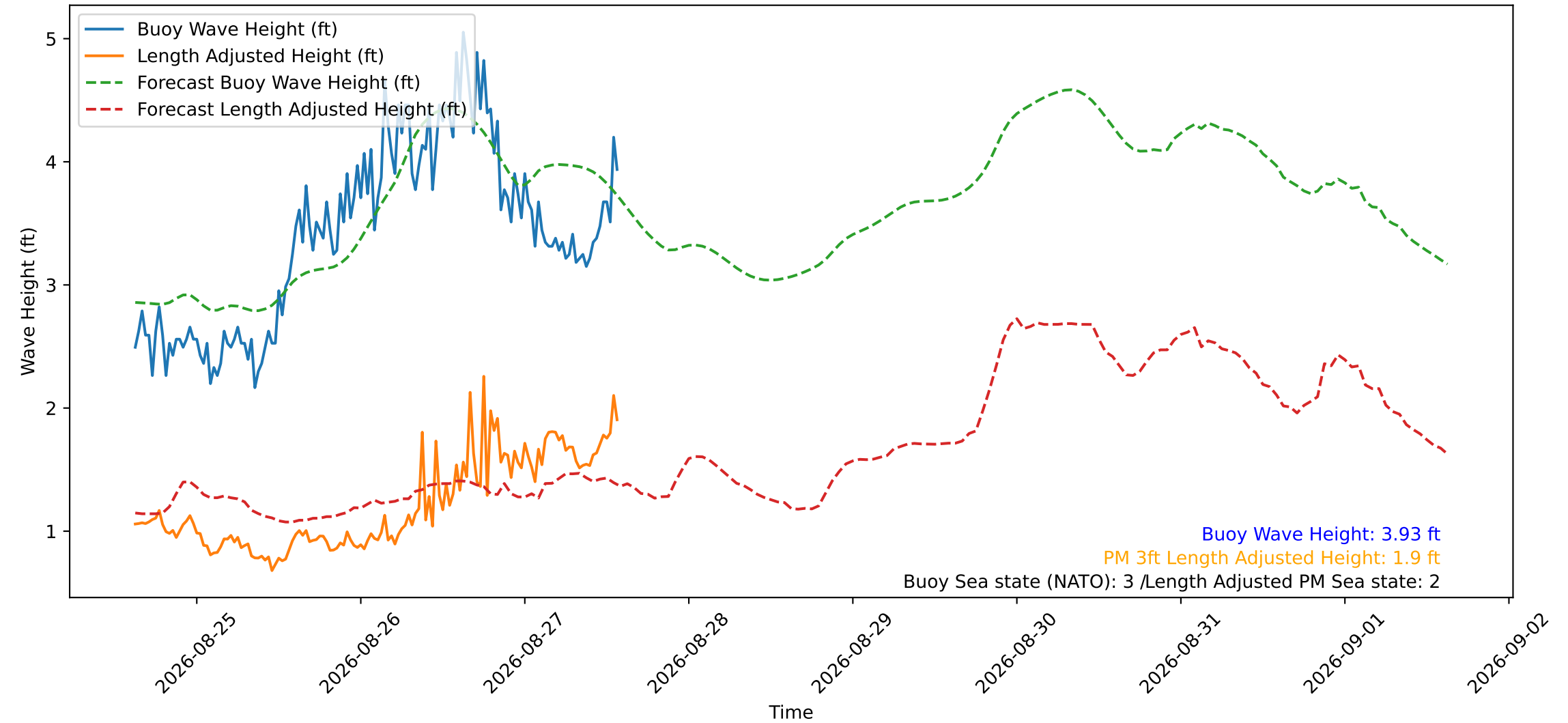
Wave Heights over Time for Red Beach at 2026-08-27 14:30:49
