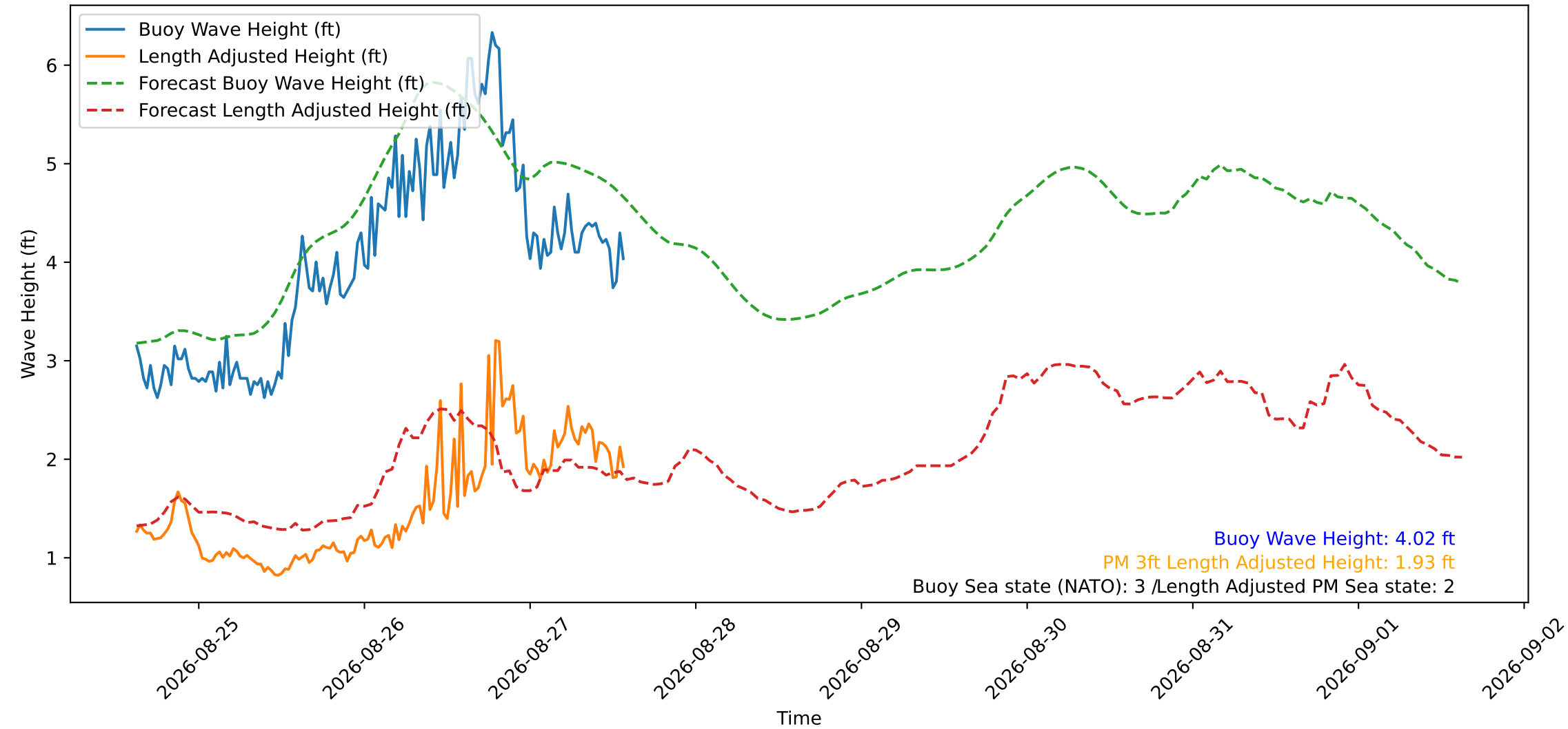
Wave Heights over Time for Green Beach at 2026-08-27 14:31:11
