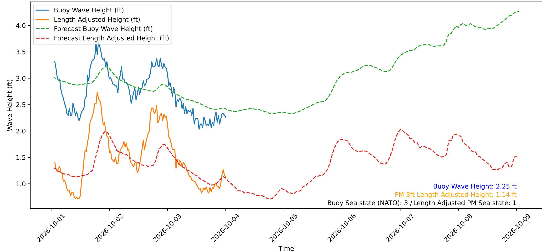
Wave Heights over Time for Green Beach at 2026-10-04 01:01:11
