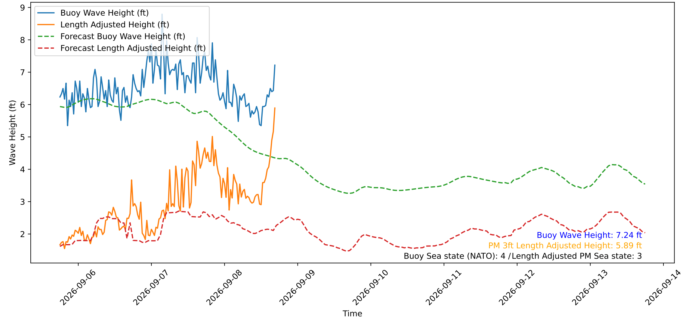
Wave Heights over Time for Green Beach at 2026-09-08 17:31:11
