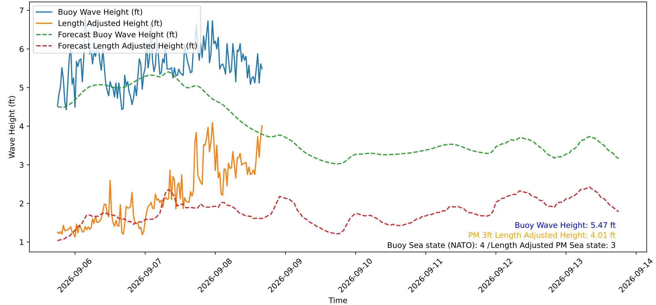
Wave Heights over Time for Red Beach at 2026-09-08 17:30:49
