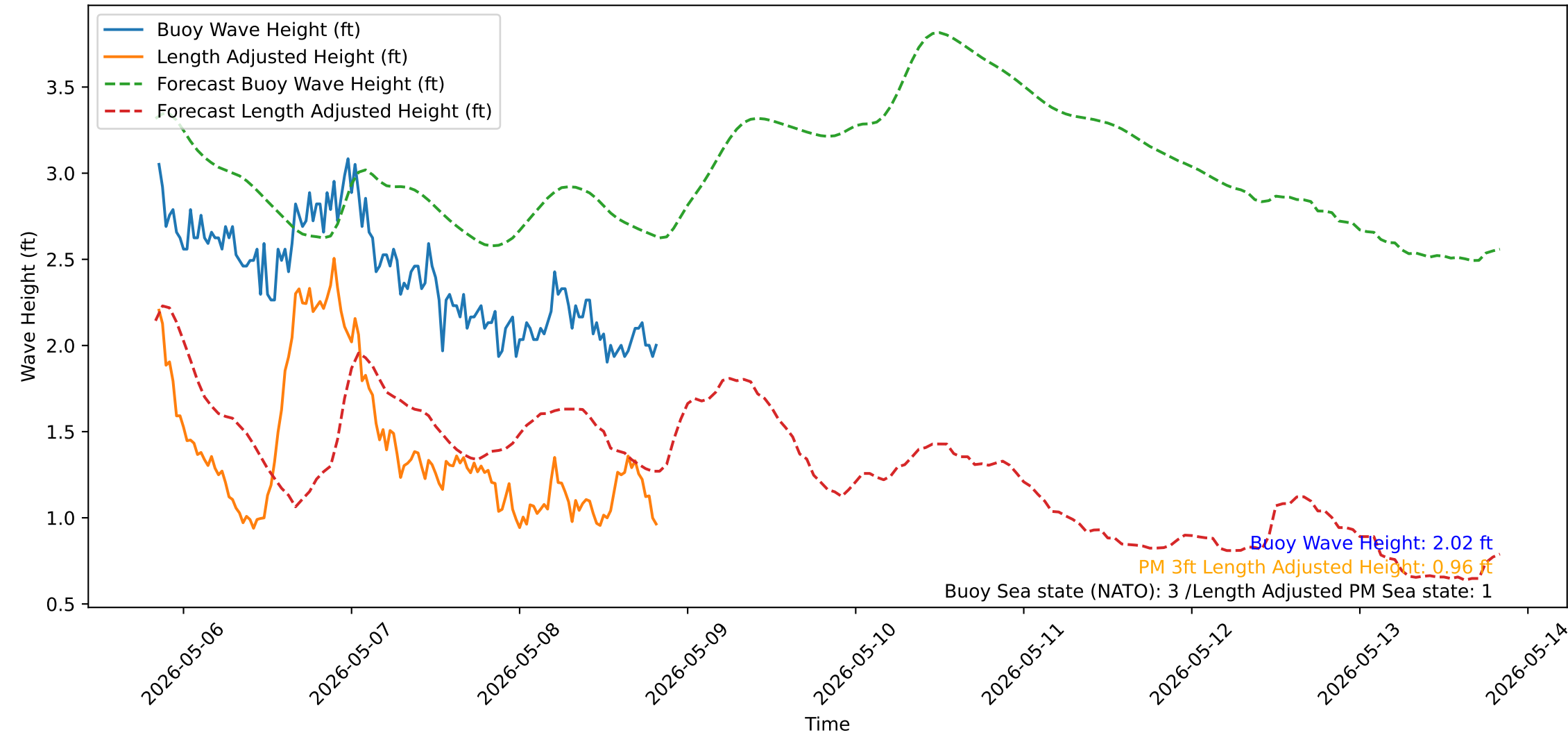
Wave Heights over Time for Red Beach at 2026-05-08 20:20:52
