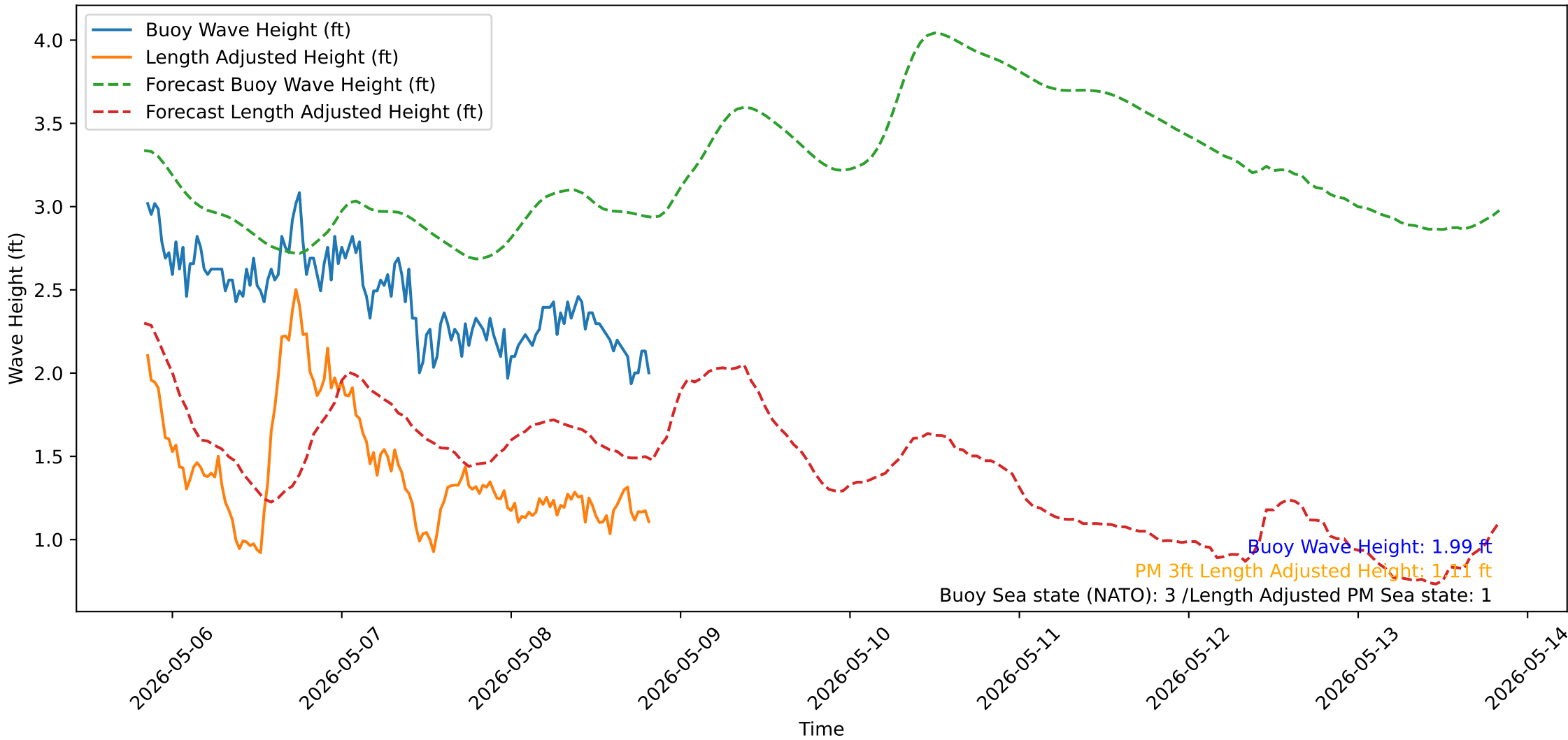
Wave Heights over Time for Oceanside Harbor at 2026-05-08 20:20:32
