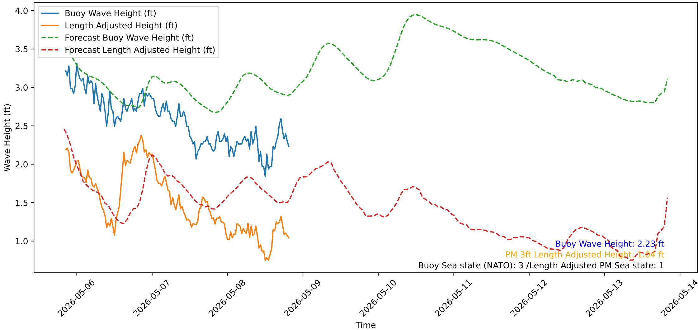
Wave Heights over Time for Green Beach at 2026-05-08 20:21:15
