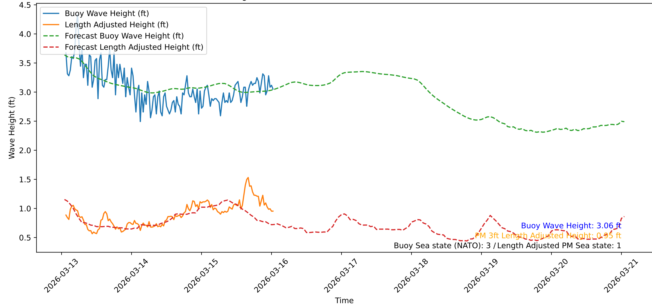
Wave Heights over Time for Red Beach at 2026-03-16 01:21:11
