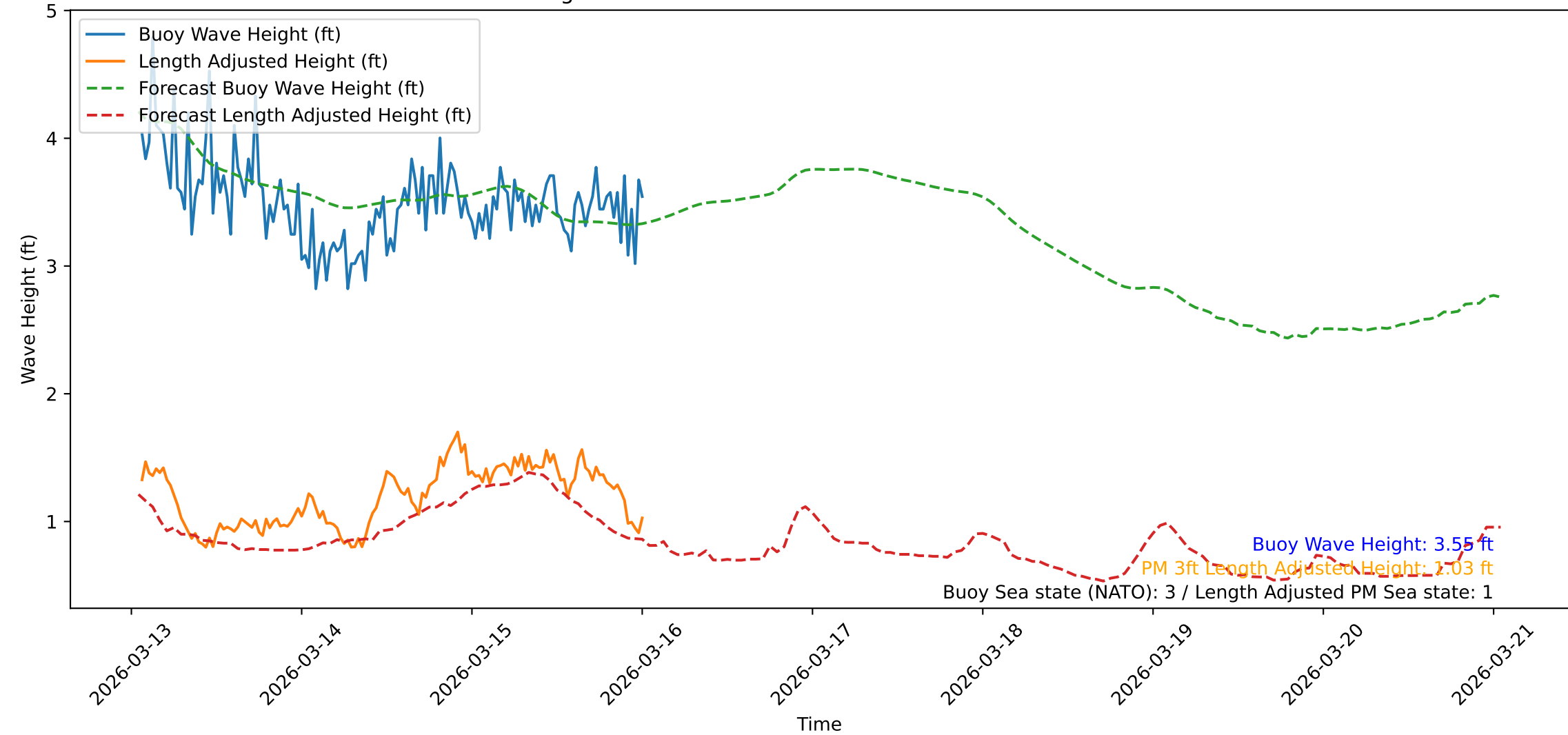
Wave Heights over Time for Green Beach at 2026-03-16 01:21:45
