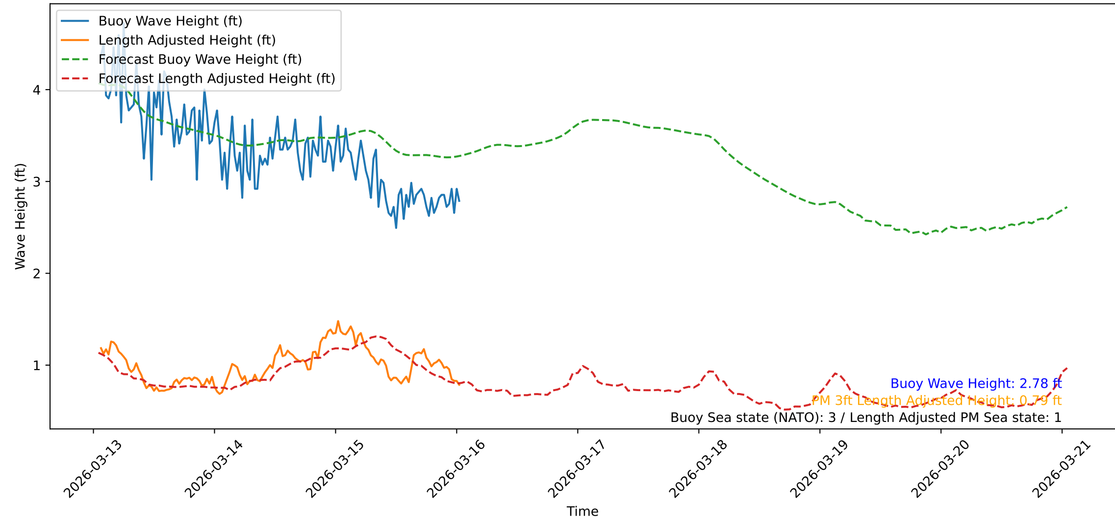
Wave Heights over Time for Oceanside Harbor at 2026-03-16 01:20:43
