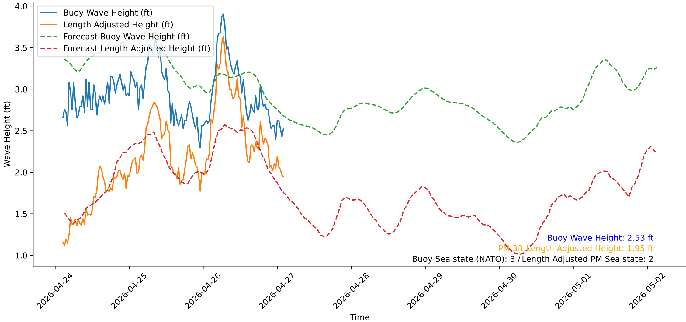
Wave Heights over Time for Oceanside Harbor at 2026-04-27 02:30:31
