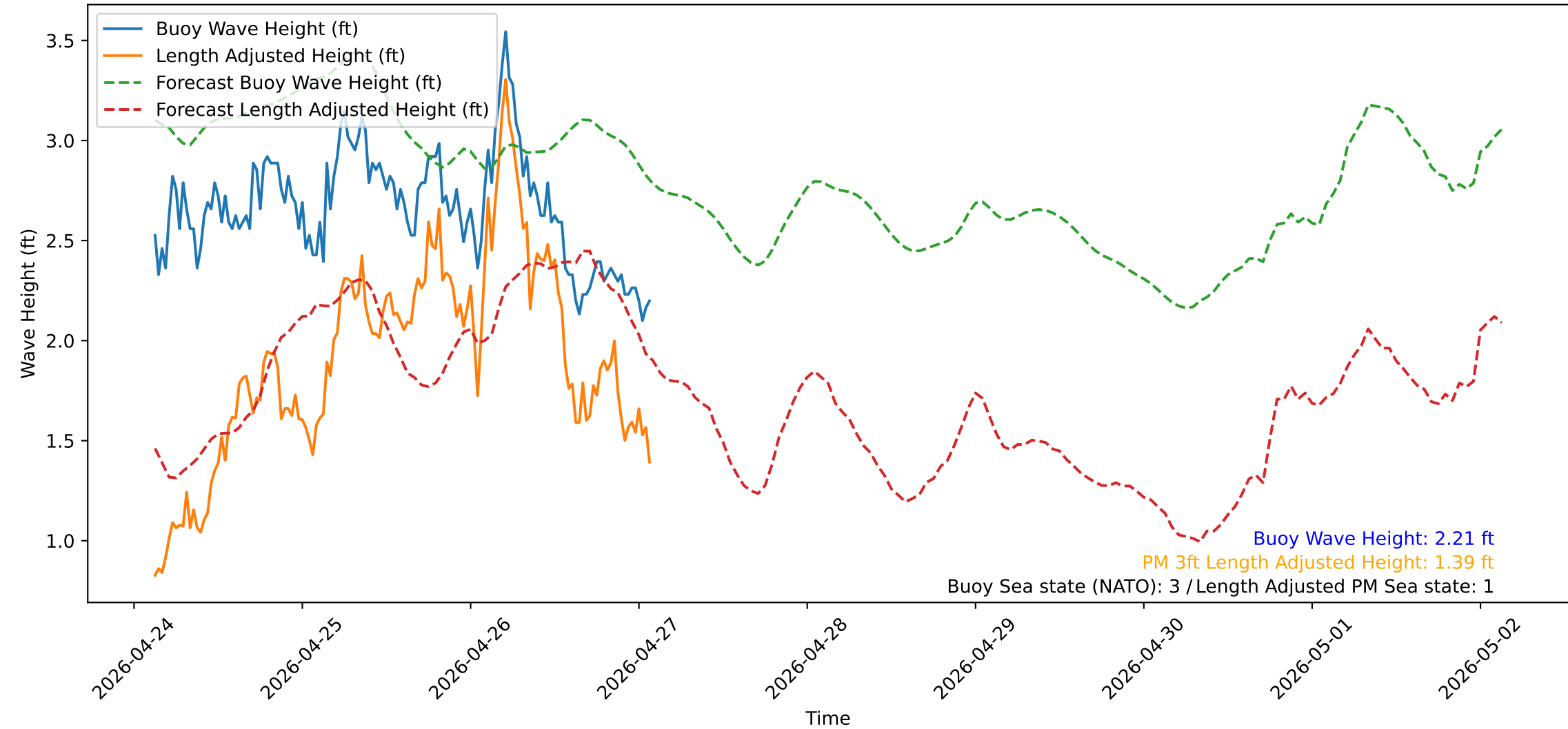
Wave Heights over Time for Red Beach at 2026-04-27 02:30:50
