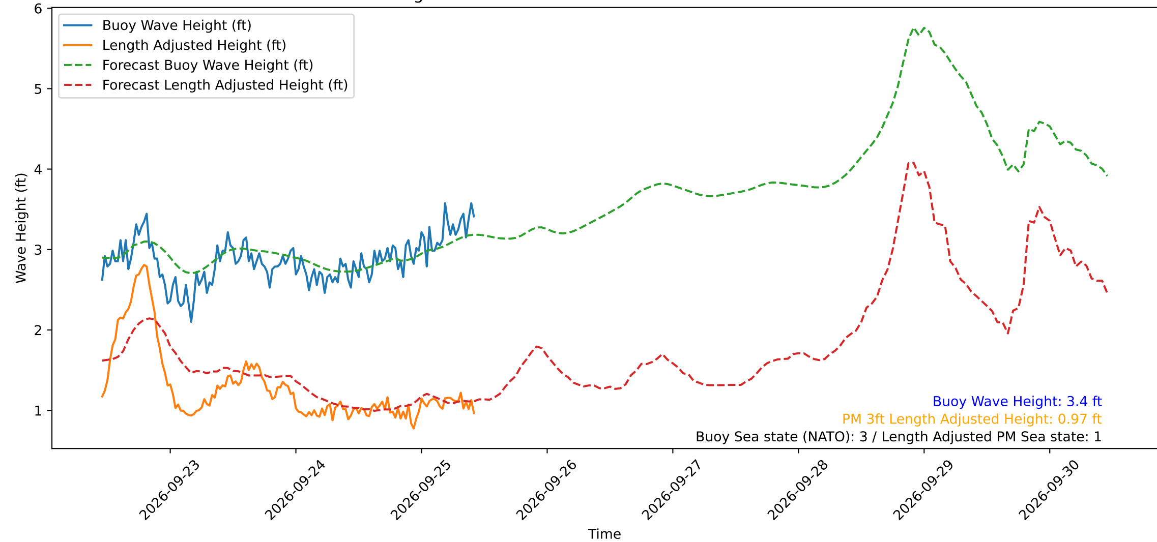
Wave Heights over Time for Green Beach at 2026-09-25 10:51:14
