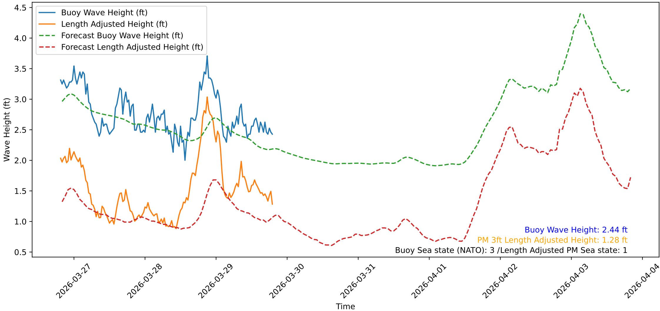
Wave Heights over Time for Green Beach at 2026-03-29 19:41:10
