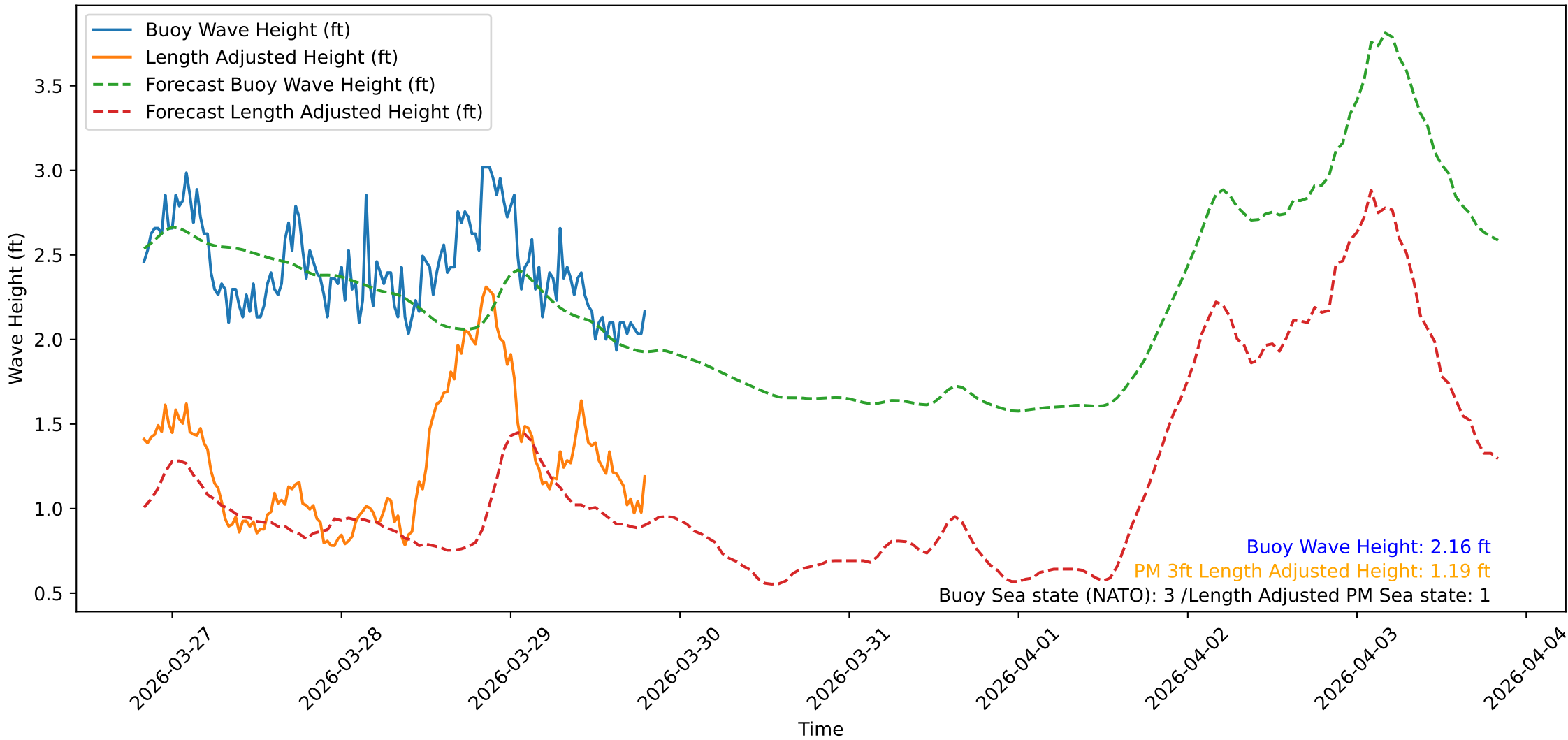
Wave Heights over Time for Red Beach at 2026-03-29 19:40:47
