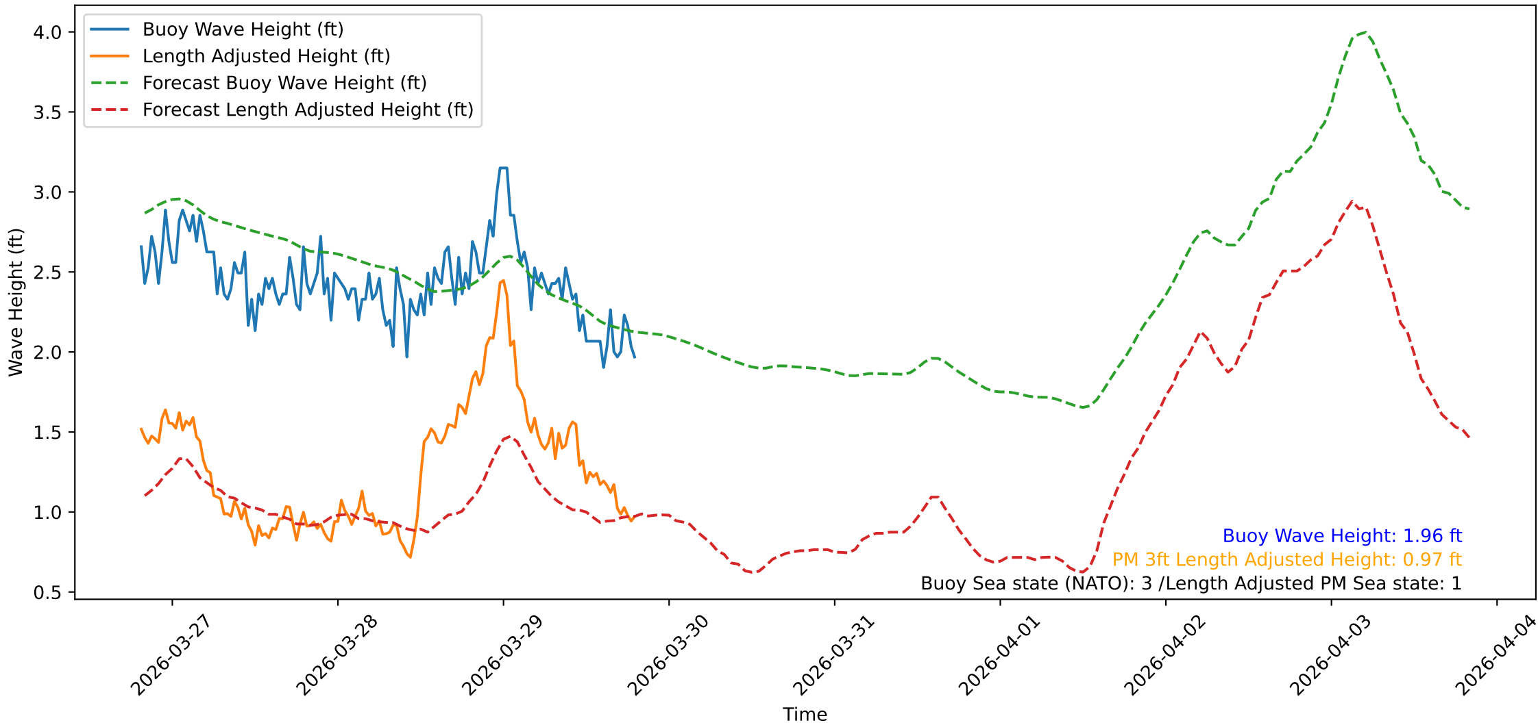
Wave Heights over Time for Oceanside Harbor at 2026-03-29 19:40:31
