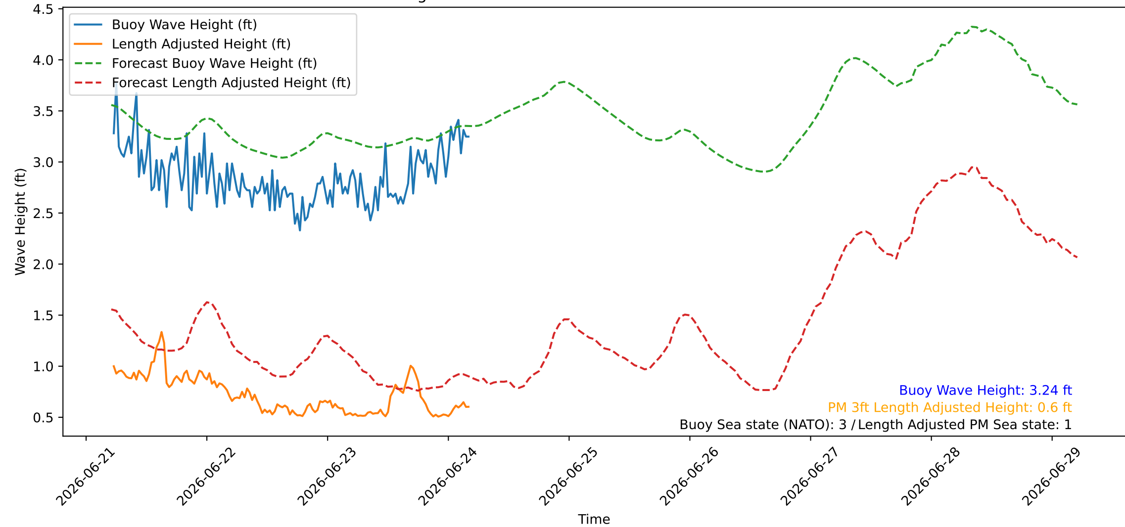
Wave Heights over Time for Red Beach at 2026-06-24 05:00:46
