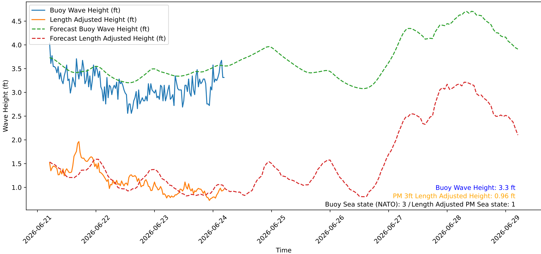
Wave Heights over Time for Oceanside Harbor at 2026-06-24 05:00:26
