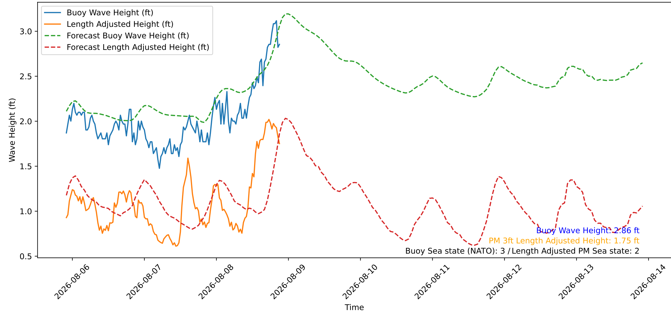
Wave Heights over Time for Red Beach at 2026-08-08 21:40:46
