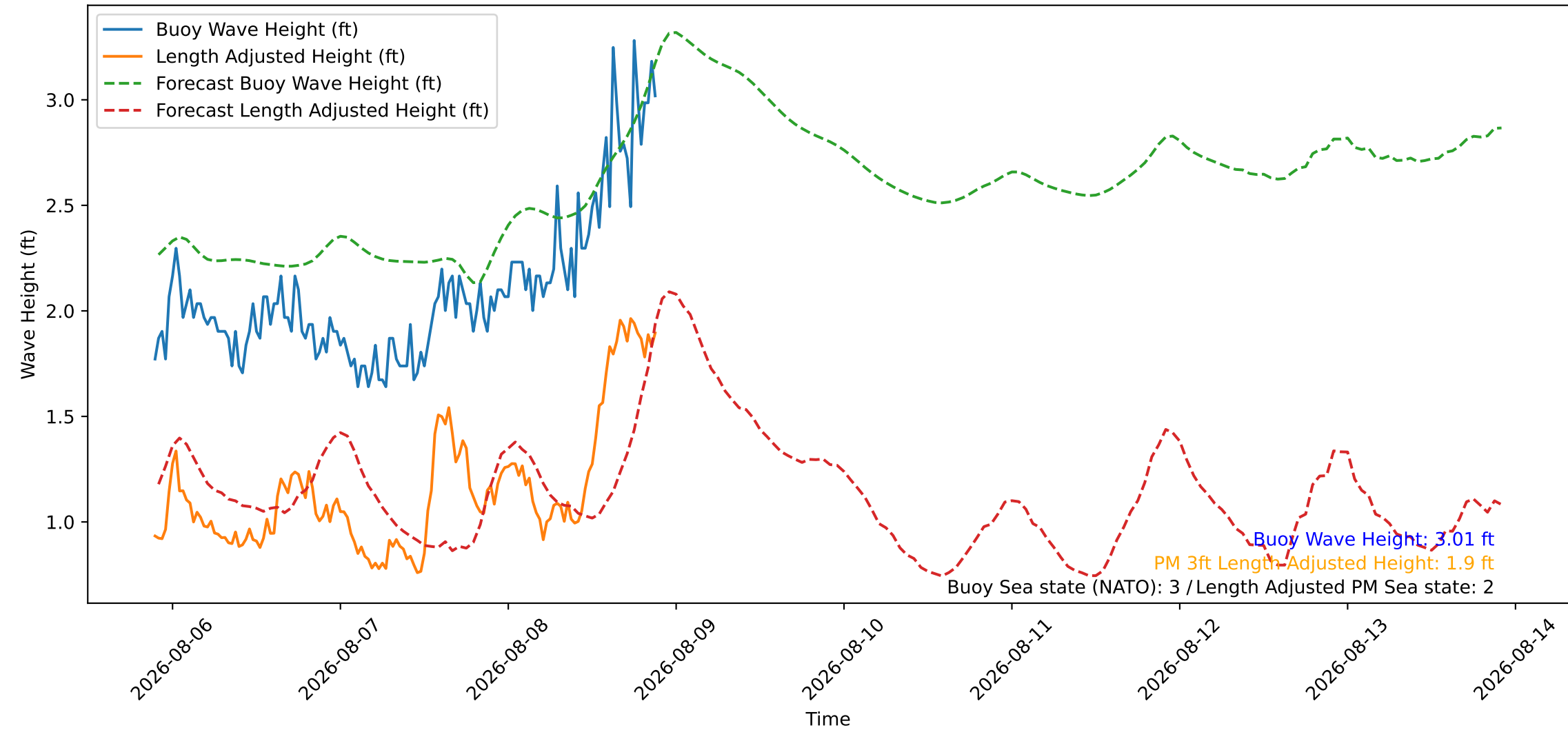
Wave Heights over Time for Oceanside Harbor at 2026-08-08 21:40:26
