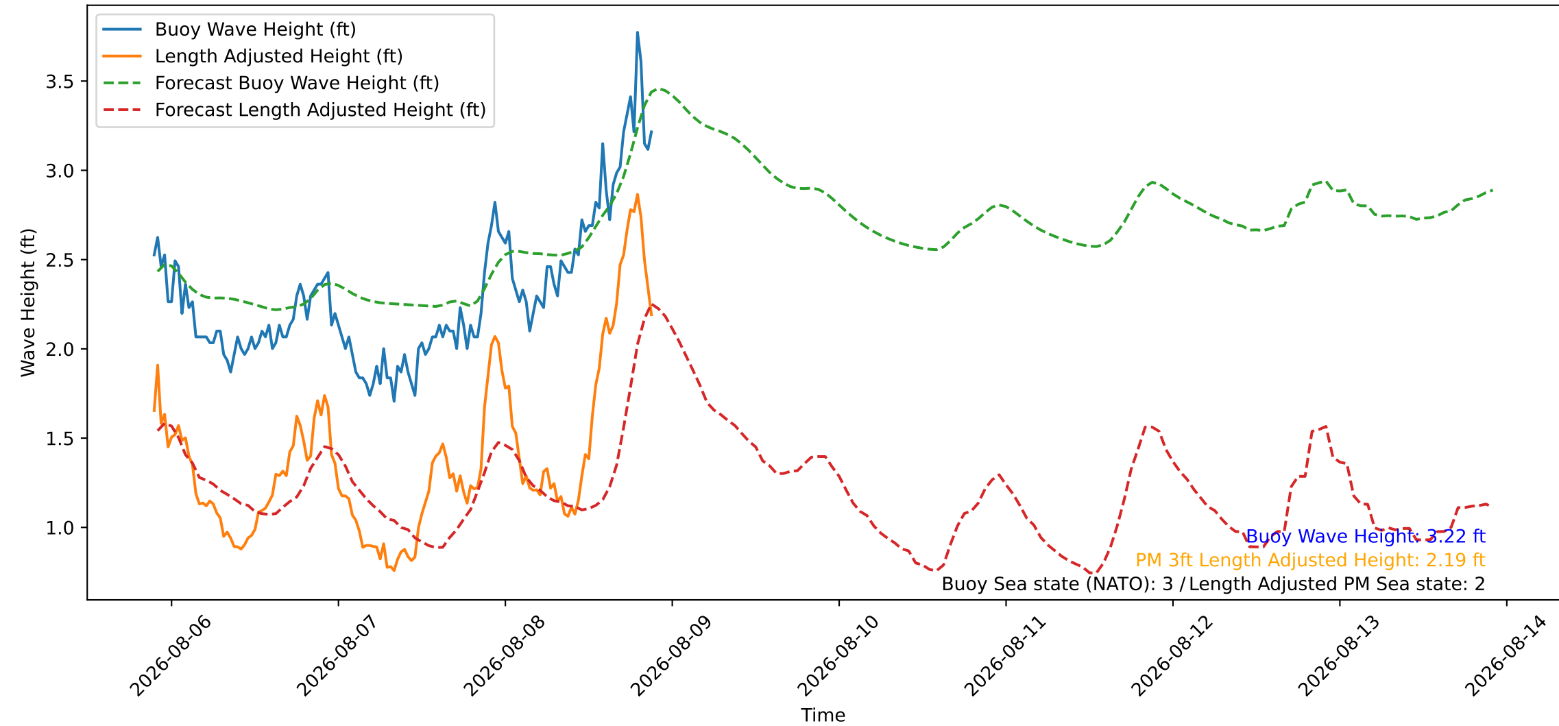
Wave Heights over Time for Green Beach at 2026-08-08 21:41:08
