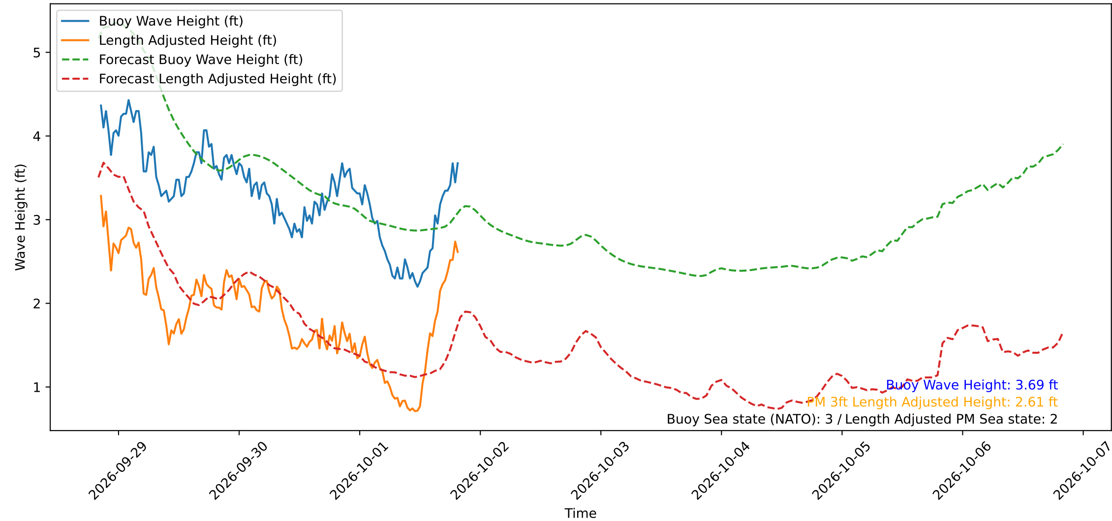
Wave Heights over Time for Green Beach at 2026-10-01 20:21:16
