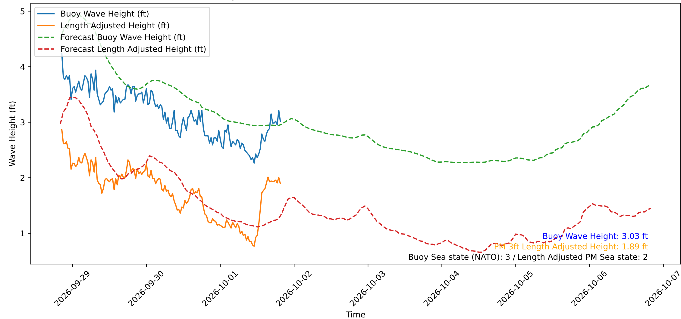
Wave Heights over Time for Oceanside Harbor at 2026-10-01 20:20:30
