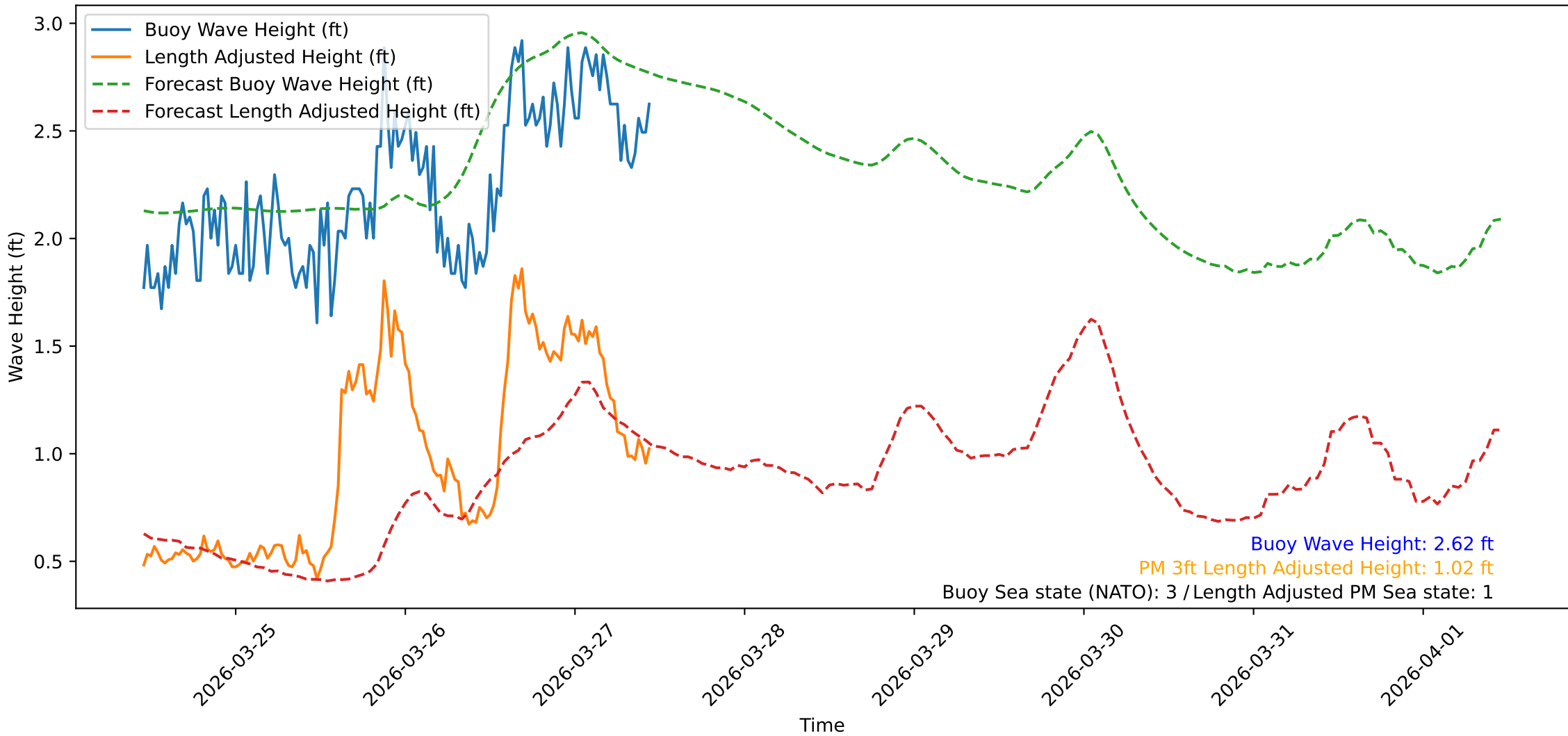
Wave Heights over Time for Oceanside Harbor at 2026-03-27 11:00:31
