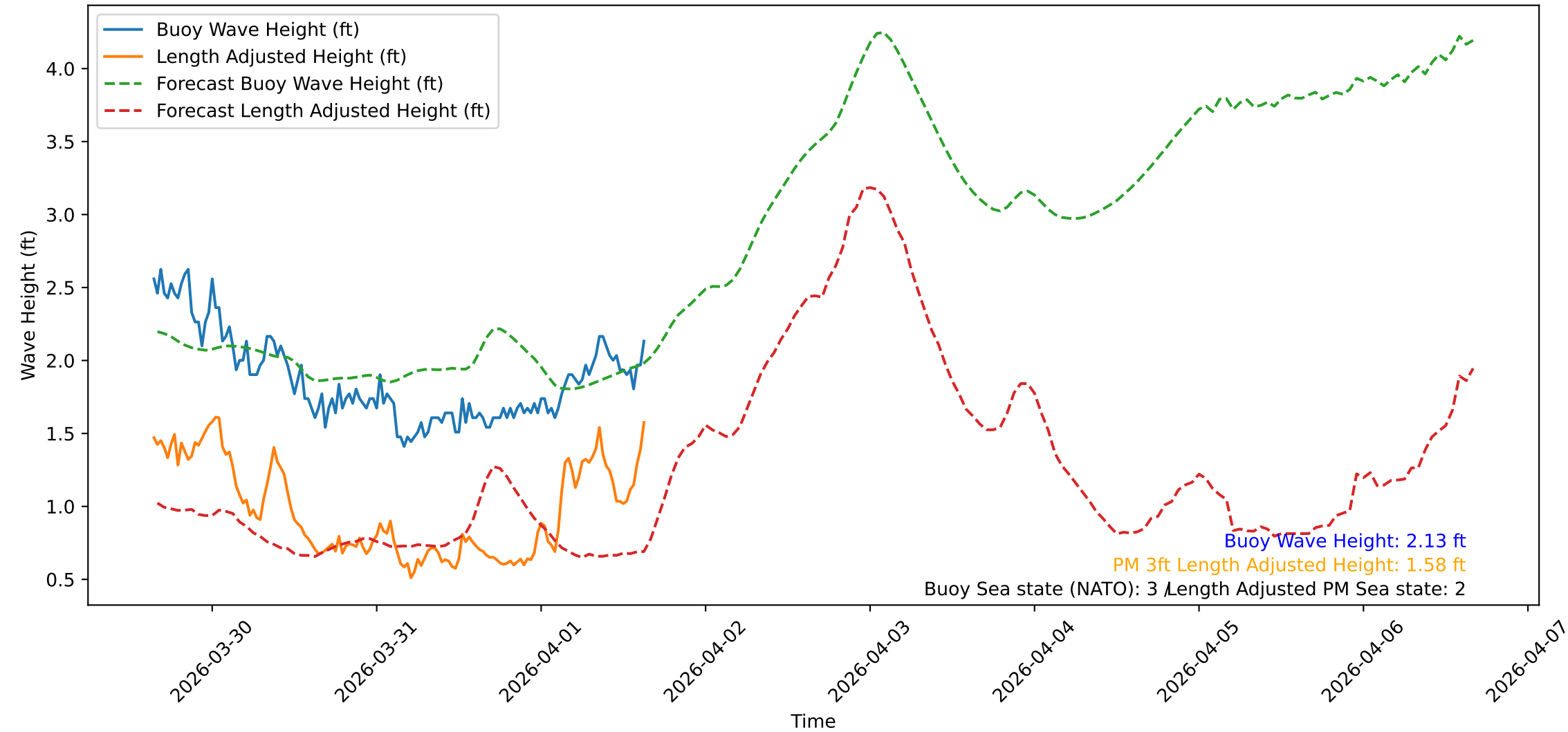
Wave Heights over Time for Green Beach at 2026-04-01 15:41:11
