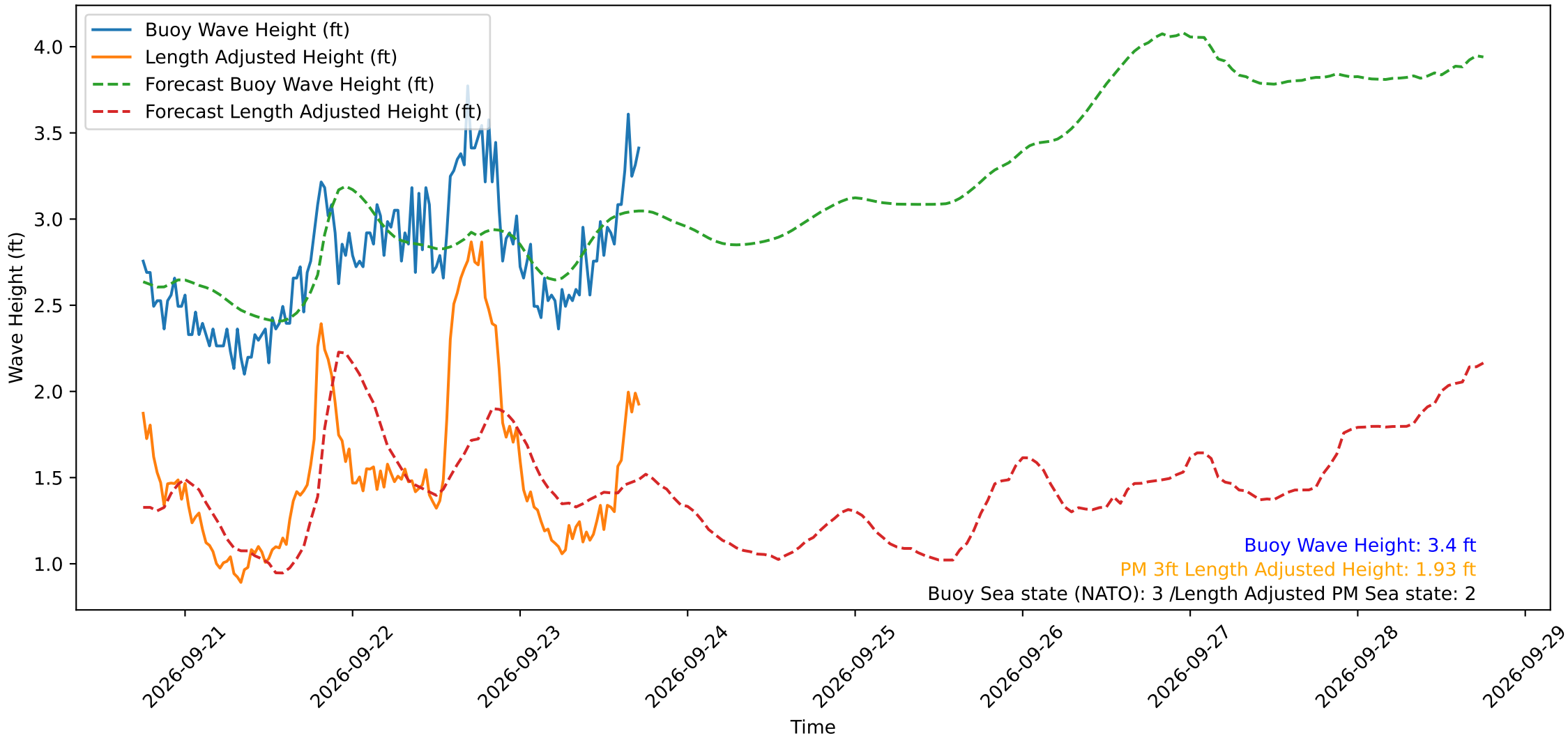
Wave Heights over Time for Oceanside Harbor at 2026-09-23 17:50:30
