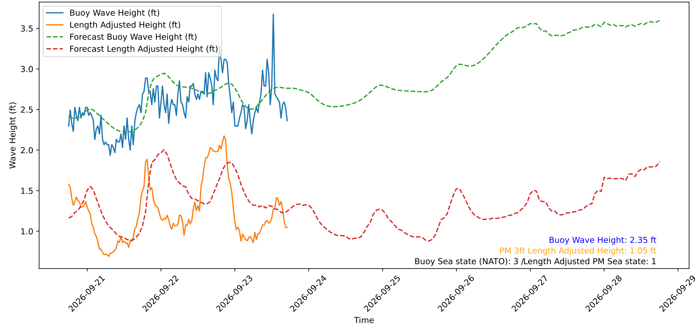
Wave Heights over Time for Red Beach at 2026-09-23 17:50:50
