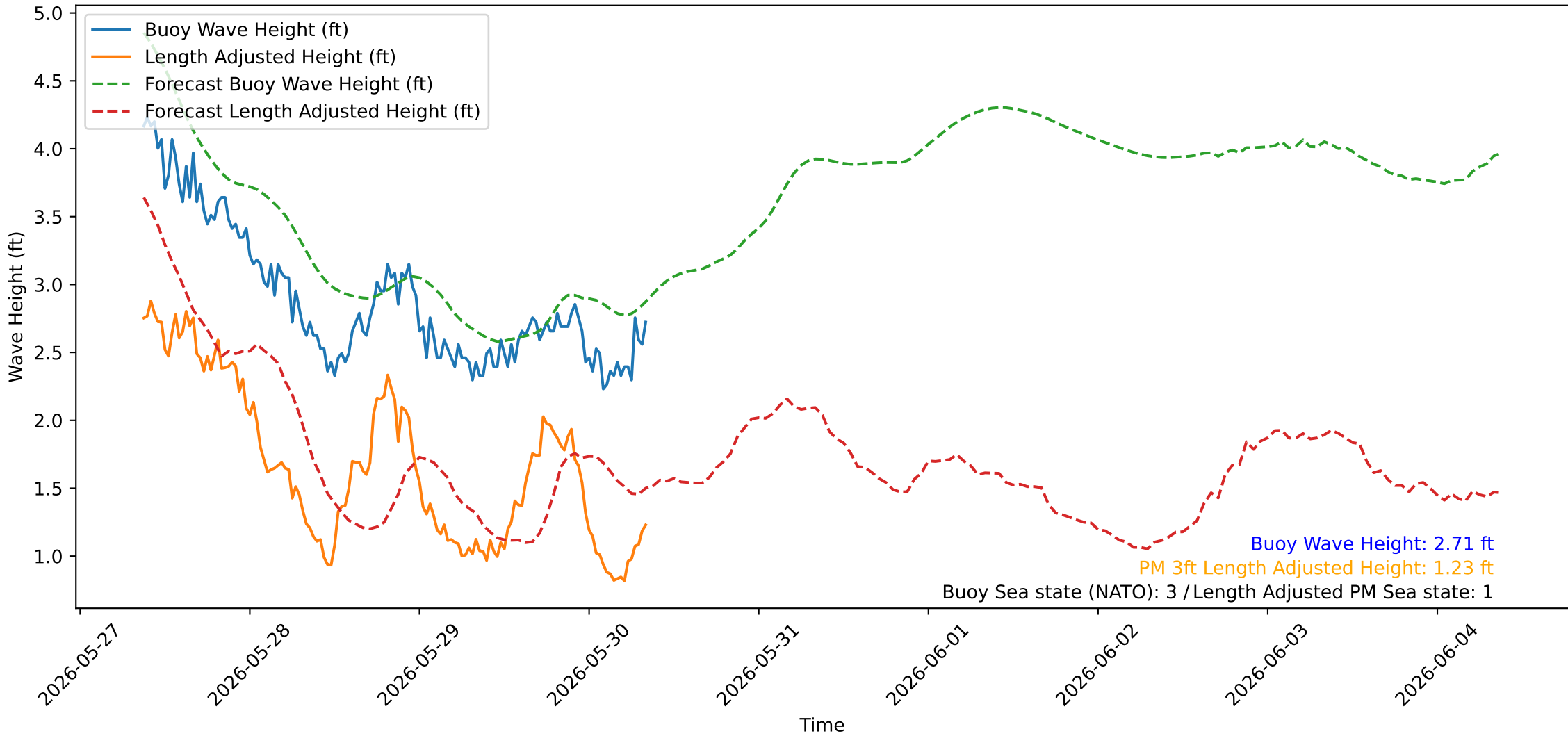
Wave Heights over Time for Red Beach at 2026-05-30 08:50:44
