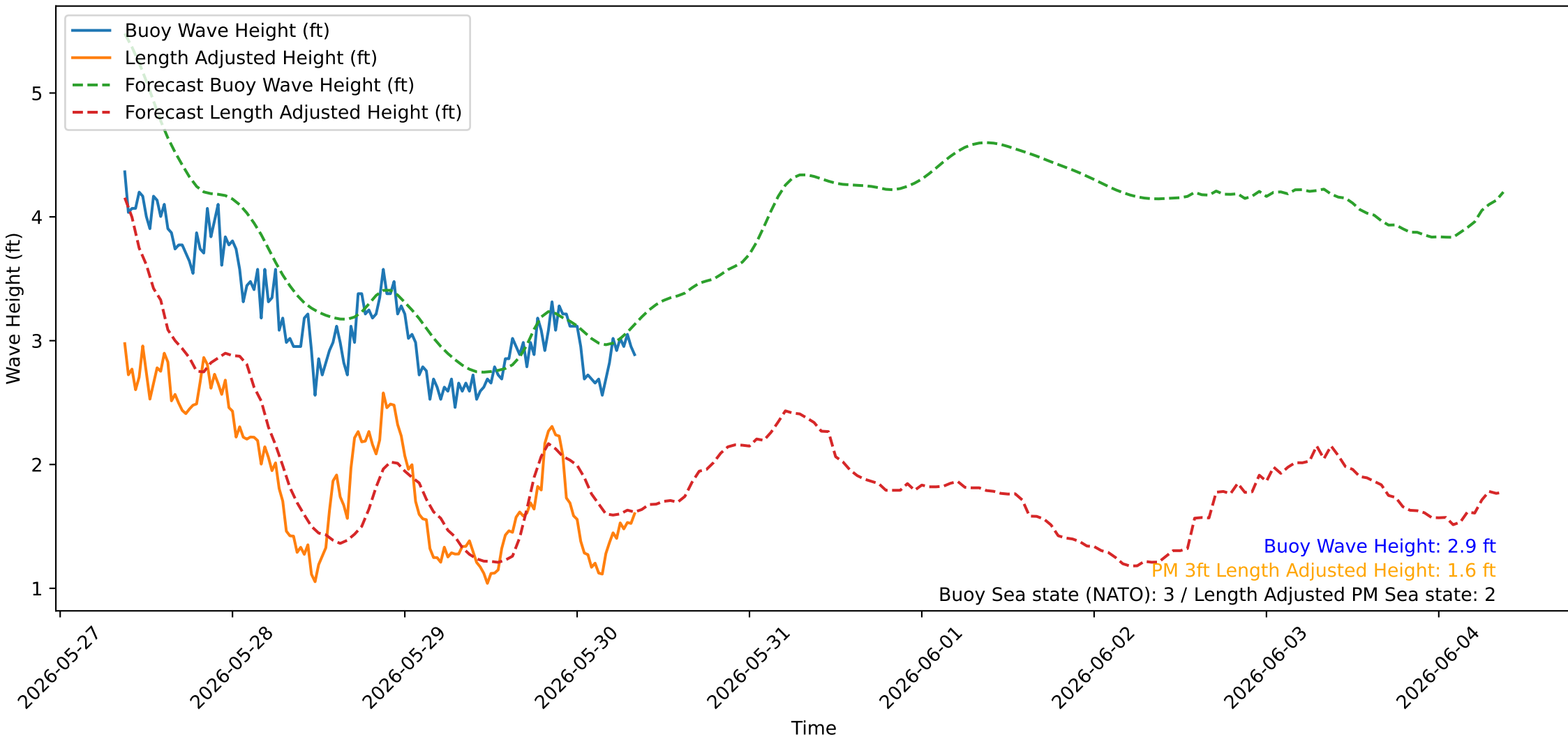
Wave Heights over Time for Green Beach at 2026-05-30 08:51:07
