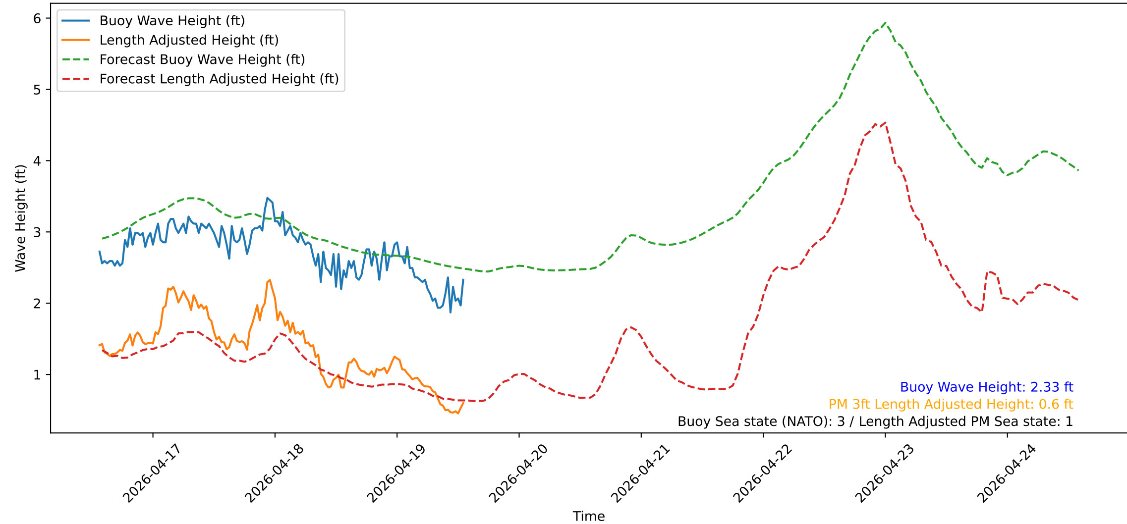
Wave Heights over Time for Green Beach at 2026-04-19 13:41:12
