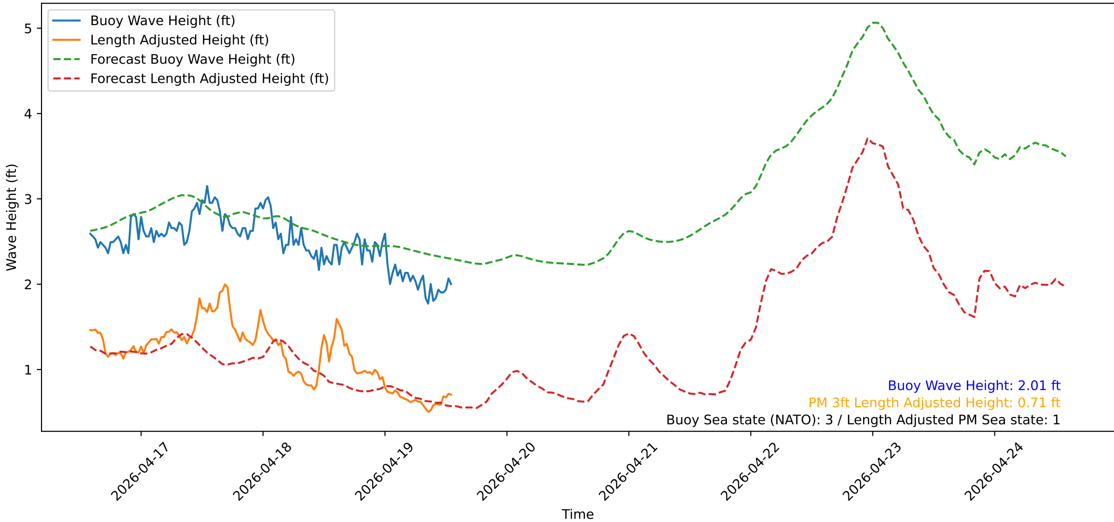
Wave Heights over Time for Red Beach at 2026-04-19 13:40:50
