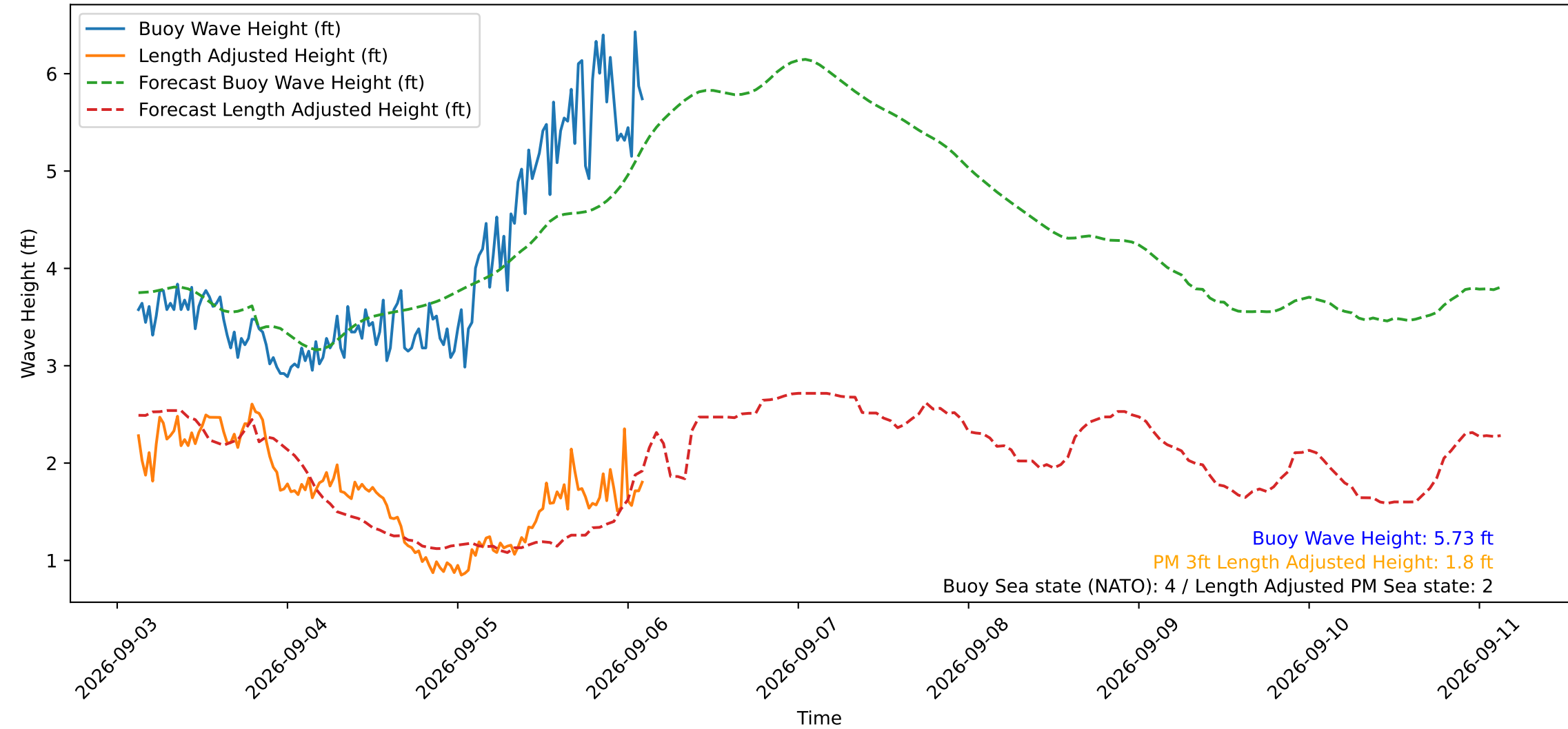
Wave Heights over Time for Oceanside Harbor at 2026-09-06 02:50:30
