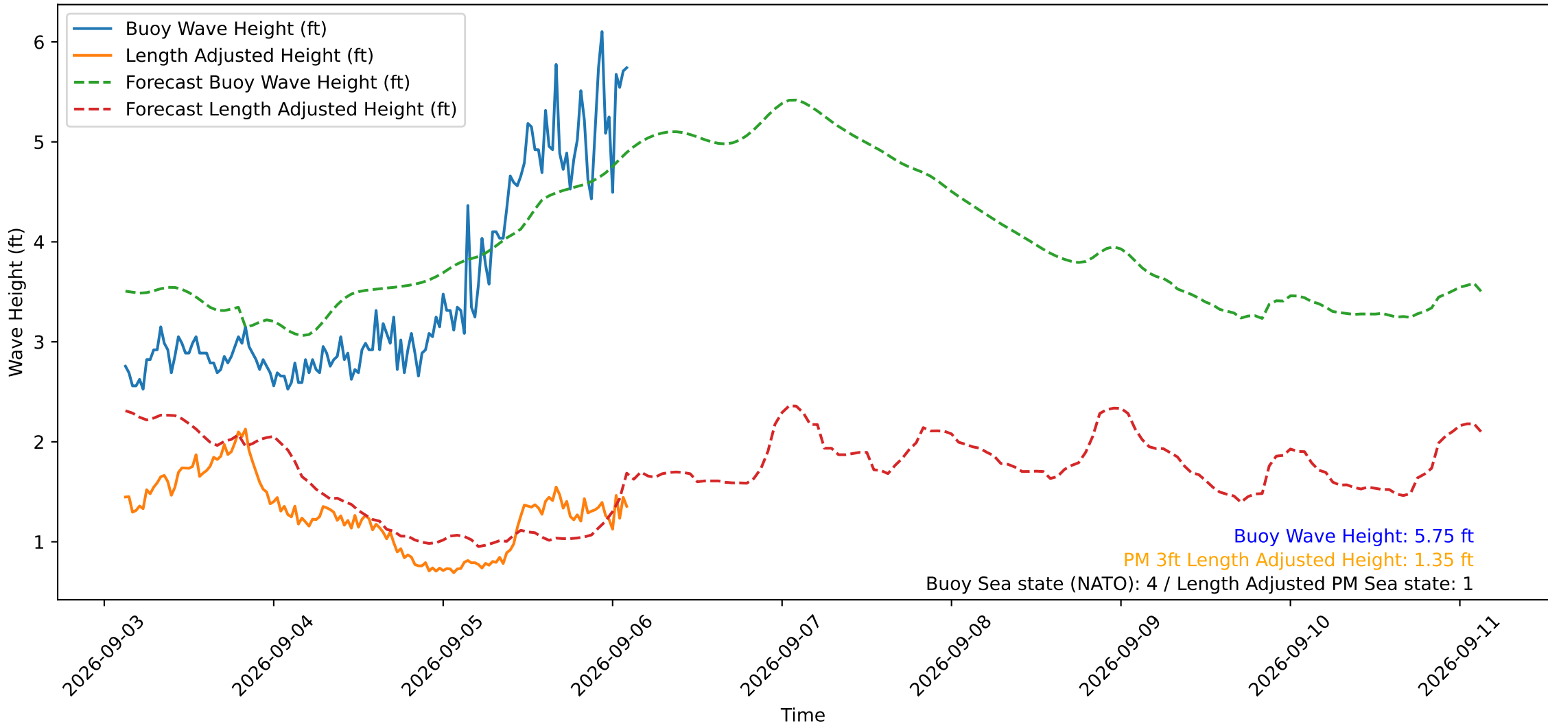
Wave Heights over Time for Red Beach at 2026-09-06 02:50:51
