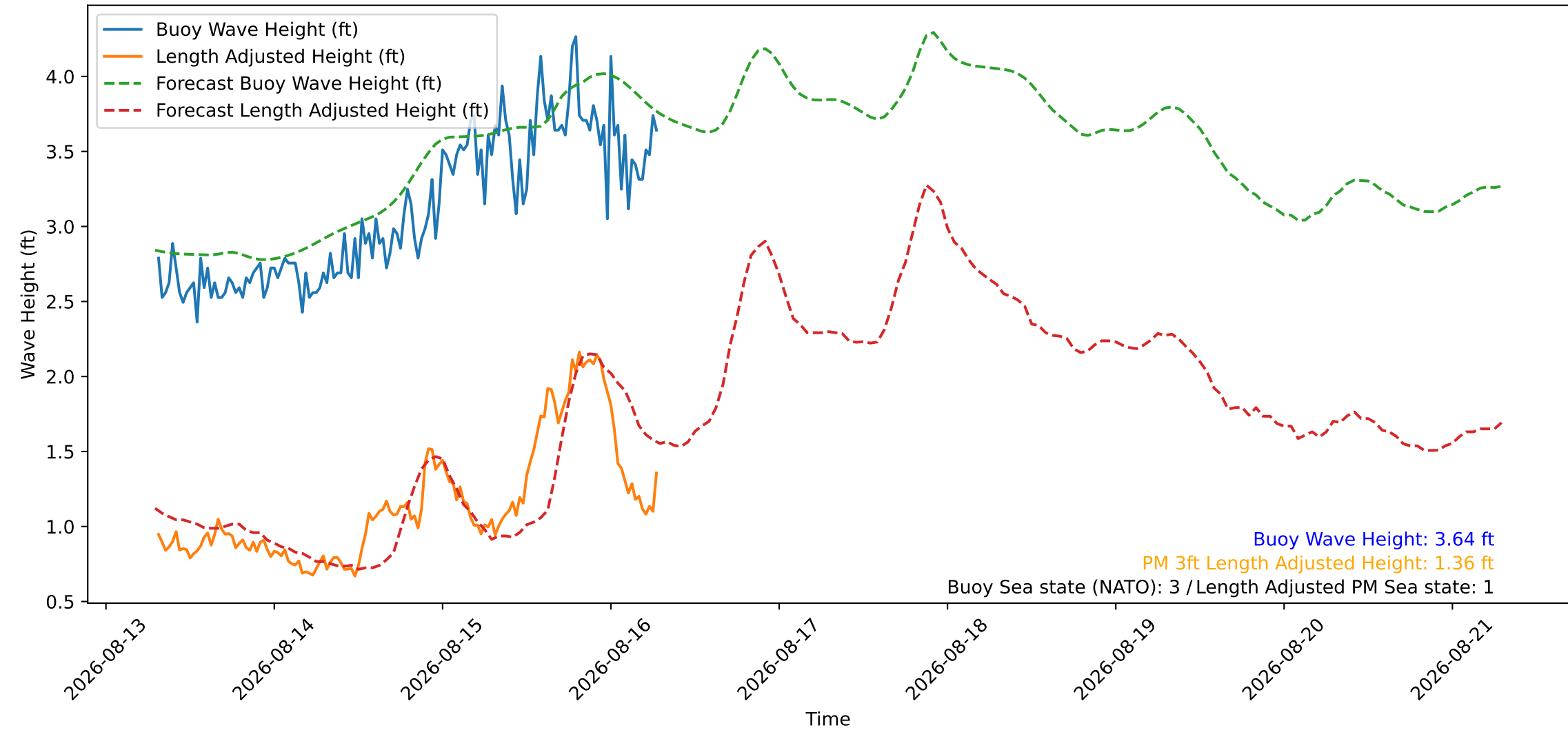
Wave Heights over Time for Green Beach at 2026-08-16 07:21:11
