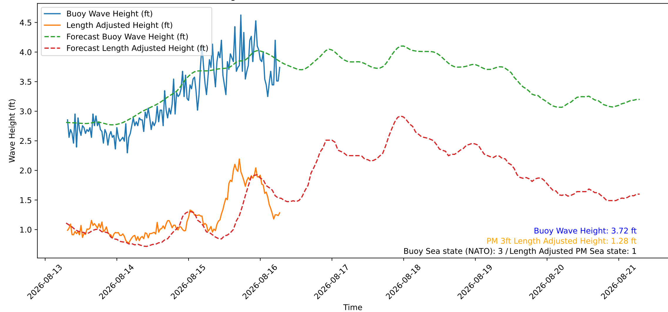
Wave Heights over Time for Oceanside Harbor at 2026-08-16 07:20:26
