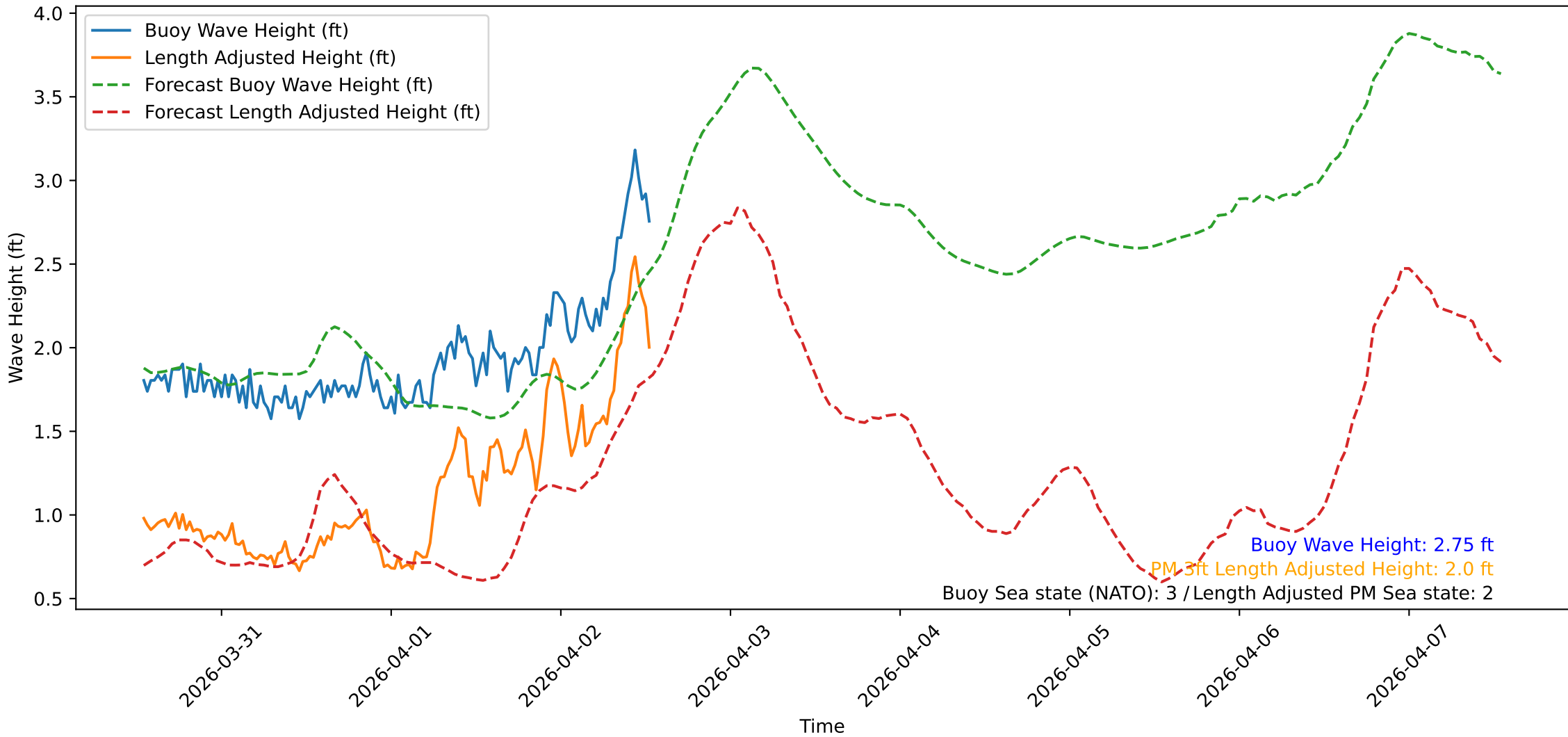
Wave Heights over Time for Oceanside Harbor at 2026-04-02 13:10:31
