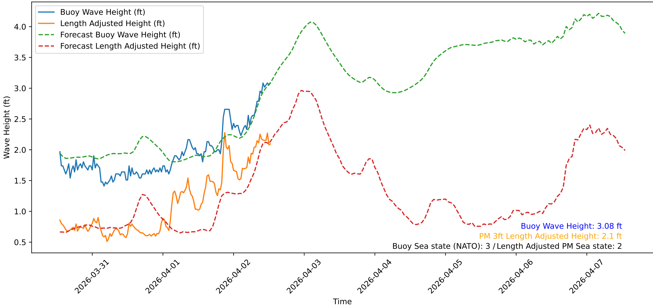
Wave Heights over Time for Green Beach at 2026-04-02 13:11:10
