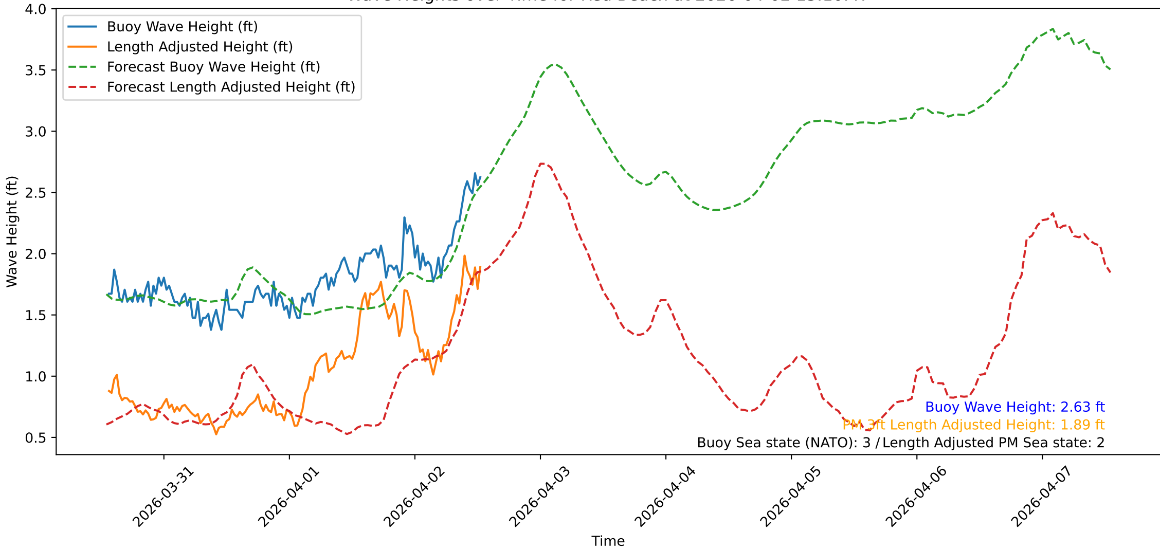
Wave Heights over Time for Red Beach at 2026-04-02 13:10:47
