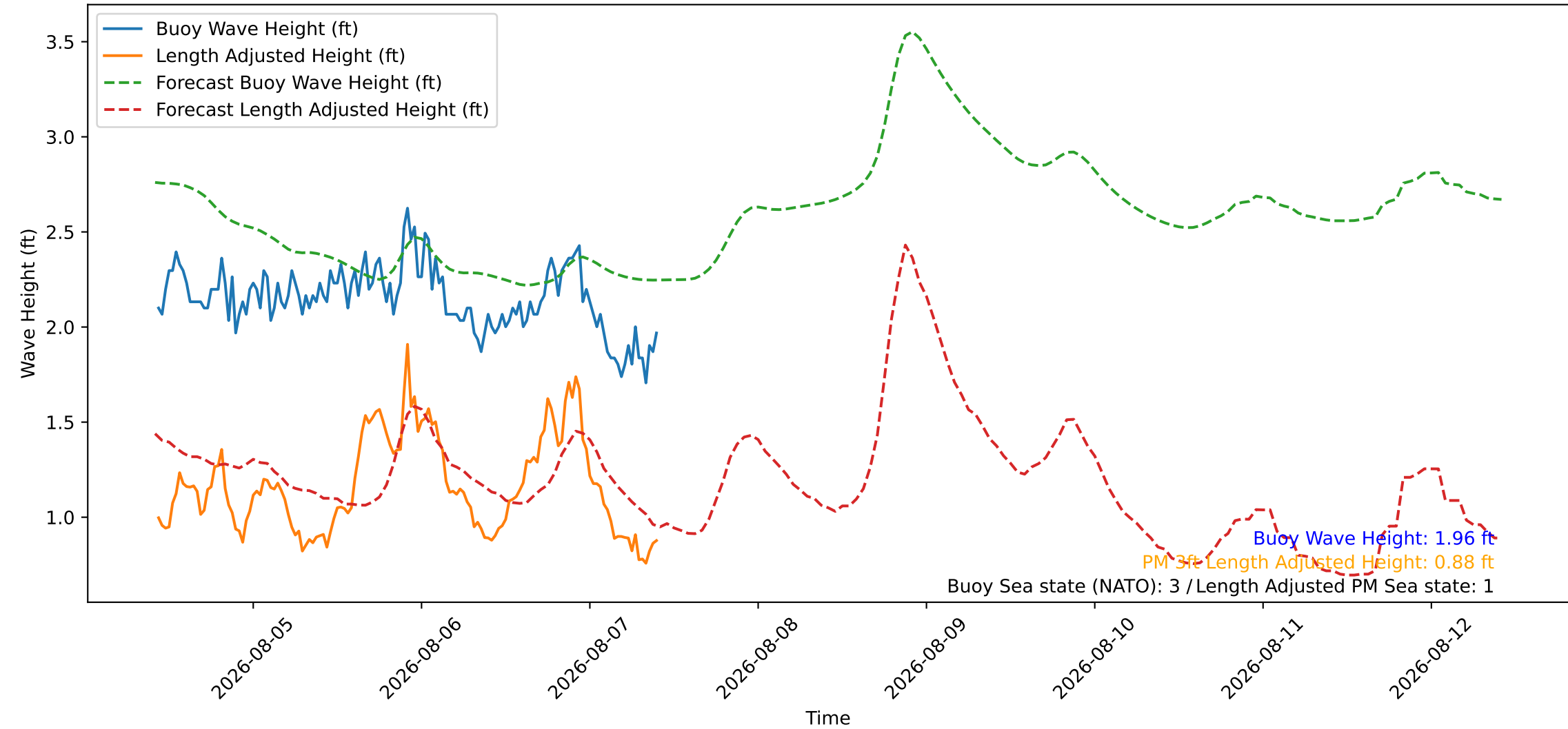
Wave Heights over Time for Green Beach at 2026-08-07 10:21:08
