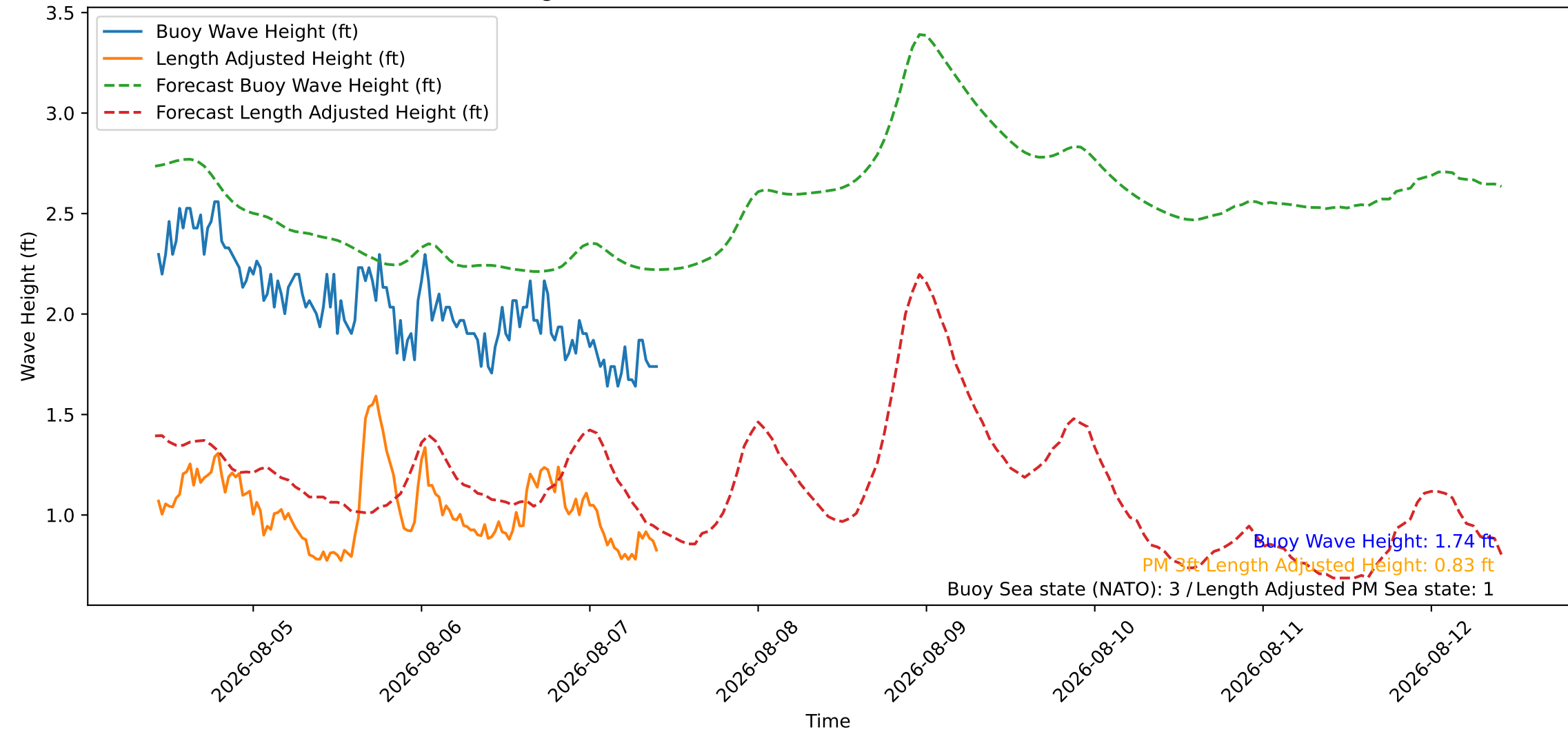
Wave Heights over Time for Oceanside Harbor at 2026-08-07 10:20:25
