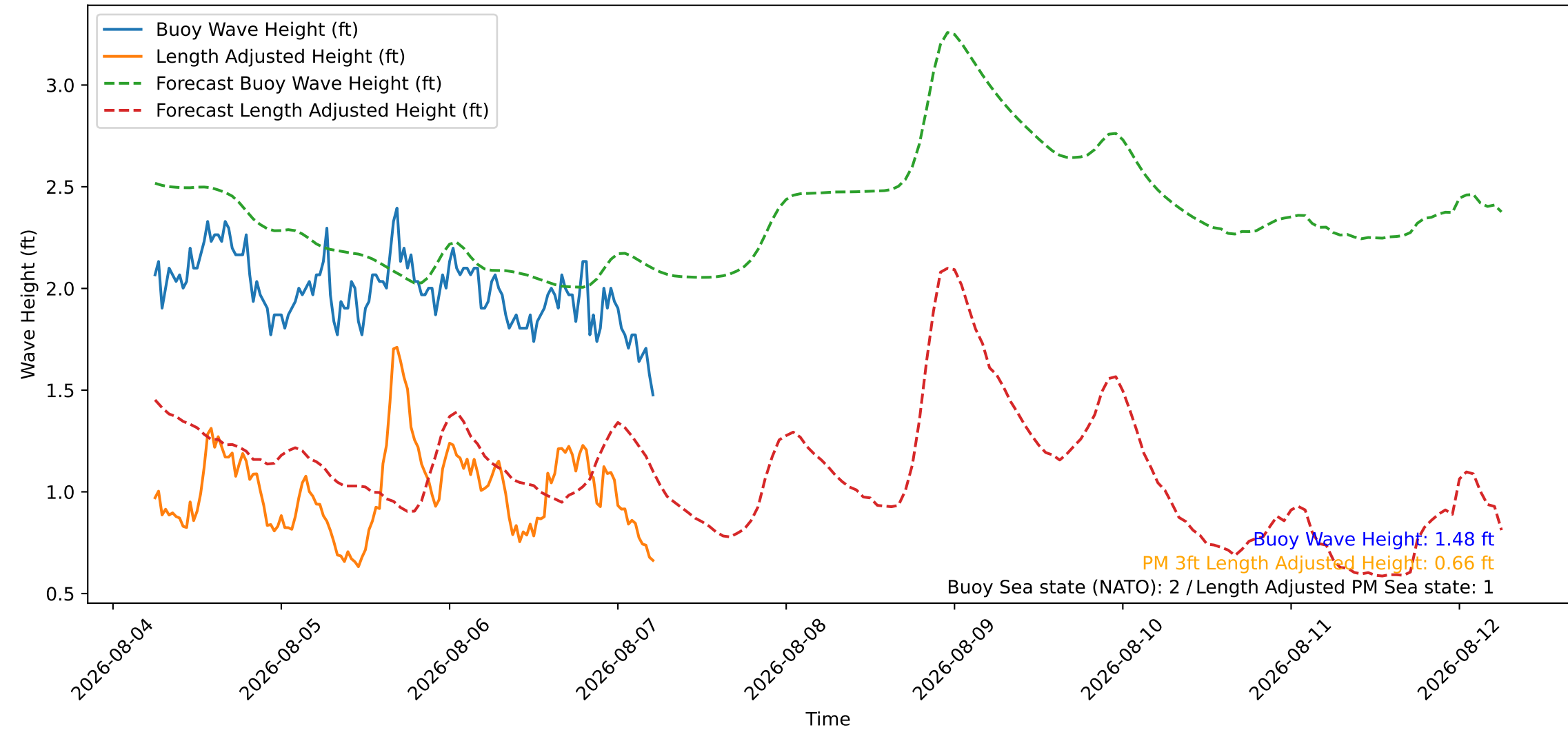
Wave Heights over Time for Red Beach at 2026-08-07 05:40:45
