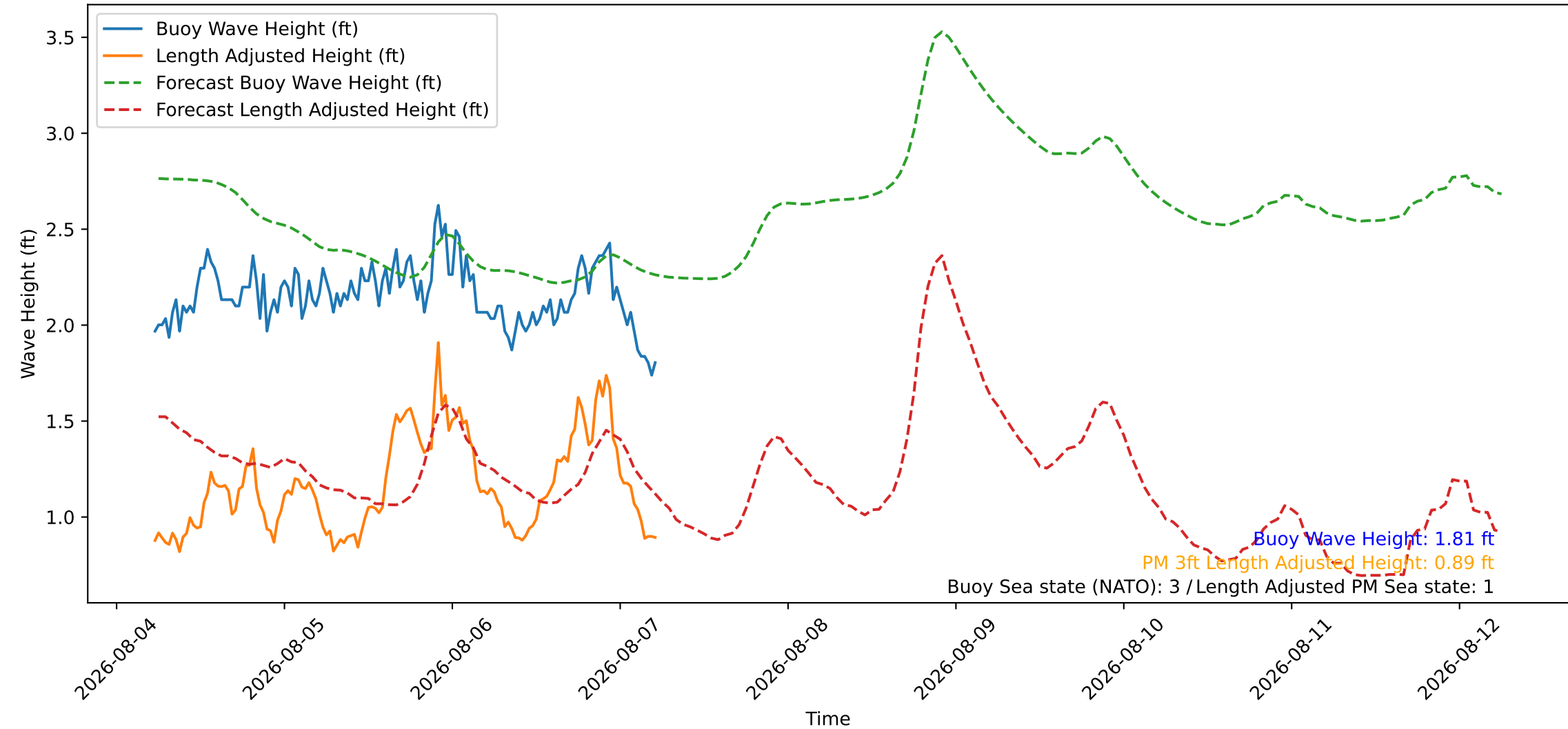
Wave Heights over Time for Green Beach at 2026-08-07 05:41:08
