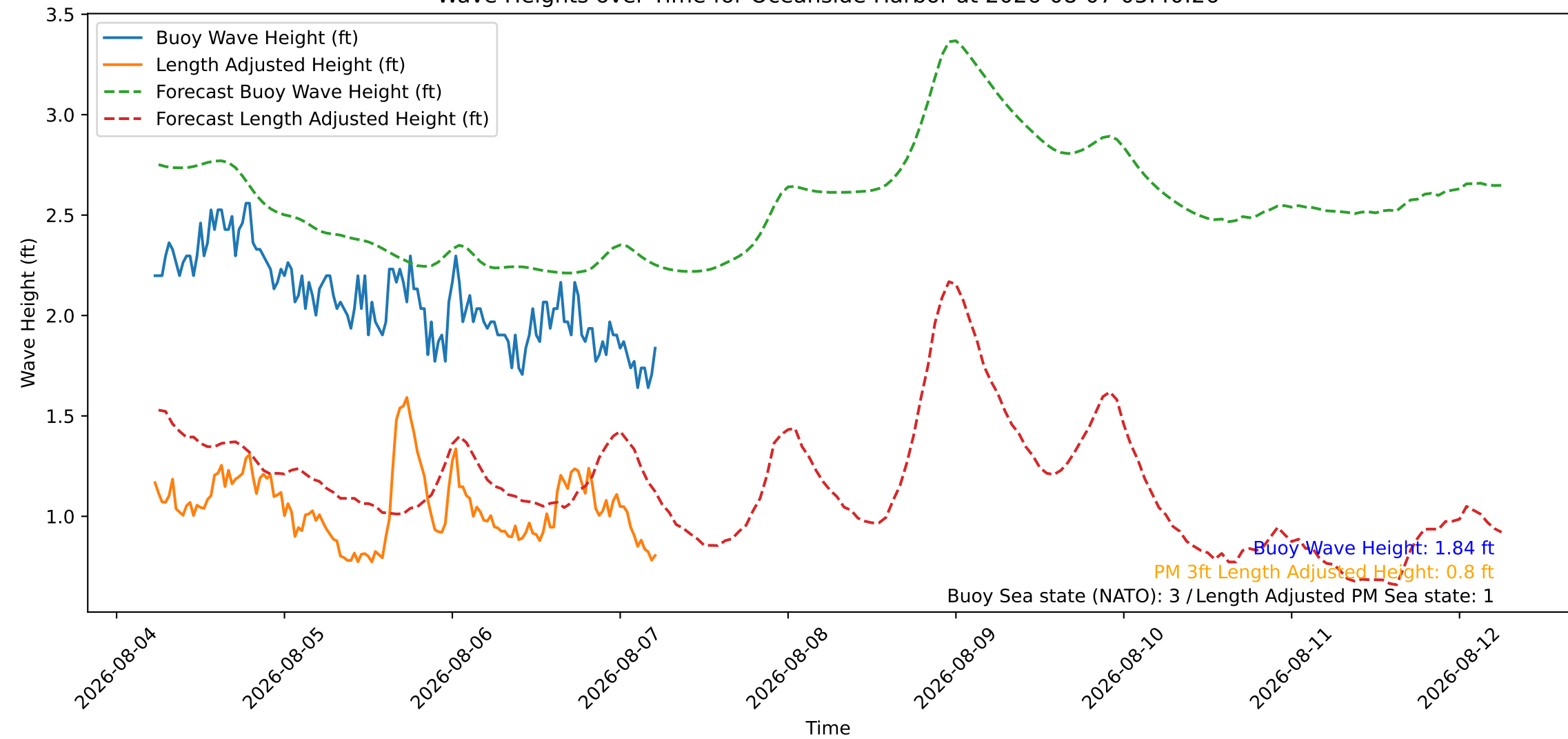
Wave Heights over Time for Oceanside Harbor at 2026-08-07 05:40:26
