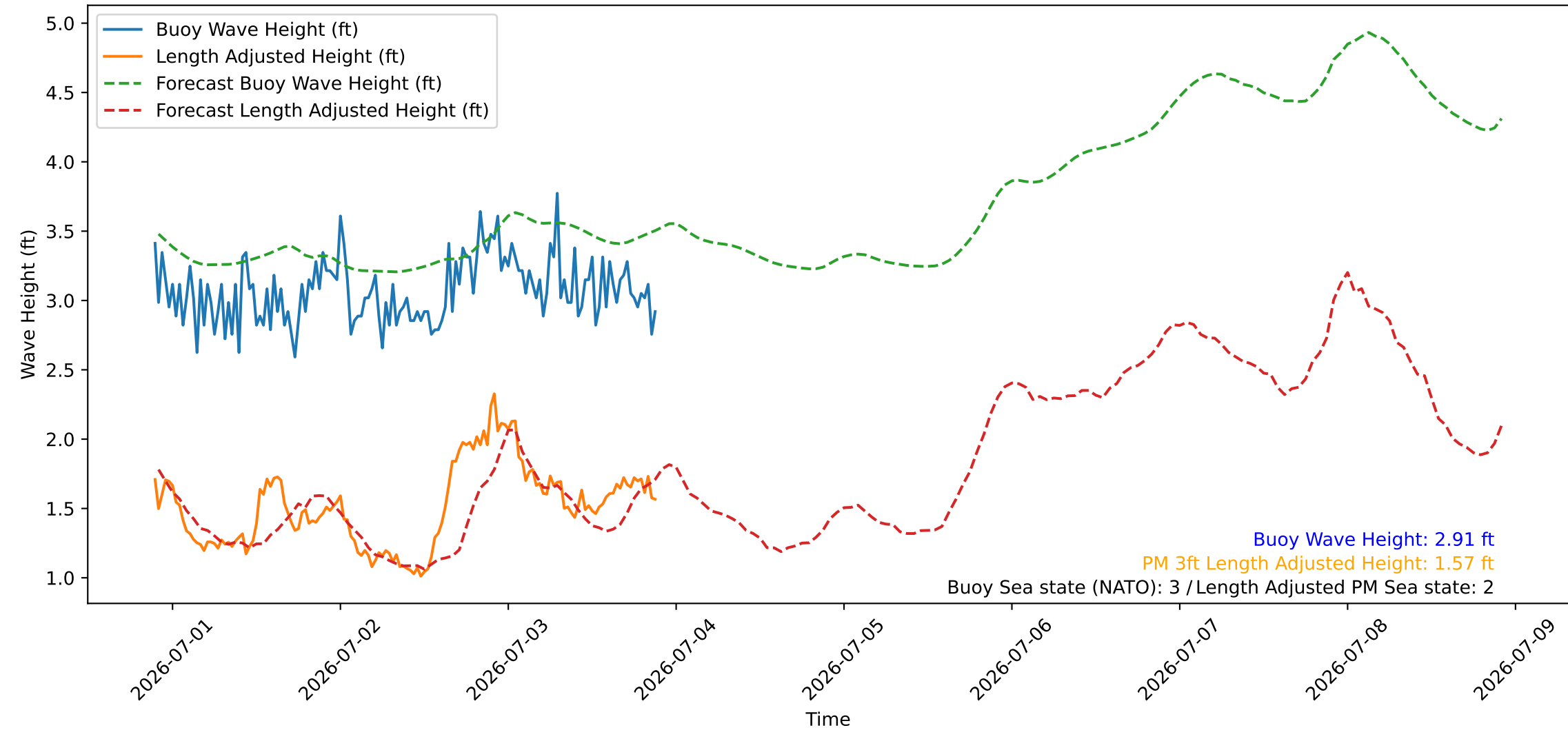
Wave Heights over Time for Oceanside Harbor at 2026-07-03 21:30:26
