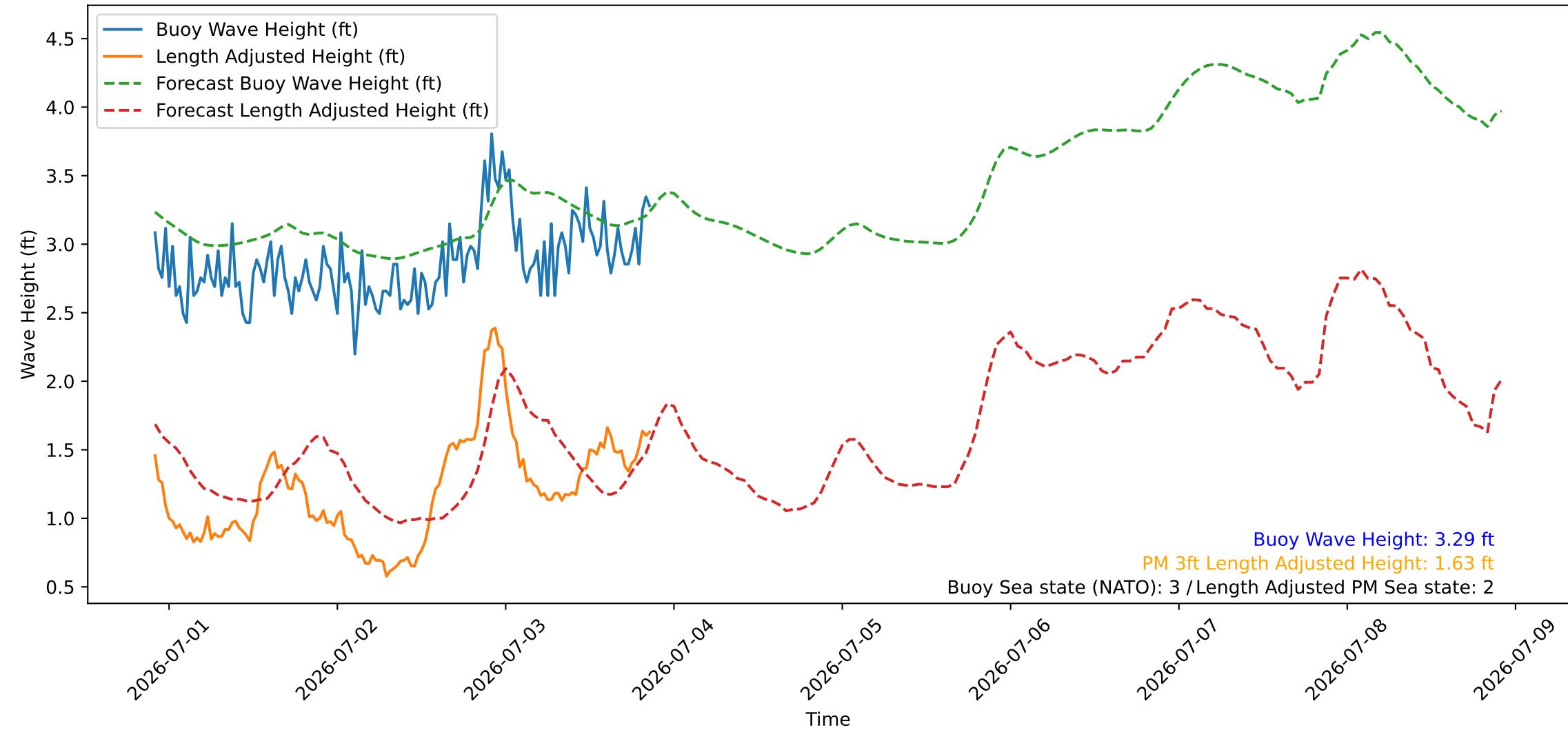
Wave Heights over Time for Red Beach at 2026-07-03 21:30:46
