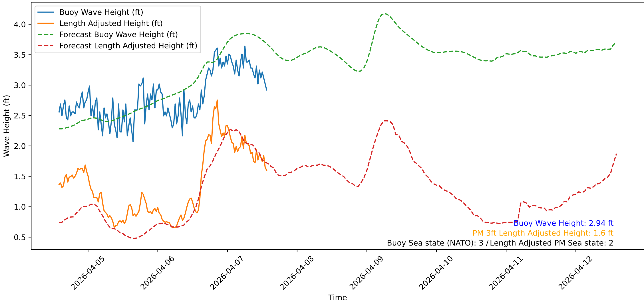
Wave Heights over Time for Oceanside Harbor at 2026-04-07 14:00:31
