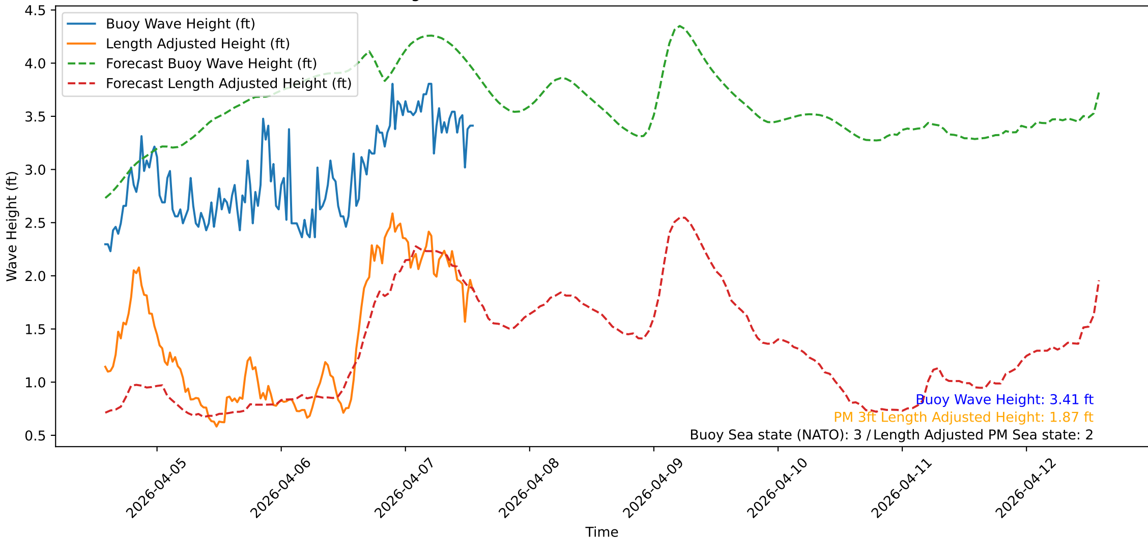
Wave Heights over Time for Green Beach at 2026-04-07 14:01:09
