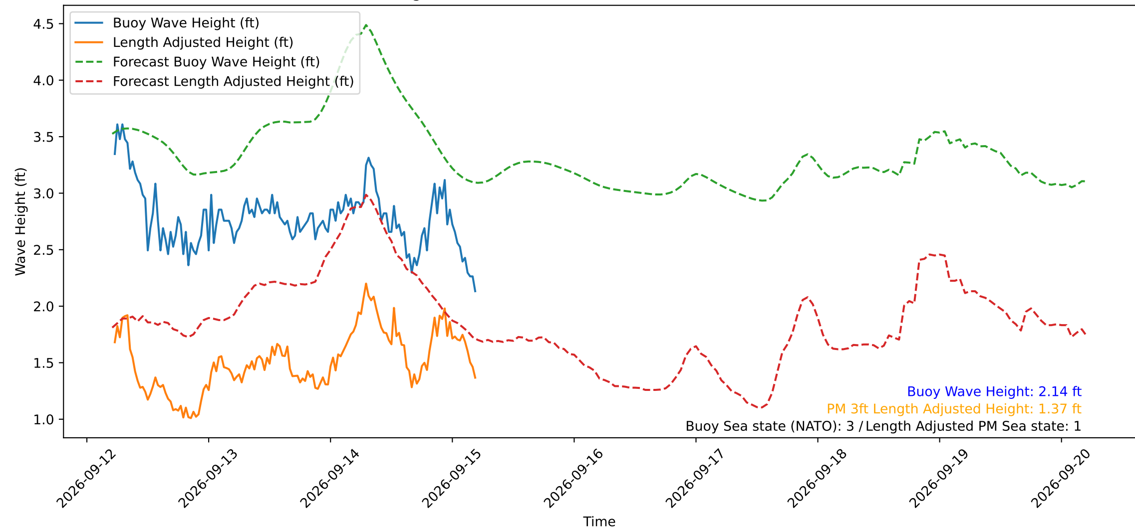
Wave Heights over Time for Green Beach at 2026-09-15 05:21:14
