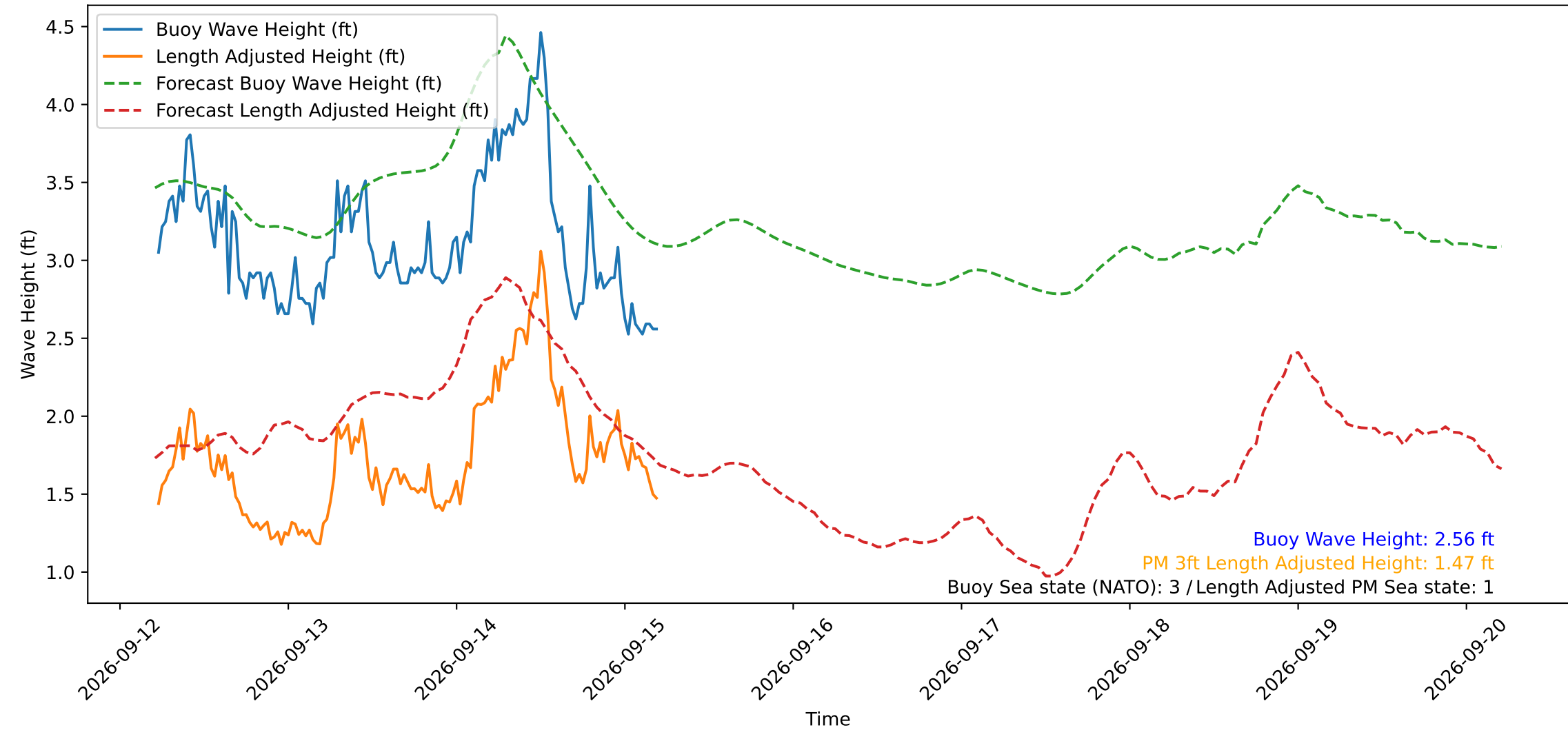
Wave Heights over Time for Oceanside Harbor at 2026-09-15 05:20:29
