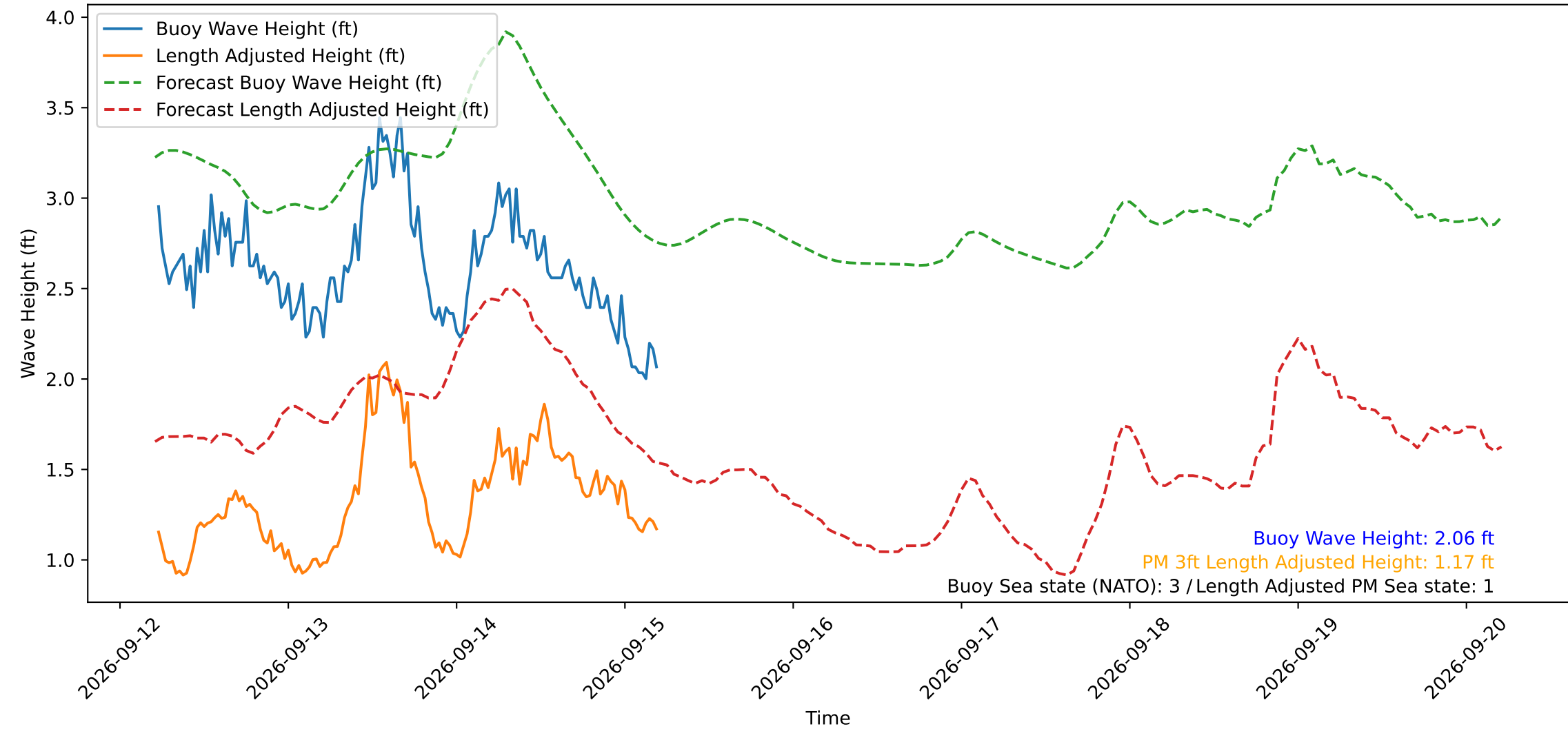
Wave Heights over Time for Red Beach at 2026-09-15 05:20:50
