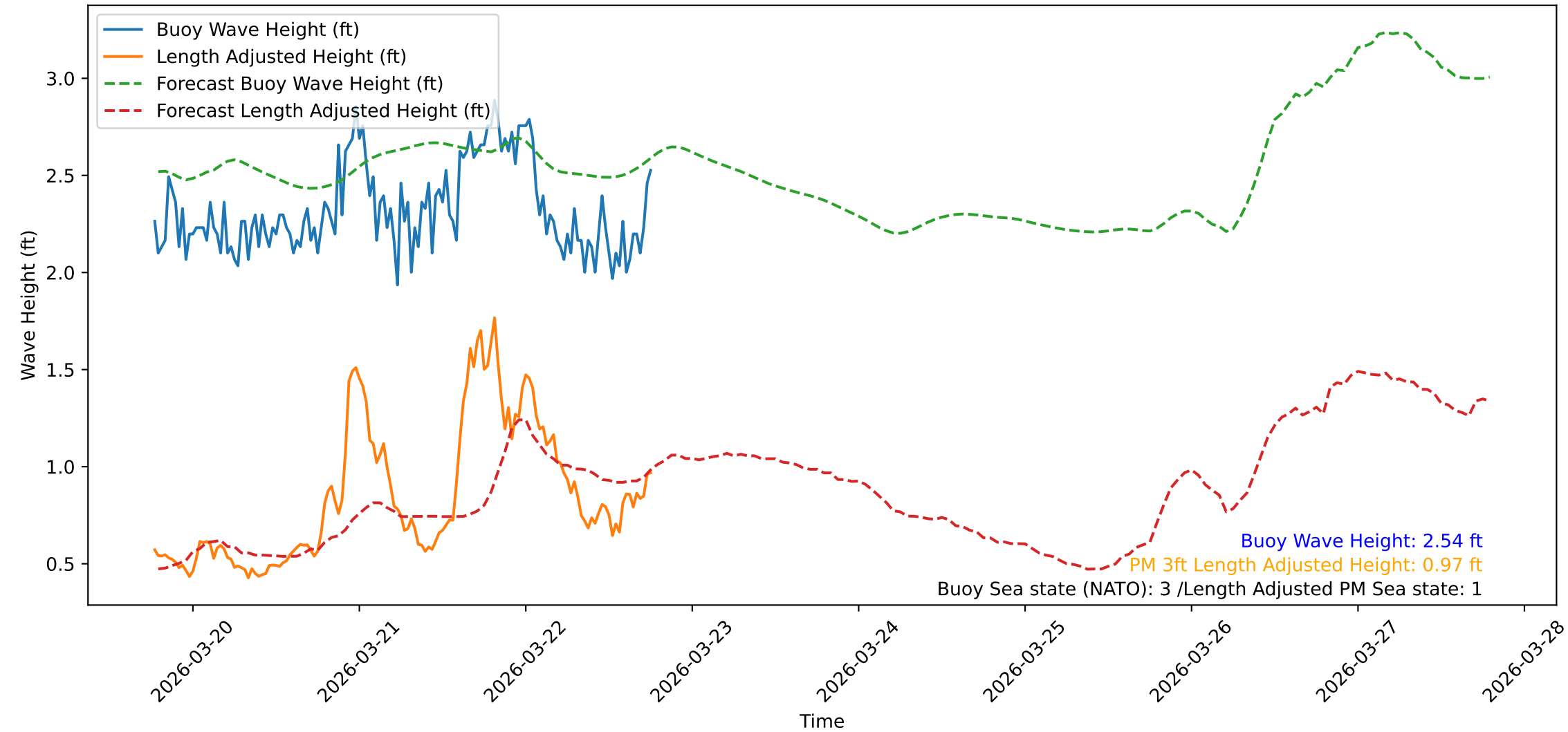
Wave Heights over Time for Green Beach at 2026-03-22 18:41:10
