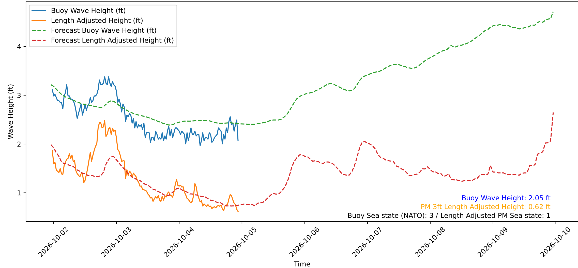
Wave Heights over Time for Green Beach at 2026-10-04 23:11:11
