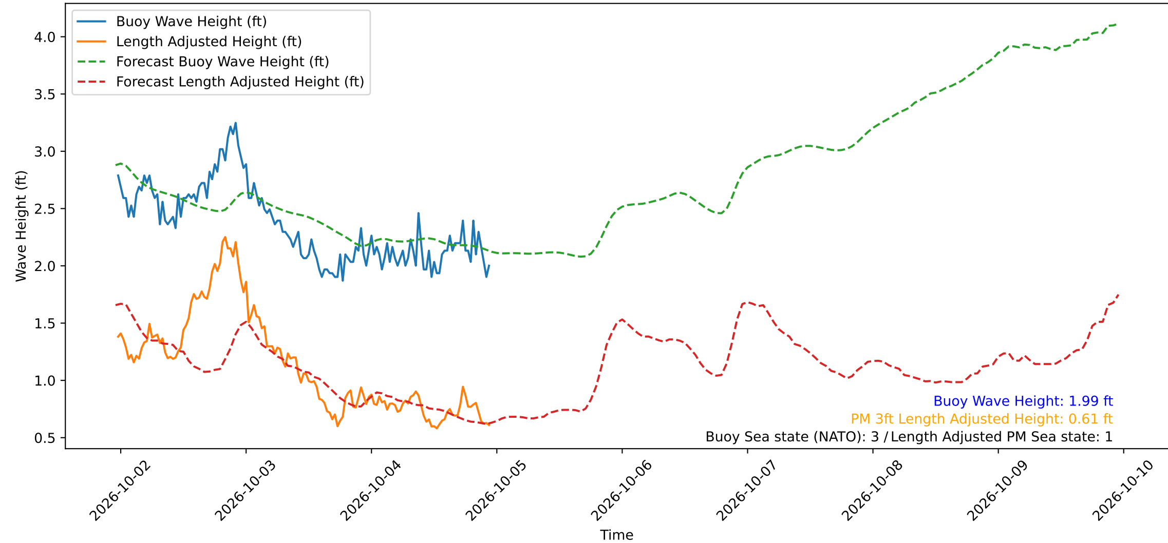
Wave Heights over Time for Red Beach at 2026-10-04 23:10:49
