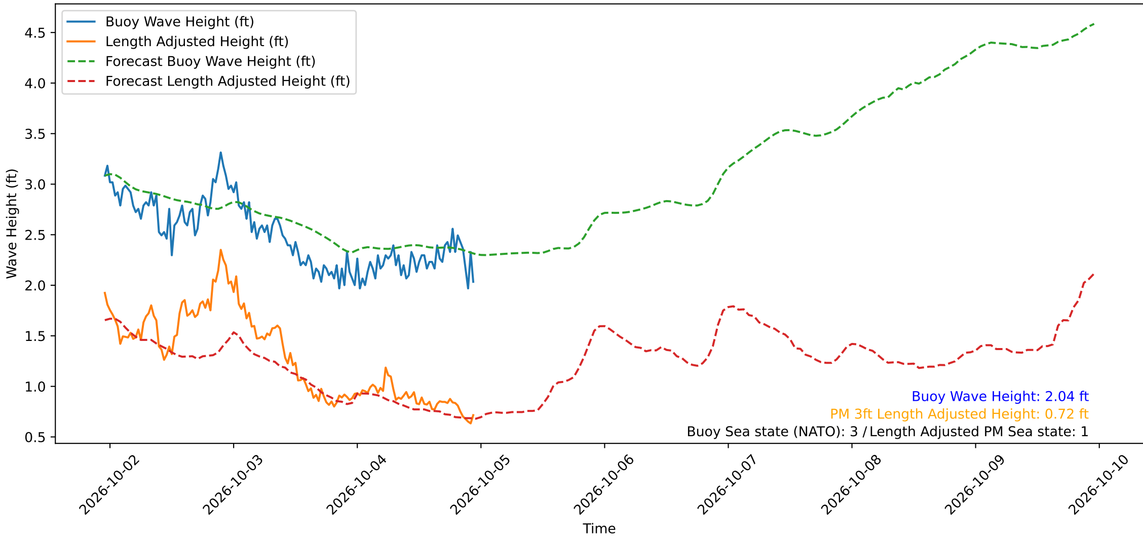
Wave Heights over Time for Oceanside Harbor at 2026-10-04 23:10:29
