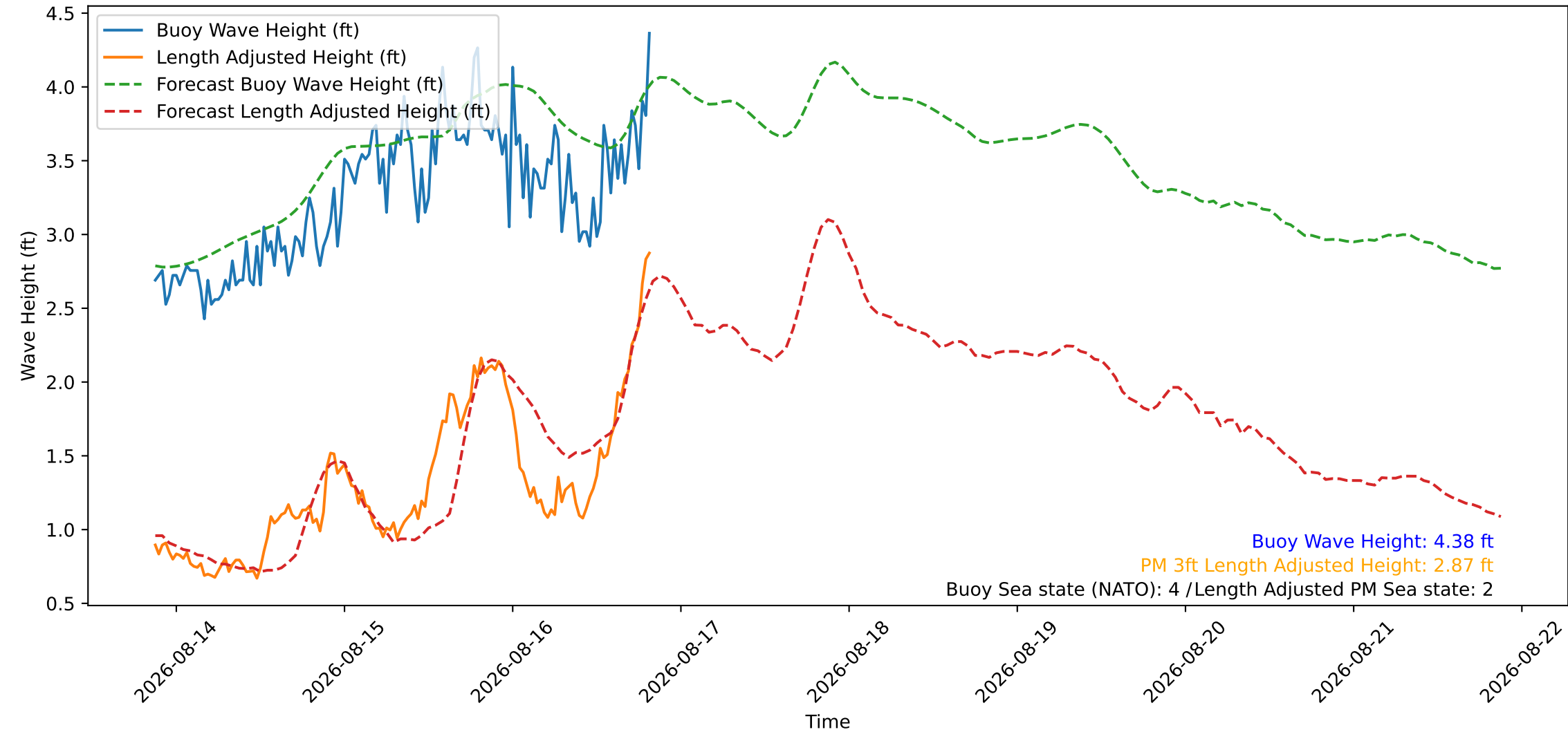
Wave Heights over Time for Green Beach at 2026-08-16 20:31:08
