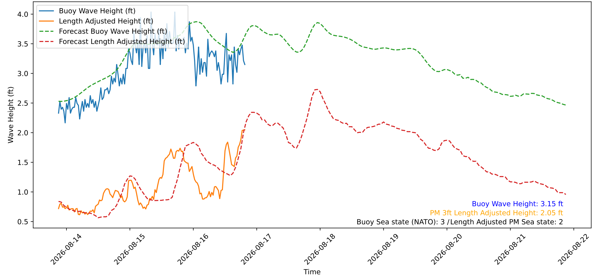
Wave Heights over Time for Red Beach at 2026-08-16 20:30:46
