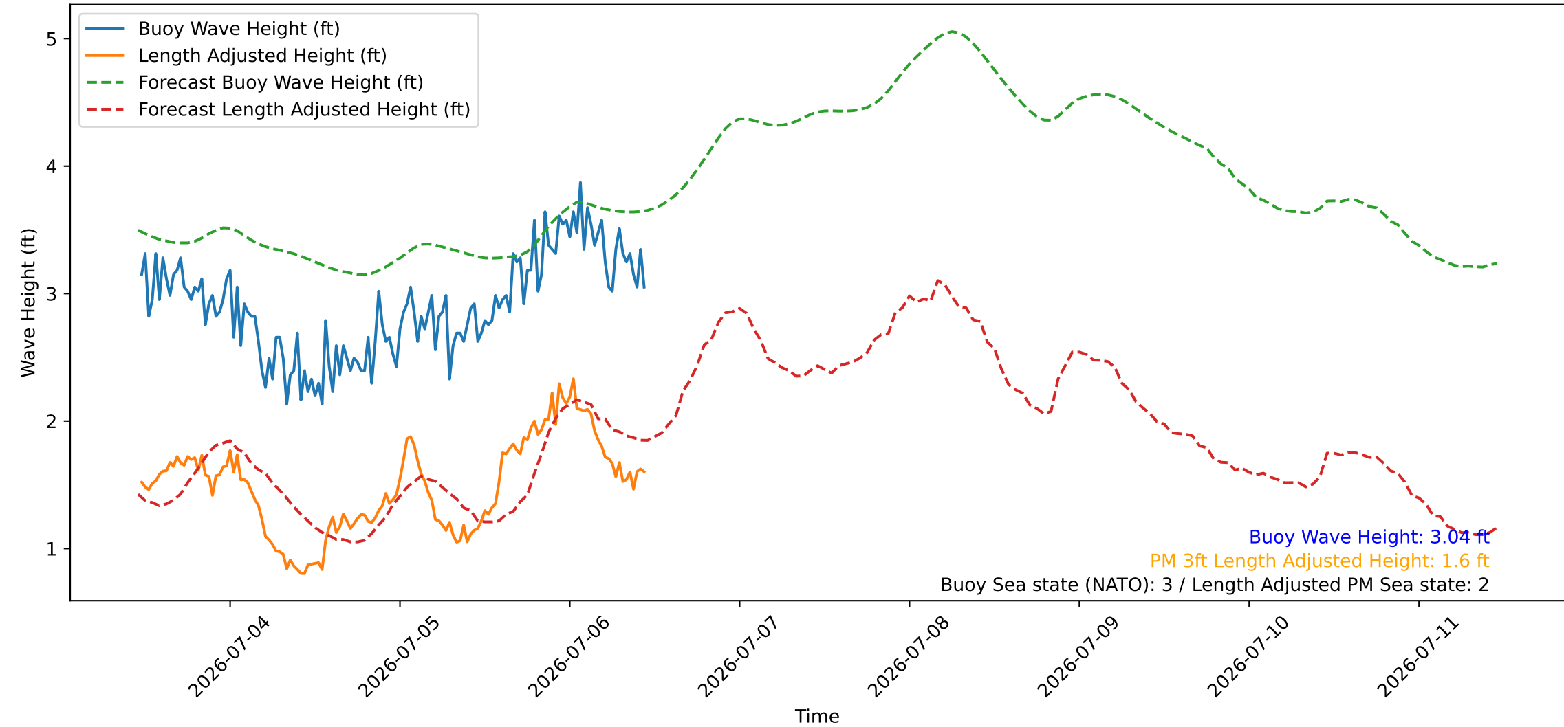
Wave Heights over Time for Oceanside Harbor at 2026-07-06 11:20:27
