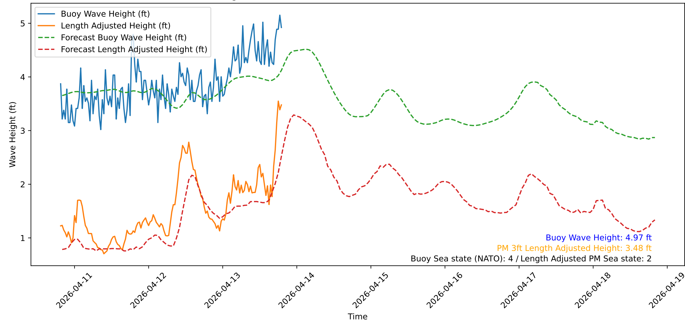
Wave Heights over Time for Oceanside Harbor at 2026-04-13 19:40:31
