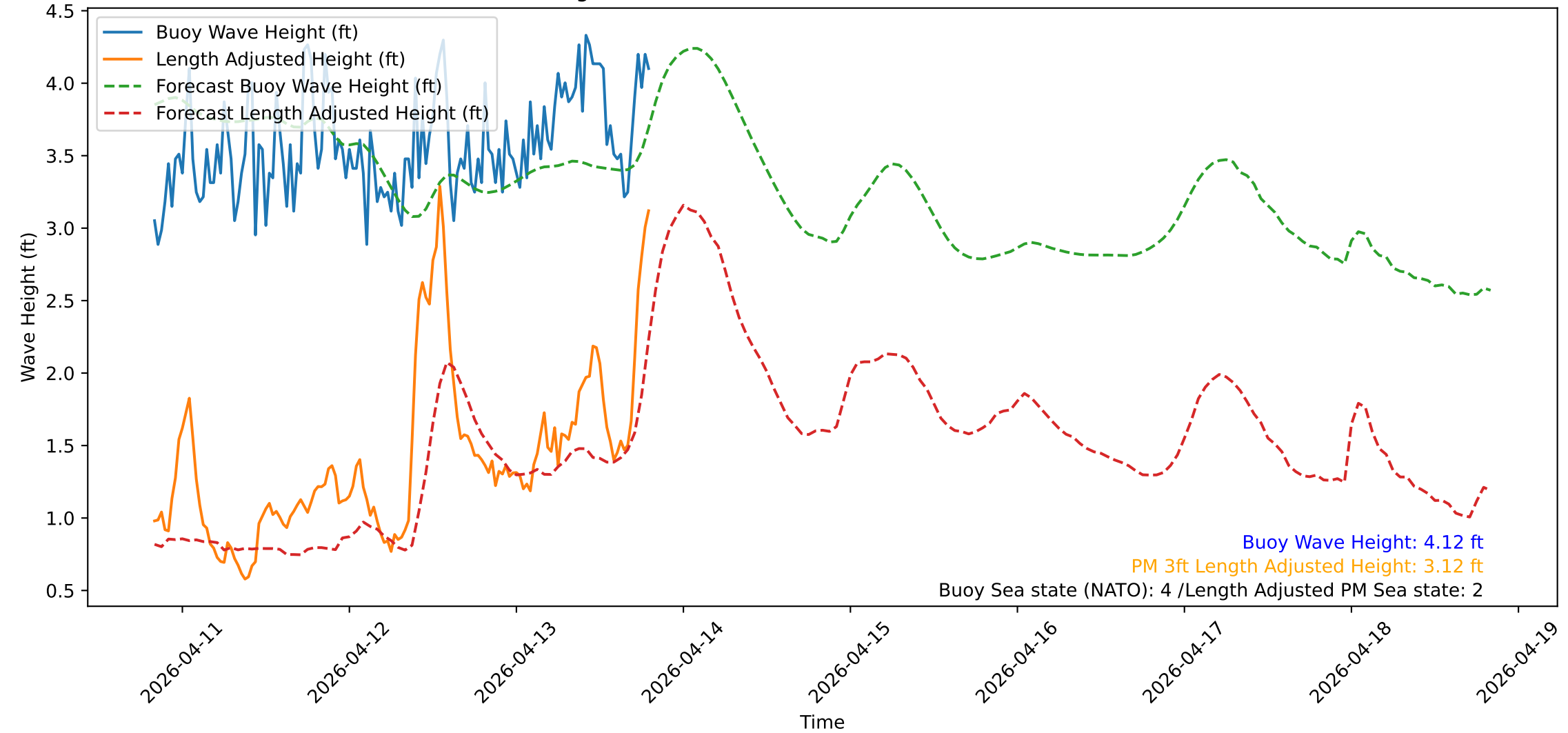
Wave Heights over Time for Red Beach at 2026-04-13 19:40:50
