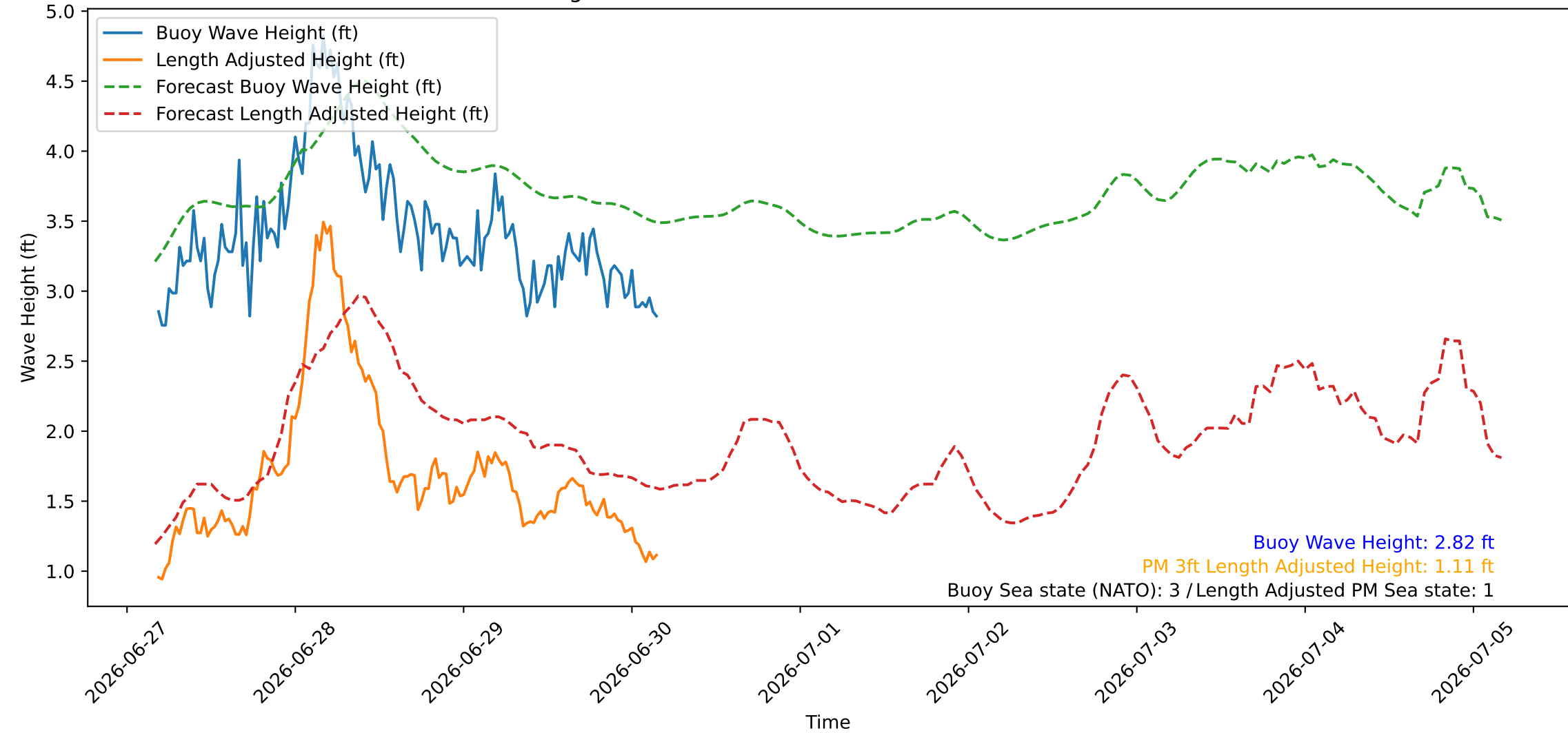
Wave Heights over Time for Green Beach at 2026-06-30 04:21:09
