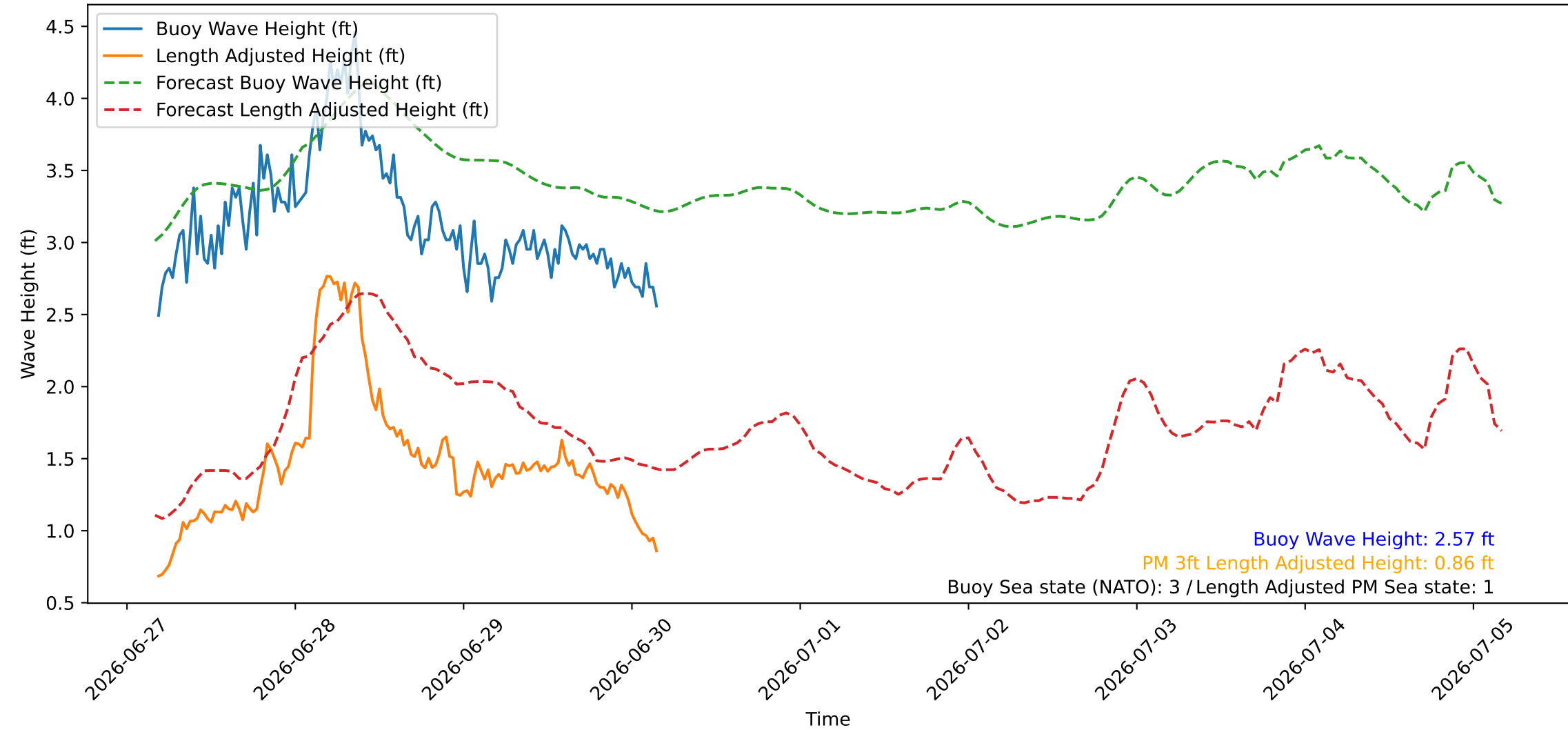
Wave Heights over Time for Red Beach at 2026-06-30 04:20:47
