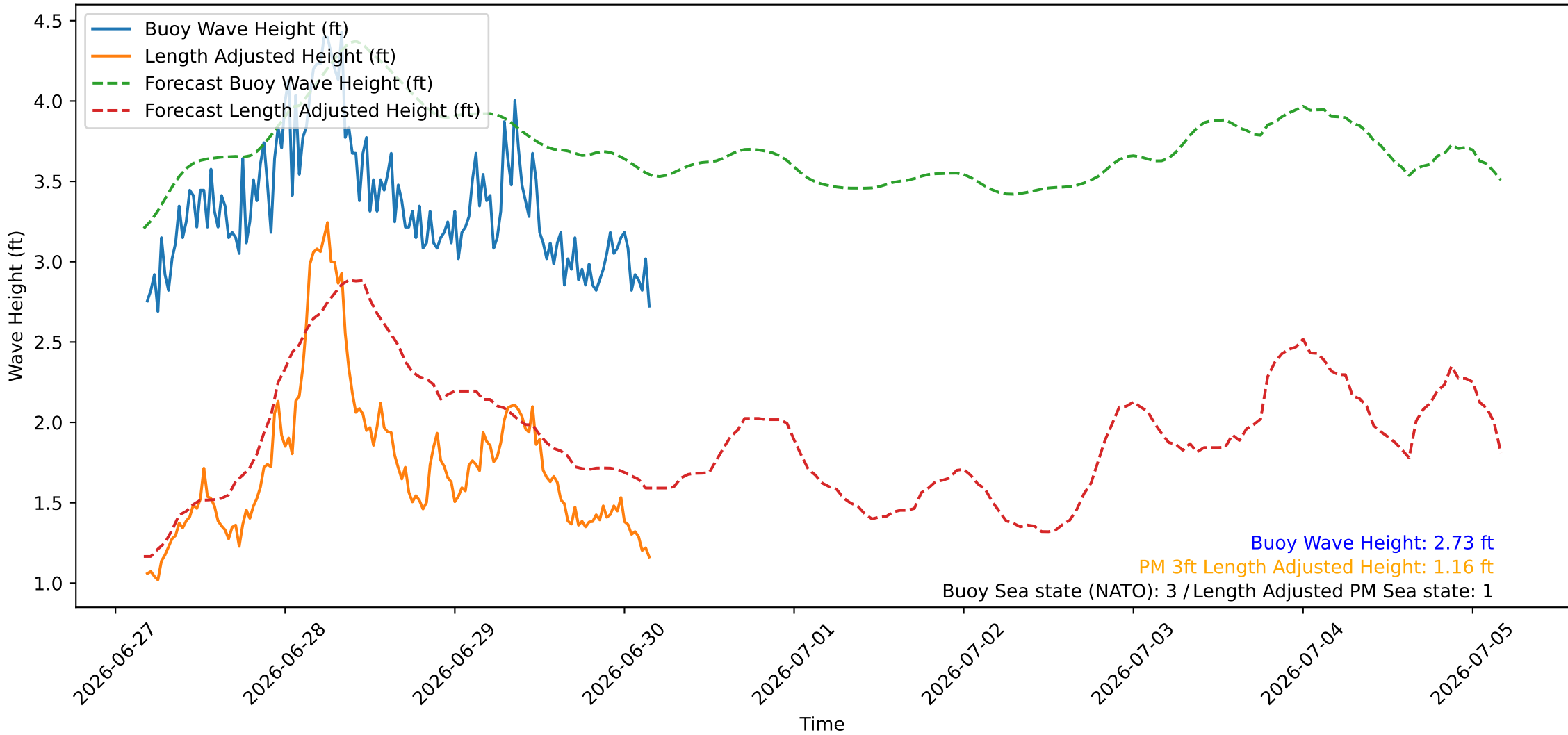
Wave Heights over Time for Oceanside Harbor at 2026-06-30 04:20:26
