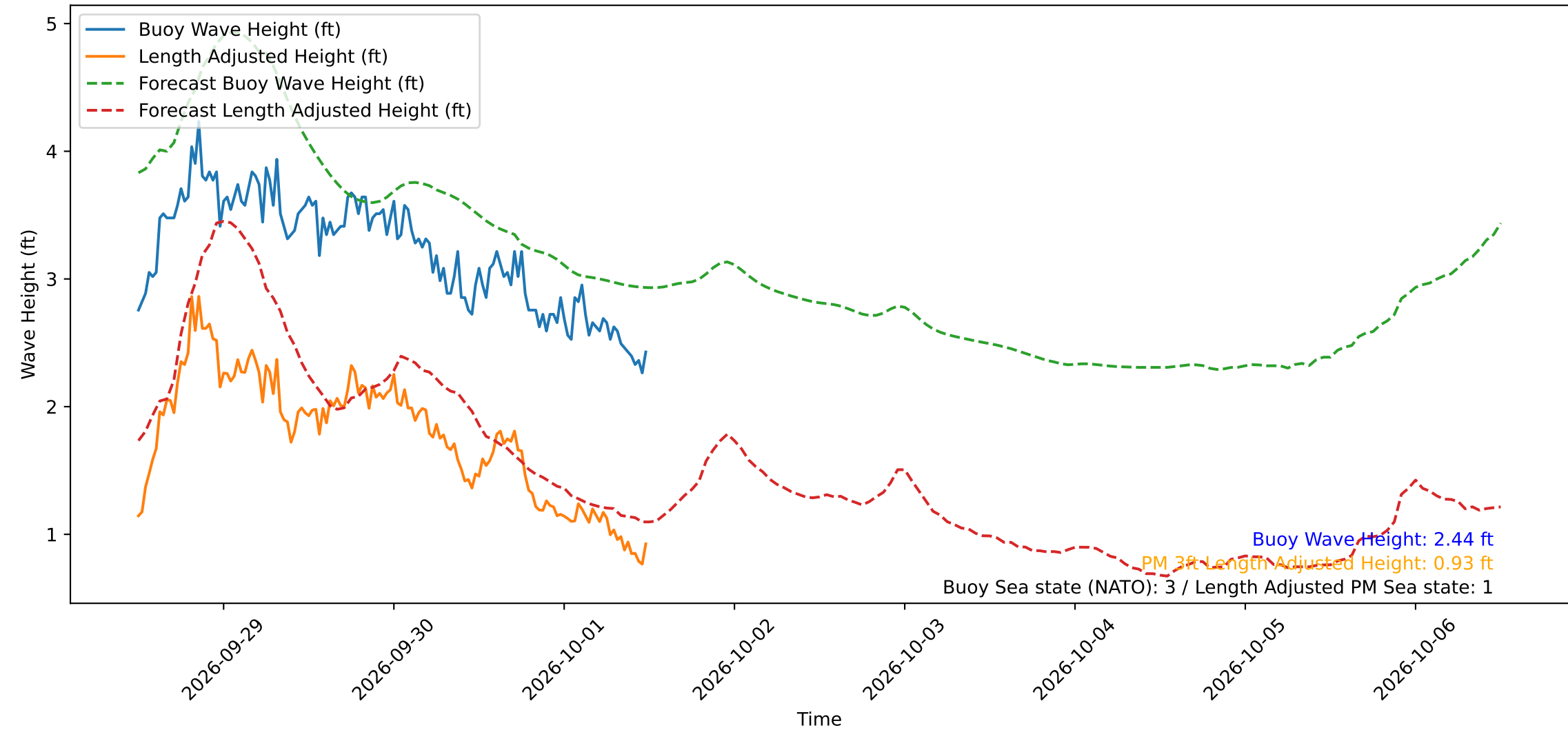
Wave Heights over Time for Oceanside Harbor at 2026-10-01 12:10:30
