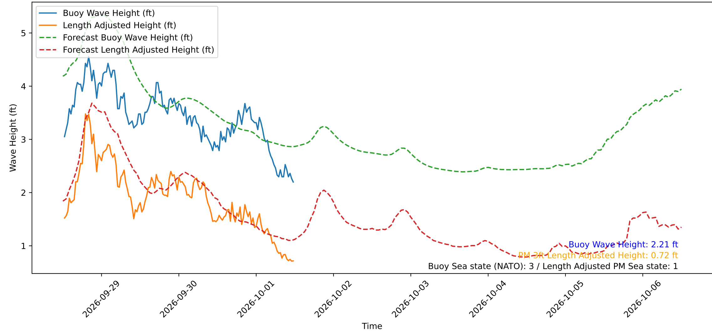
Wave Heights over Time for Green Beach at 2026-10-01 12:11:12
