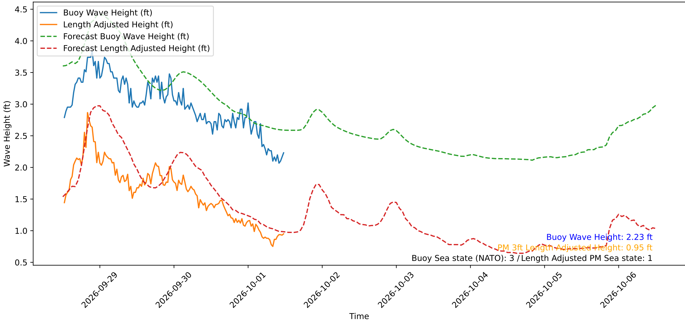
Wave Heights over Time for Red Beach at 2026-10-01 12:10:50
